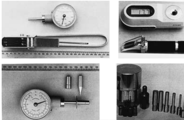
Figure 12.85 Texture measuring equipment, also with refractometers at the top right. Source: Dr James Ssemwanga.
