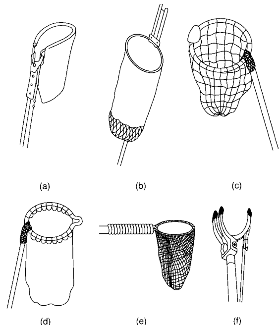
Figure 3.2 Bags and other fitments used on picking poles which are used as a harvesting aid for fruit on tall trees. (a) Pole with clippers attached, from Thailand. (b) For harvesting papaya in Thailand. (c) Hand-woven bag with cutting edge opposite the pole attachment. (d) Canvas bag with cutting notch. (e) Mango harvester from the Philippines. (f) Apple harvester from the UK. Sources: Bautista (1990), Kitmoja and Kader (1993).
