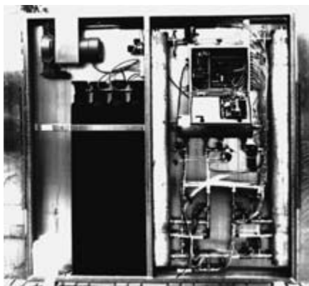
Figure 11.6 Controlled atmosphere reefer container controls. Source: Tim Bach of Cronos.
