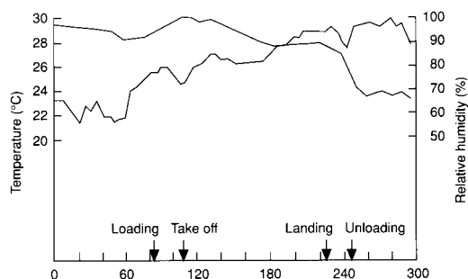
Figure 11.9 Temperature and humidity of okras ( Hibiscus esculentus ) during airfreight transport. Source: Akinaga and Kohda (1993).
