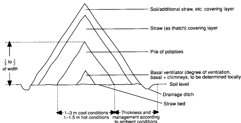
Figure 7.4 Details of the construction of a potato clamp. Source: CIP (1981).
