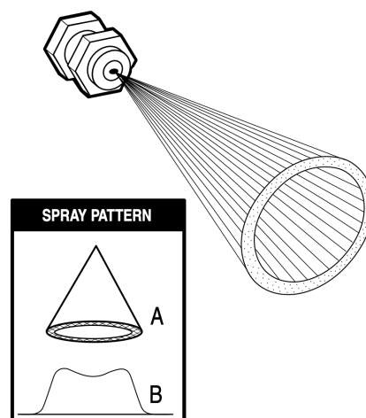
Figure 11-7. Hollow cone nozzle spray pattern (A) and spray distribution (B).
