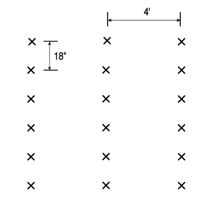
Figure 4-2. Spacing diagram for the matted row system.
