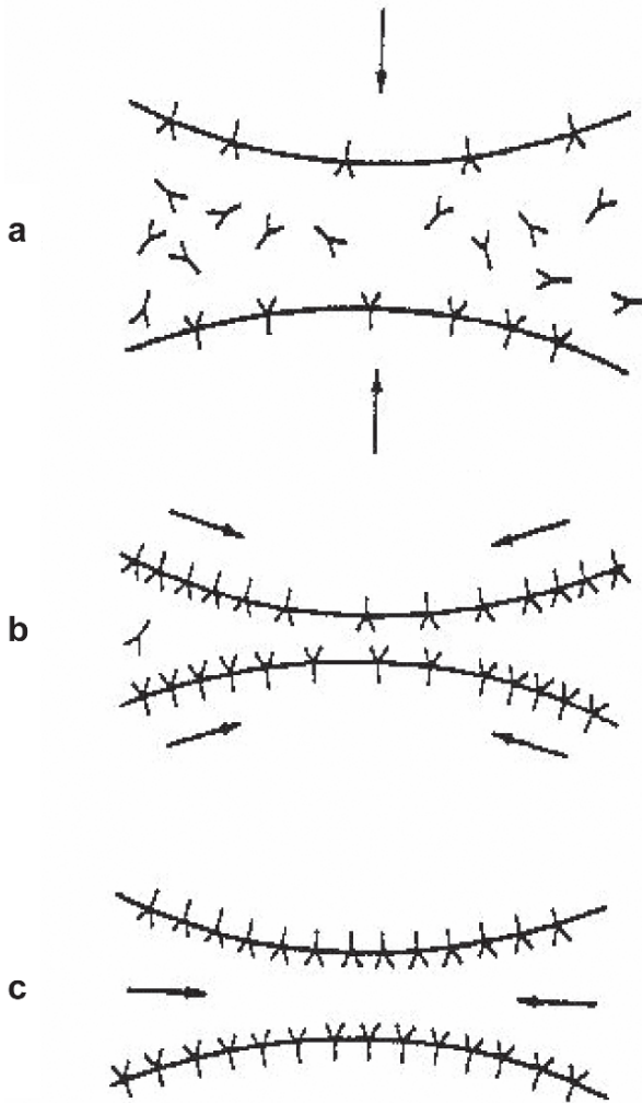
Fig. 13.18 Gibbs-Marangoni effect for two approaching droplets during emulsification. Surfactant molecules are depicted by Y (Király and Vincent 1992)
