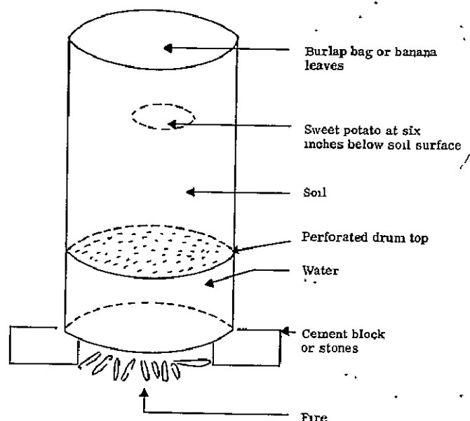
Figure 78. HOME MADE SOIL STERILIZER.
