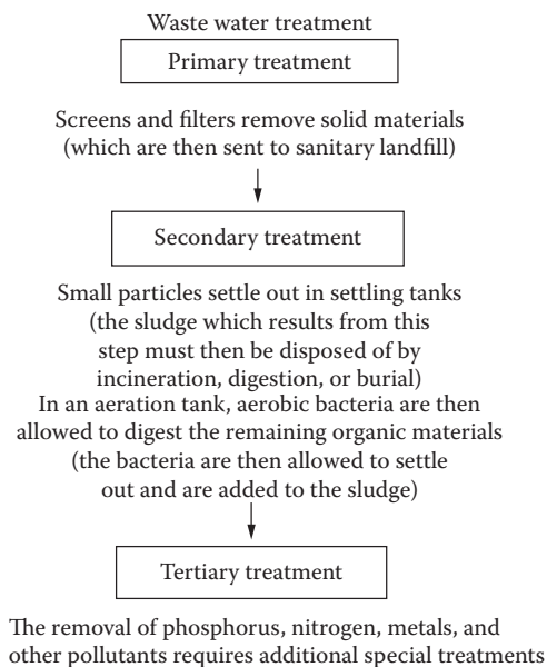
FIGURE 17.4 Wastewater treatment.
