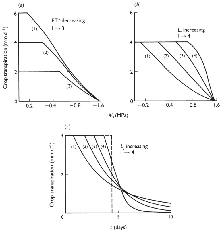
Fig. 9.6 Simulated crop transpiration ( E_p ) in response to soil water potential for (a) three levels of ET^* = 6, 4 , and 2 \text{ mm d}^{-1} ; (b) four levels of root-length density ( L_v = 0.12, 0.25, 0.5 \text{ cm}^{-2} and very dense); and (c) the decrease in E_p with time from an initially wet soil is shown for four levels of L_v ( 0.12, 0.25, 0.5 \text{ cm}^{-2} , and very dense). (After Cowan 1965.)
