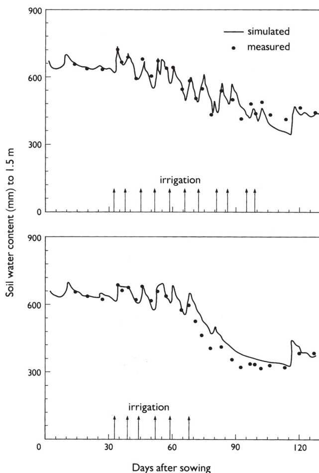
Fig. 9.9 Measured and simulated soil water content under sunflower crops with different irrigation regimes at Tatura, Australia (Connor, unpublished).
