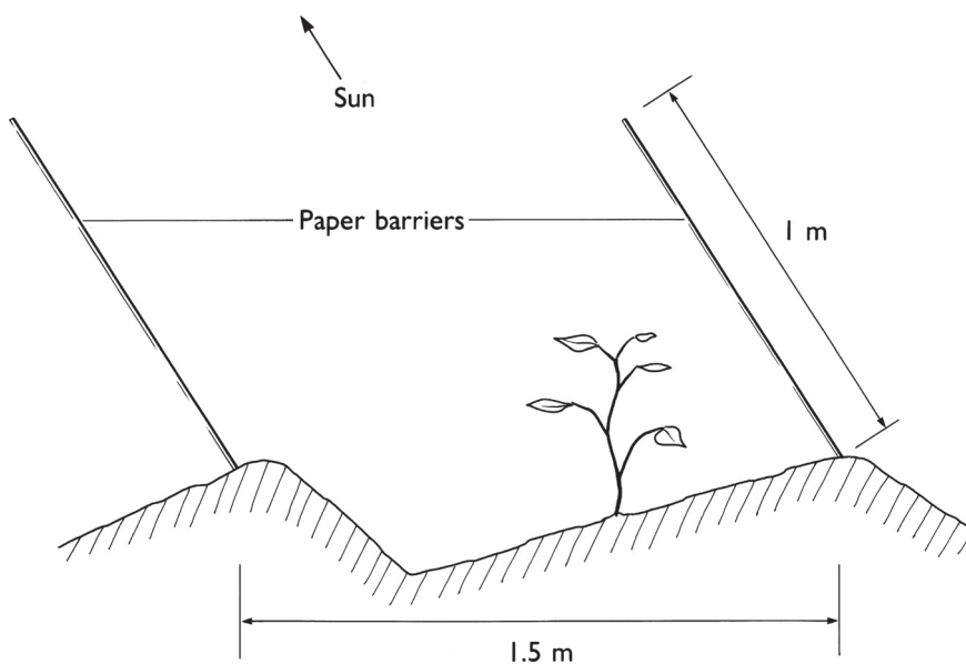
Fig. 12.6 Sloped seedbed with protective paper shelters used for forcing vegetable production in a cool climate. The arrangement creates non-uniform soil temperatures (cold behind the barrier, warm towards the sun) while protecting plants from wind and, at night, from radiation frost.
