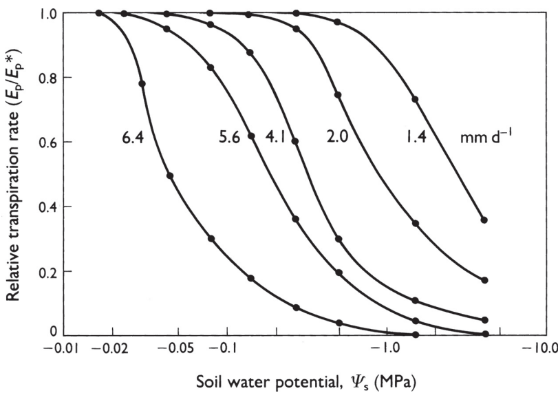
Fig. 9.7 Relative daily crop transpiration rate as a function of soil water potential for days of different E_p^* as shown on the curves. (After Denmead & Shaw 1962.)
