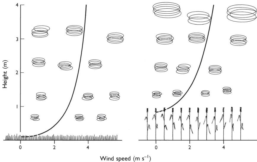
Fig. 6.11 Wind profiles and eddy size over short-grass and small-grain crops. The profiles are fit to Eq. 6.19.
