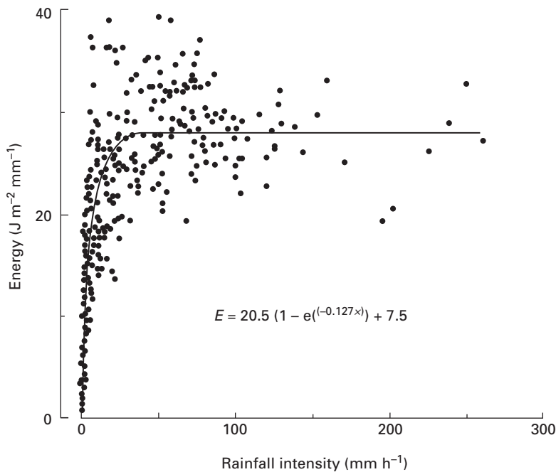
Fig. 12.7 Kinetic energy of rainfalls at Holly Springs, Mississippi, as a function of rainfall intensity. (Redrawn from McGregor & Mutchler 1977.)
