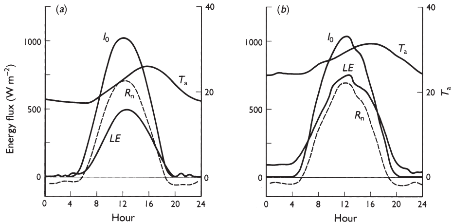
Fig. 6.9 (a) Hourly distribution of solar radiation, R_n , and latent heat exchanges ( LE ) of a ryegrass crop on a clear day in late spring at Davis, California, USA. Air temperature ( T_a ) is also shown. The daily totals of SW radiation ( I_o ) and R_n were near 31 \text{ MJ m}^{-2} and 19 \text{ MJ m}^{-2} , respectively; winds were light all day. (b) The same crop two days later with similar conditions except that winds were strong. In this case, LE > R_n . (Adapted from Pruitt 1964.)
