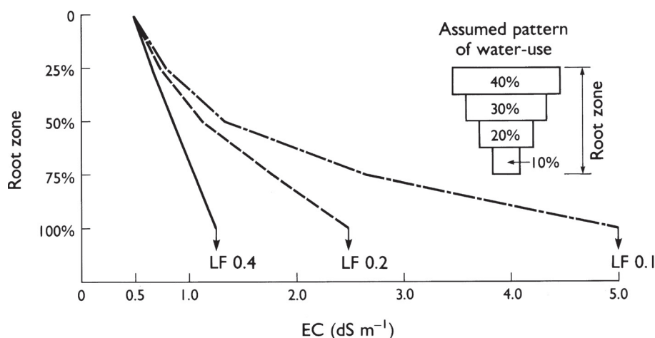
Fig. 14.2 Salinity profiles expected to develop after long-term use of water of EC = 1.0 \text{ dS m}^{-1} at leaching fractions (LF) = 0.1, 0.2, and 0.4 (after Ayers & Westcot 1985).
