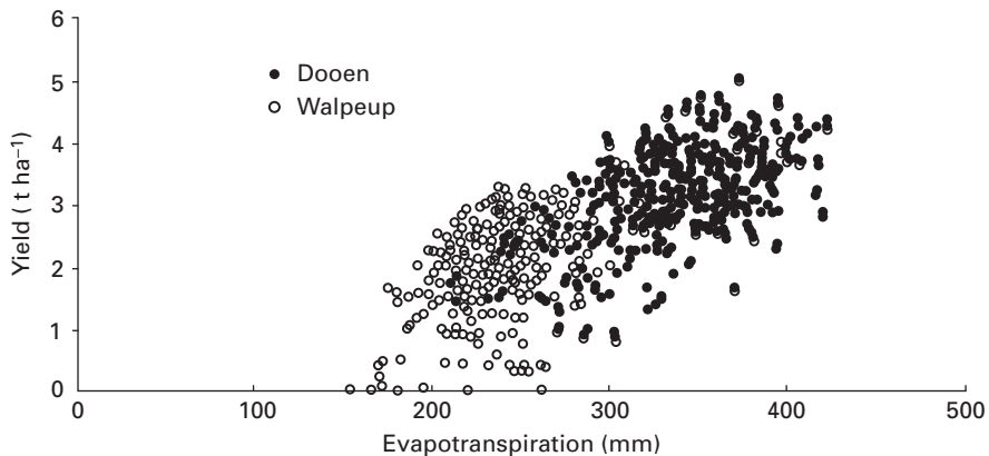
Fig. 13.9 Relationships between wheat yield and ET from the simulations presented in Fig. 13.8.
