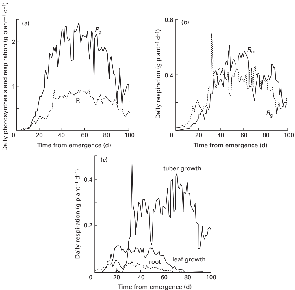
Fig. 11.3 (a) Simulated course of gross photosynthesis ( P_g ) and total respiration ( R ) for a potato crop at Aberdeen, Idaho, beginning with emergence on June 9. (b) Total respiration partitioned between R_m and R_g . (c) R_g partitioned among the costs of growing fine roots, leaves, and tubers. (After Ng & Loomis 1984.)
