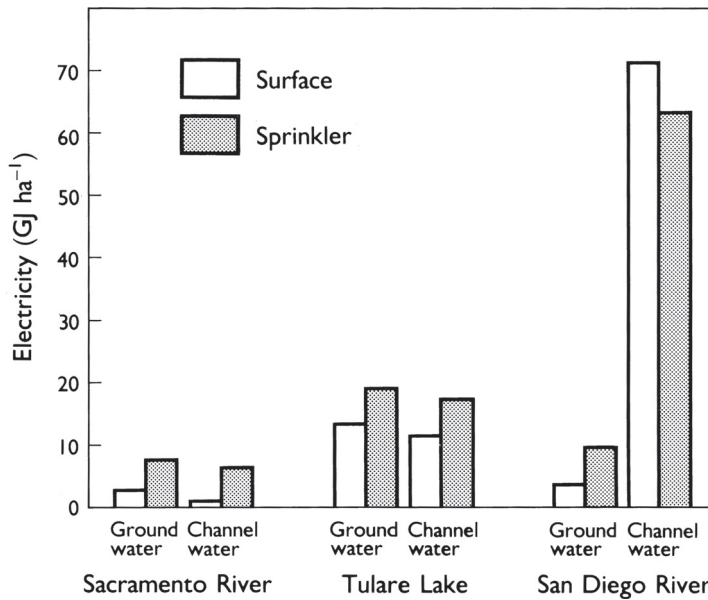
Fig. 14.5 The seasonal energy cost of irrigating alfalfa (950 mm) in three hydrologic basins in California. For each basin, a comparison is made between surface and sprinkler irrigation with water obtained from channels or from ground water. The calculations assume sprinklers use 20% less water than surface methods (after Knutson et al. 1977).
