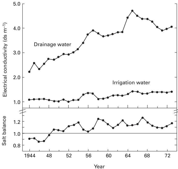
Fig. 14.8 Salinity of irrigation water, drainage water, and the annual salt balance (output/input) of the Imperial Valley irrigation area of southern California, USA, over the period 1944 to 1973 (after Kaddah & Rhoades 1976).
