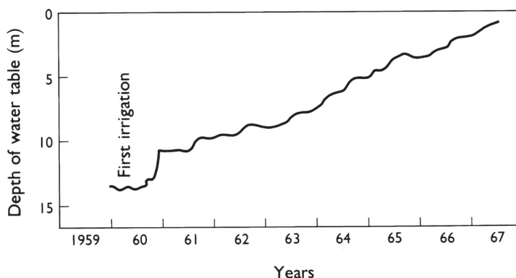
Fig. 14.3 Rising water tables under irrigation in Solano County, California (after Houston 1967).
