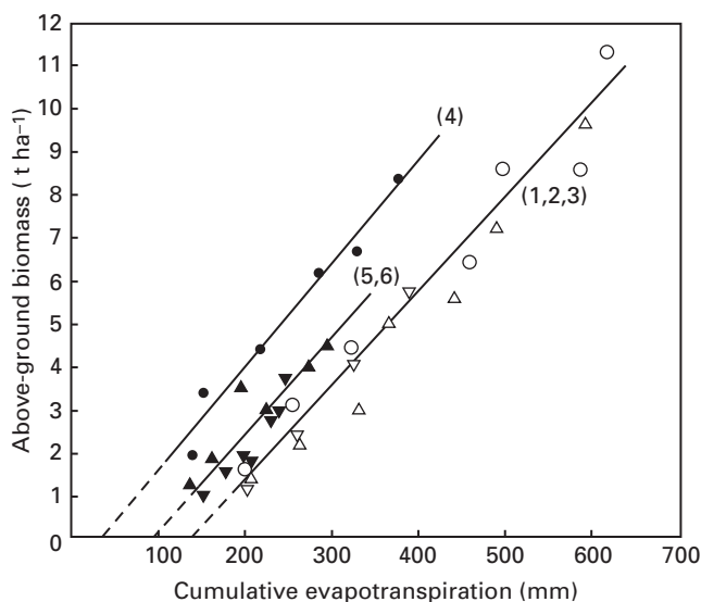
Fig. 9.19 Growth and progressive evapotranspiration (ET) of sunflower crops subjected to different irrigation sequences. Three linear relationships describe the responses. Transpiration efficiencies ( TE_B , gradients of the lines) were comparable for all crops but soil evaporation ( E_s ) (intercepts of lines with the abscissa) were different because of differences in wetting patterns and exposure of the soil surface. Differences in evapotranspiration efficiency ( \Delta B/\Delta ET ) were due to differences in E_s . (After Connor et al. 1985a.)
