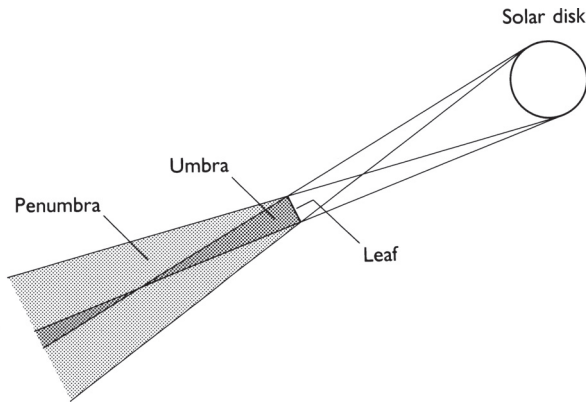
Fig. 6.3 Diffusion of a leaf's shadow due to penumbral effects caused by the finite size of the Sun. A full shadow from direct beam radiation occurs only within the umbra. The distance d , beyond which shadows are fully diffuse, equals approximately 100 times leaf width. (Not drawn to scale.)
