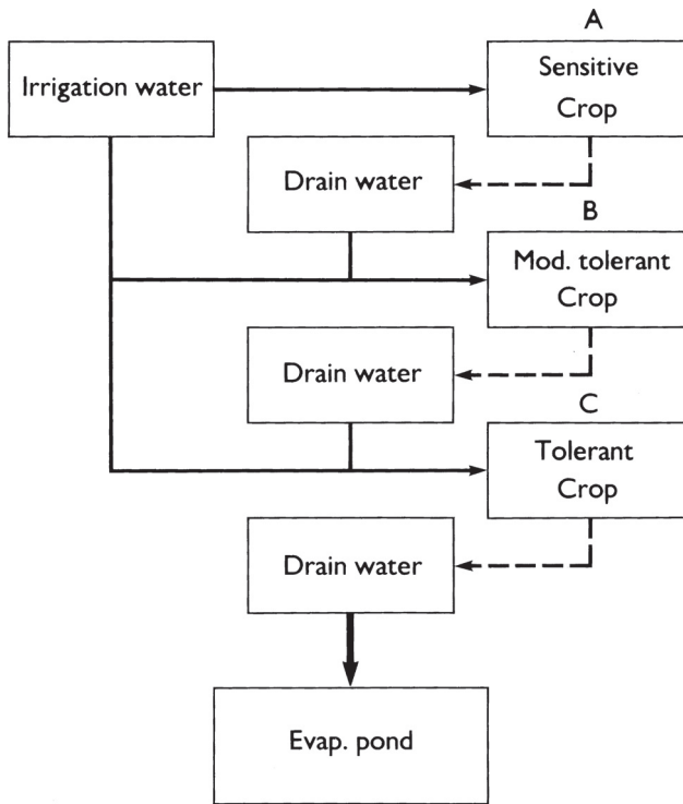
Fig. 14.6 A scheme for use of drainage water in irrigated agriculture. At each step, drainage water is mixed with high-quality water from the irrigation source. Crop types A, B, and C have increasing salinity tolerance.
