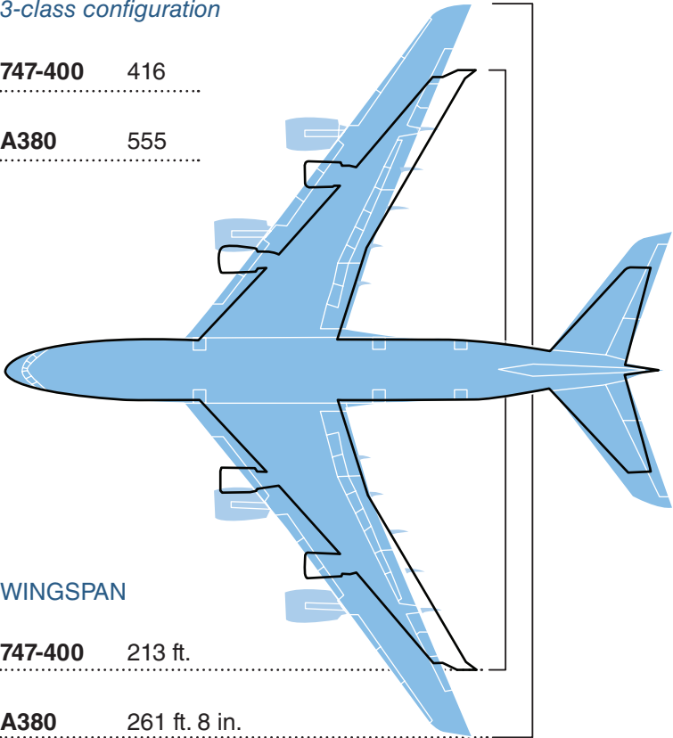
FIGURE II The Airbus A380 versus the Boeing 747-400
