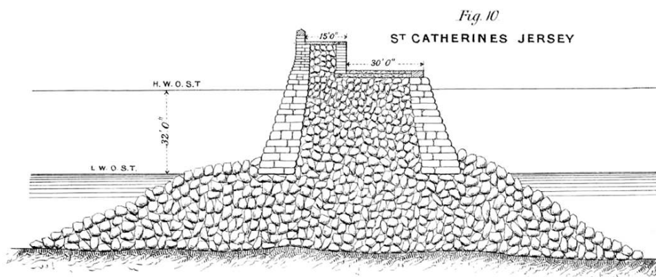
Fig. 10. Vertical breakwater at St Catherine's, Jersey
