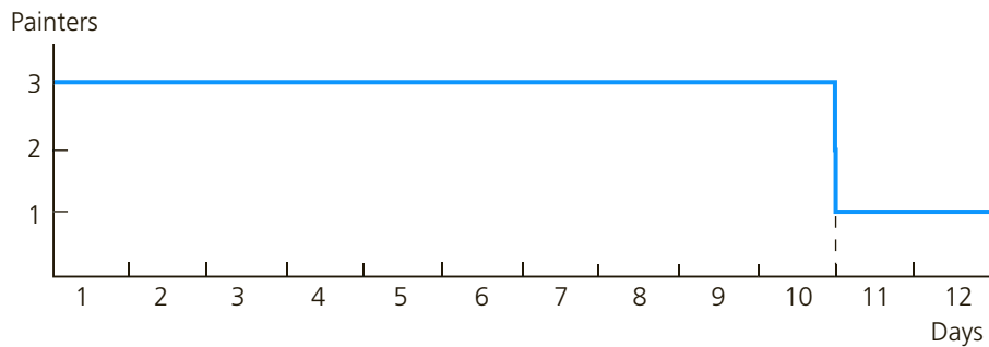
FIGURE 6.8 Resource-levelled Utilization for Painters
