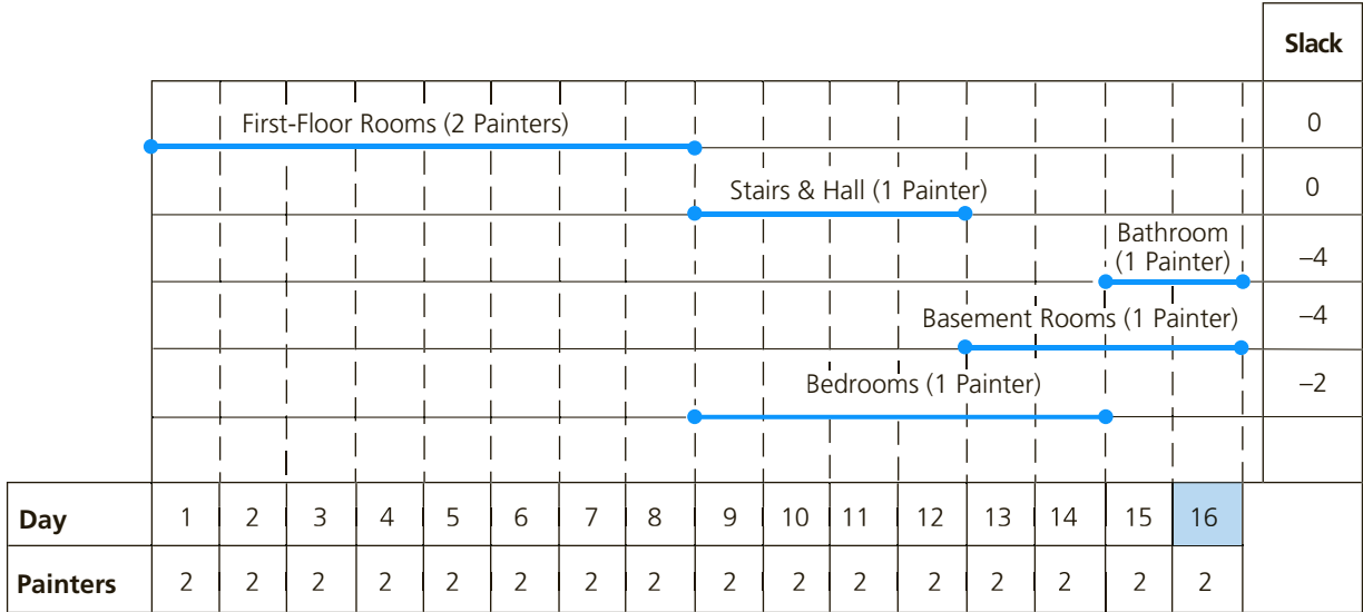
FIGURE 6.13 Third Resource Allocation
