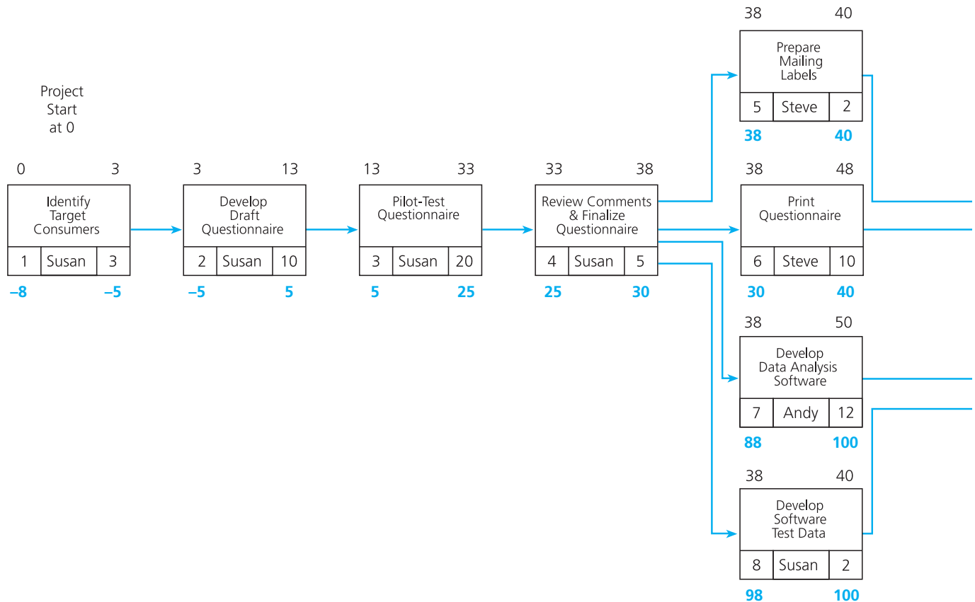
FIGURE 5.7 Network Diagram for Consumer Market Study Project, Showing Latest Start and Finish
