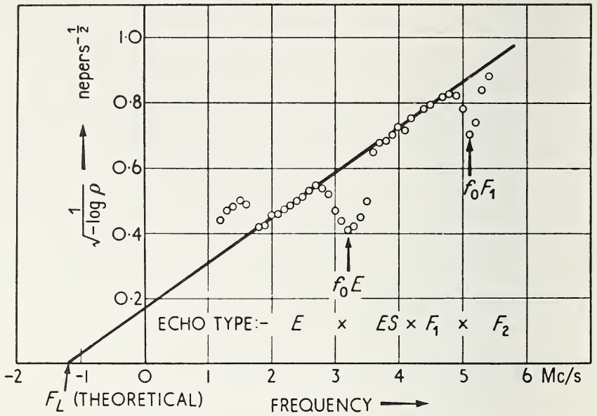
FIGURE 3.26. Variation of absorption with wave frequency (vertical propagation.)
