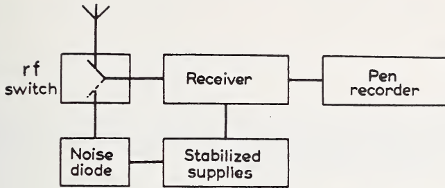
FIGURE 3.4. Block diagram of riometer.
