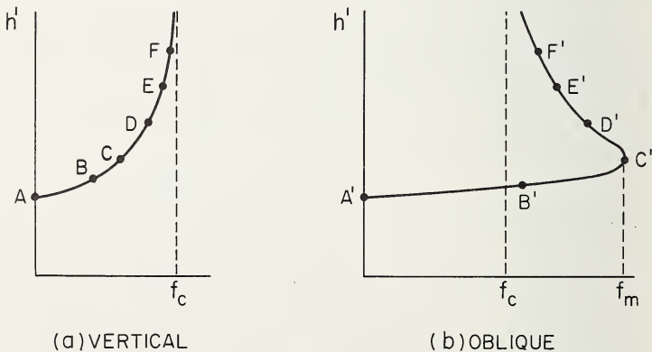
FIGURE 4.11. Corresponding vertical and oblique ionograms.
