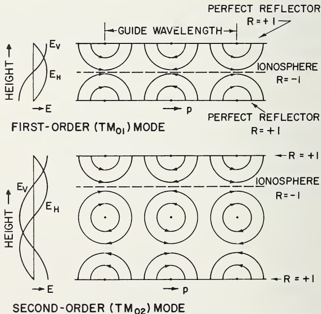
FIGURE 9.2. E field in an idealized earth-ionosphere waveguide.
