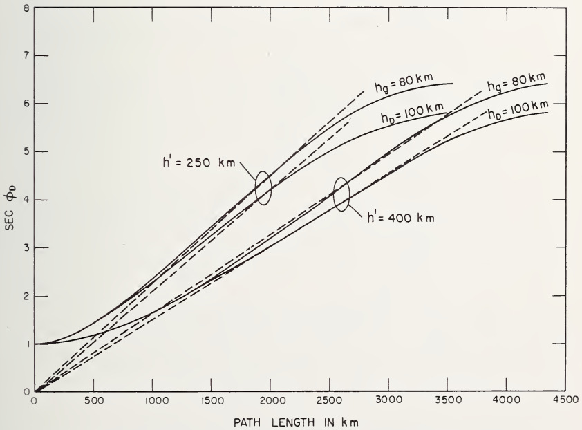
FIGURE 5.12. Variation of \text{sec } \phi_D with ground range for the model shown in figure 5.10.
