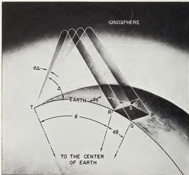
FIGURE 5.5. The divergence of a radio beam for a curved earth.
