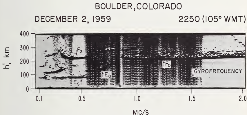
FIGURE 3.10. Low-frequency ionogram.
