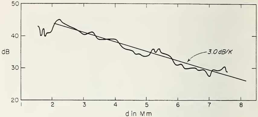
FIGURE 9.16. Experimental data showing attenuation rate over the Pacific.
