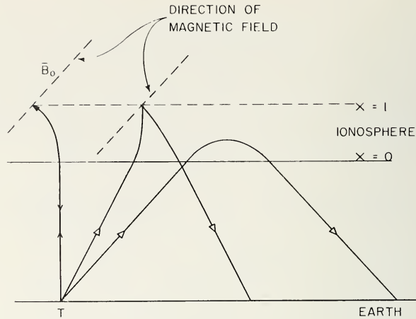
FIGURE 4.40. Sample ordinary ray paths for oblique propagation in magnetic meridian, showing the Spitzze.
