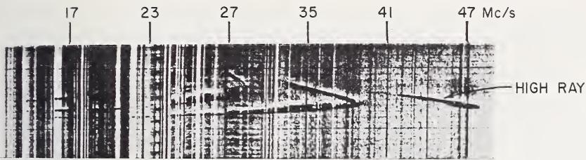
FIGURE 4.17. Ottawa-Slough ionogram, Nov. 14, 1957, 1556 UT.
