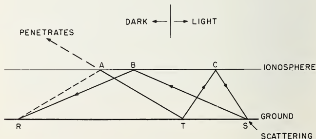
FIGURE 4.24. Importance of ground scatter.
