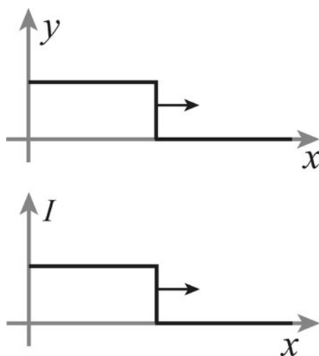
Figure 10.5.3 When you first apply a voltage to the left end of a transmission line, you generate a wavefront in the voltage which propagates down the line, accompanied by a wavefront in the current.
