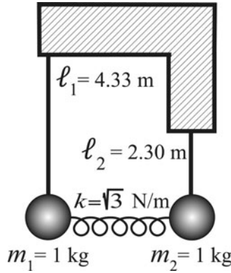
Figure 6.3.1 An example of an asymmetric coupled pendulum system with equal masses.
