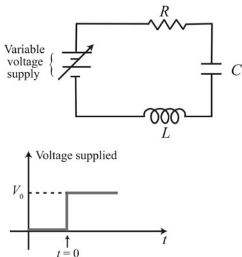
Figure 3.P.1 An RLC circuit suddenly has a nonzero voltage applied to it.
