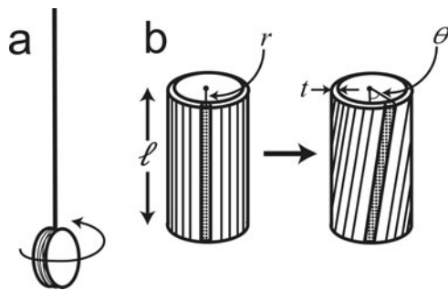
Figure 2.5.1 a: A yo-yo twisting on the end of its string. b: Twisting a thin-walled tube.
