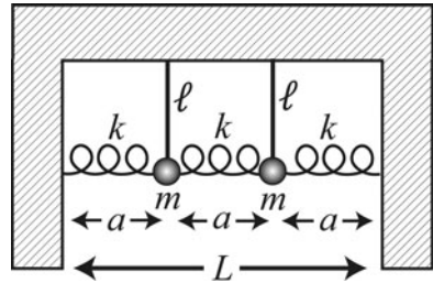
Figure 6.P.3 A set of two coupled pendula.
