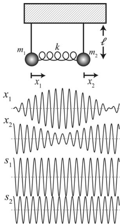
Figure 6.7.2 Top: Coupled pendula with unequal masses. For the example discussed in the text, m_1 = 1 kg, m_2 = 2 kg, \ell = 1 m, k = 1 N/m, and g = 10 m/s 2 . Bottom: Position versus . time for each of the two masses ( x_1 and x_2 ) and for each of the normal mode coordinates ( s_1 and s_2 ).
