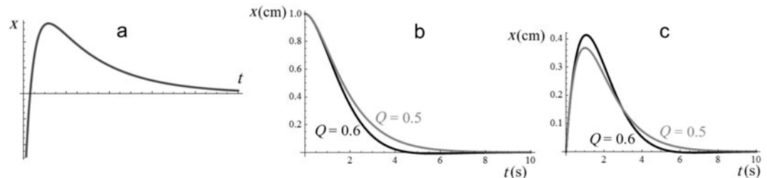
Figure 3.5.1 a: In the overdamped case, there is at most one crossing of the equilibrium point; even this can only occur if the initial velocity is high and the initial position is close to x = 0 . b and c: Comparison of underdamped and critically damped systems. In part b, the initial velocity is zero but the initial position is nonzero. In part c, the initial position is zero but the initial velocity is non-zero. In both cases, the underdamped system ( Q = 0.6 ) returns to equilibrium a little more quickly than the critically damped system.
