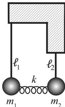
Figure 6.2.1 An asymmetric coupled pendulum system.
