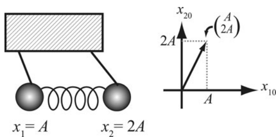
Figure 5.6.1 If we require the initial velocities of both pendula to be zero, then any initial condition can be depicted as a vector on the plane shown in the right part of the figure. The vector can be specified in column matrix format, with x_{10} in the top line and x_{20} in the bottom line.
