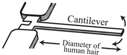
Figure 3.4.1 A micromachined silicon cantilever used to detect the pressure or molecular weight of gas via the change in the oscillation frequency due to damping. The cantilever is produced by a combination of photolithography and etching (“micromachining”) and is suspended a few \mu\text{m} above the substrate, so that it can oscillate in a plane parallel to the substrate, as shown in the schematic diagram. Top image reprinted with permission from Y. Xu, J. -T. Lin, B. W. Alphenaar, and R. S. Keynton, Appl. Phys. Lett. 88 , 143513 (2006). Copyright 2006, American Institute of Physics.
