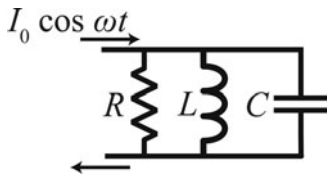
Figure 4.P.4 A parallel RLC oscillator.
