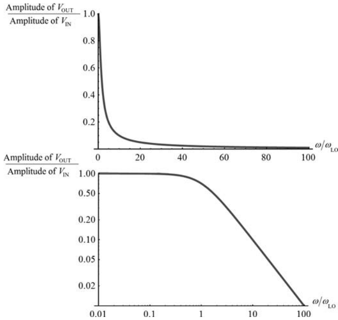
Figure 1.10.3 Amplitude ratio for the low-pass filter shown in figure 1.10.2b. Top: linear axes. Bottom: same data with log-log axes.
