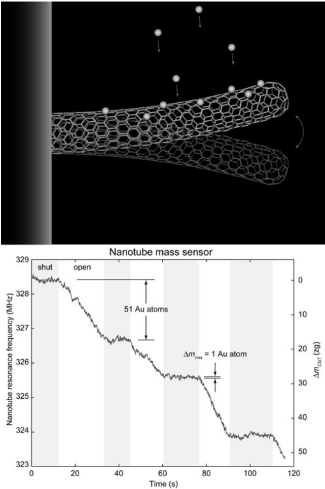
Figure 2.6.2 Deposition of gold atoms onto a cantilever made from a carbon nanotube (shown schematically at the top) increases the mass of the cantilever, thus decreasing the vibration frequency (left vertical scale of the graph). During the shaded time periods (e.g. 60 s to 76 s), no atoms are deposited, so the frequency is constant. During the unshaded periods, atoms are added, and the frequency decreases. Images Courtesy Zettl Research Group, Lawrence Berkeley National Laboratory and University of California at Berkeley.
