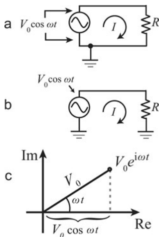
Figure 1.10.1 a: A signal generator (denoted by a sine wave inside a circle) connected to a resistor. b: Same circuit, drawn in the more conventional way using the ground symbol. c: Complex representation for an AC voltage.
