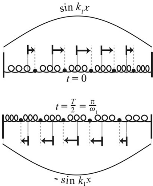
Figure 7.5.3 Displacements at t = 0 and half a period later for the mode n = 1 for longitudinal oscillations.
