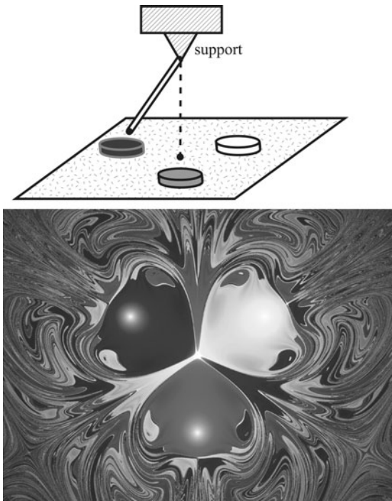
Figure 4.8.2 Top: In the magnetic pendulum, a rigid rod is free to swing from a top support. The bottom of the rod is attached to a small piece of iron, which is attracted to the three magnets on the surface below. Bottom: Basins of attraction for the three magnets, as simulated on a computer using an approximate model for the forces. If the pendulum is released from rest in any of the white regions, it eventually winds up pointing to the white magnet. If it is released from one of the black regions, it winds up at the black magnet, and similarly for the gray regions. The overall shading indicates the length of time required for the pendulum to settle to a final resting place, with darker shading indicating a longer time. (Lower image courtesy of and © Paul Nylander, www.bugman123.com )
