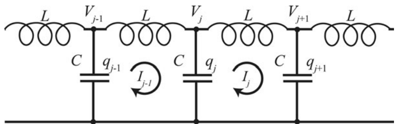
Figure 9.7.1 Model for a transmission line.
