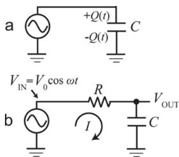
Figure 1.10.2 a: A signal generator connected to a capacitor. b: An RC low-pass filter.
