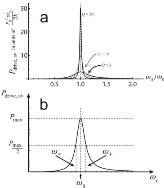
Figure 4.3.3 a: Power delivered by drive force to oscillator (averaged over a cycle) as a function of \omega_d . This is called the power resonance curve. b: Definition of FWHM.
