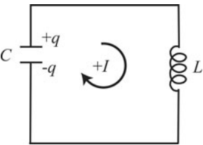
Figure 1.5.1 Electrical oscillator.
