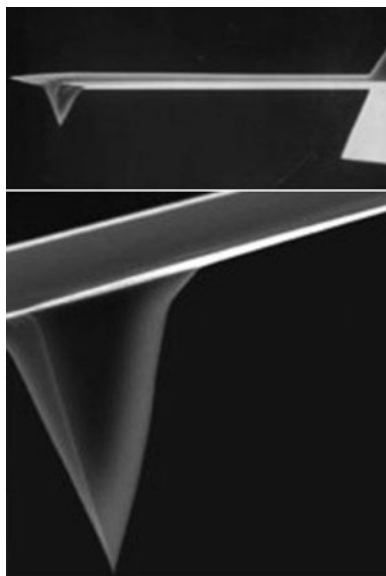
Figure 4.2.3 The cantilever for an atomic force microscope (top image) must have a moderately high Q , so that a small amplitude vibration applied at the base of the cantilever results in a vibration amplitude at the tip of about 100 nm. The length of the cantilever is 125 \mu\text{m} , about the same as the diameter of a human hair. The pyramid-shaped tip located at the end of the cantilever (bottom image) must be very sharp to obtain high resolution images. (Image courtesy of Veeco Instruments Inc.)
