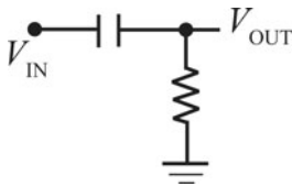
Figure 1.P.2 The RC high-pass filter.
