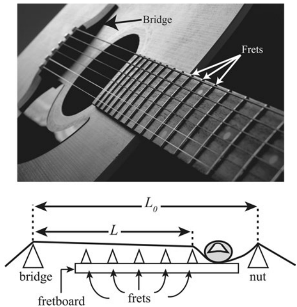
Figure 7.P.1 Top: The frets on a guitar allow the guitarist to vary the effective length of each string in a controlled way. Bottom: side view of a finger pressing a string down behind a fret. (Top image © Milinz | Dreamstime.com)
