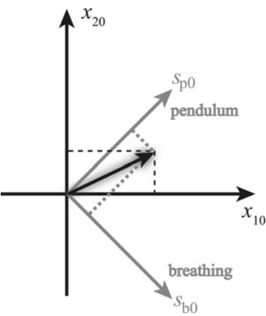
Figure 5.6.3 The black vector can be resolved into components either along the x_{10} and x_{20} axes (as shown by the black dashed lines) or along the pendulum mode and breathing mode axes (as shown by the gray dashed lines).
