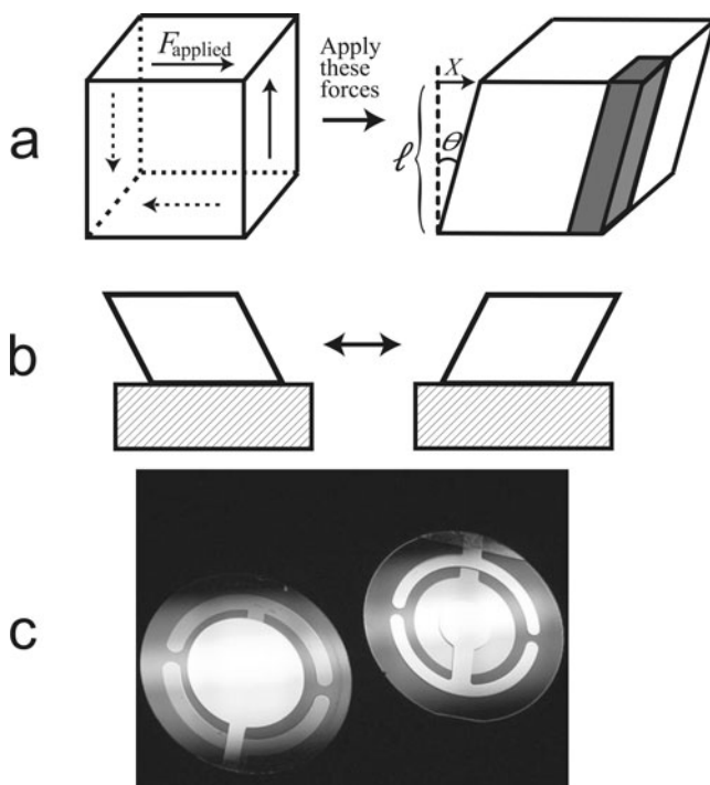
Figure 2.4.1 a: A force applied parallel to a face is called a shear force. For static equilibrium, forces must be applied to three other faces of the cube, as shown. This results in shear strain, as shown on the right. By imagining that we divide the cube into small parallel beams, such as that shown shaded on the right, we can see that the force with which the cube resists the shear deformation is proportional to the area of the top surface. b: Shear oscillations (side view). c: Front and back surfaces of a crystal from a quartz crystal microbalance, with gold electrodes applied. Image from Wikimedia Commons.
