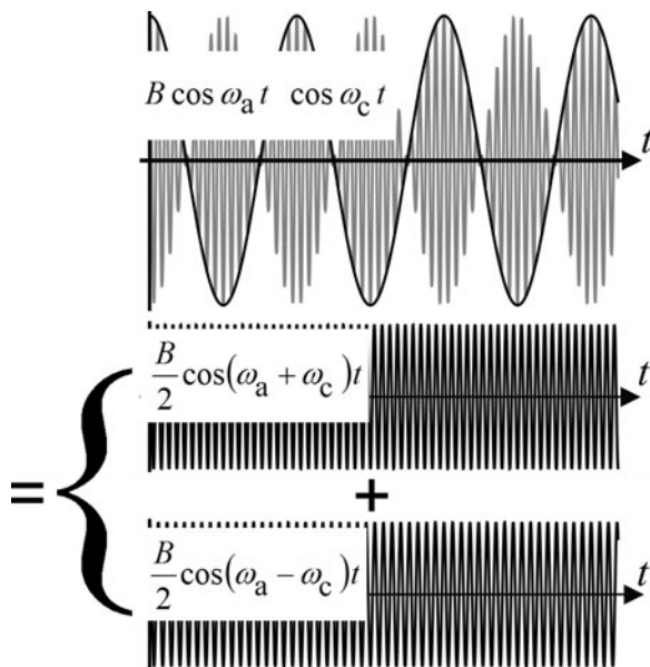
Figure 9.12.5 A rapidly oscillating carrier wave multiplied by a simple sinusoidal envelope function is equal to the sum of two sinuoids, each at an angular frequency close to that of the carrier.
