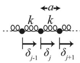
Figure 7.5.2 Quantities defined for longitudinal oscillations.
