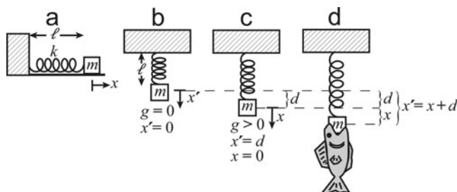
Figure 1.4.1 a: Mass on a frictionless surface. Important: The vertical line and horizontal arrow marked “ x ” at the bottom of the figure show the definition of x : it is zero at the position of the vertical line, and becomes positive in the direction of the arrow. In this example, this means that when the mass moves to the right of the position shown, x is positive, whereas if the mass moves to the left of the position shown then x is negative. We will use this combination of line and arrow to define the displacement x throughout the book. b–d: Mass on a vertical spring. The direction of positive x is downward.
