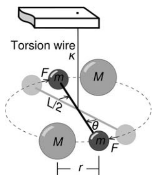
Figure 2.5.2 Schematic diagram of the Cavendish experiment. (Figure by Chris Burks.)
