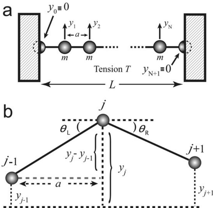
Figure 7.1.1 a: A massless string under tension T with small beads equally spaced along its length. b: Geometry needed for calculating the force on bead j .
