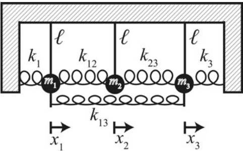
Figure 6.4.1 system of three coupled pendula with all possible couplings.
