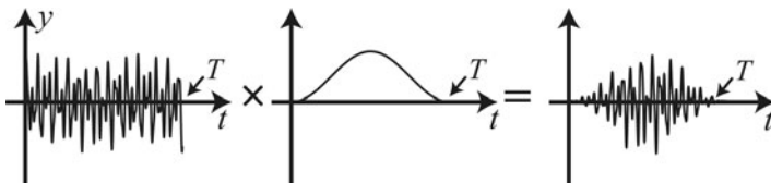
Figure 8.6.2 Because the DFT assumes the function has periodicity T , problems occur if (as is usually the case) the beginning and ending values of the sampled waveform (left) are not equal; this causes a sharp step in the assumed waveform. To avoid this problem, the sampled input waveform (left) is multiplied by a windowing function (center) to produce a waveform (right) that goes to zero at the beginning and end of the time interval T . This example shows the “Hanning window”, one of the most common windowing functions; it is simply an offset cosine.
