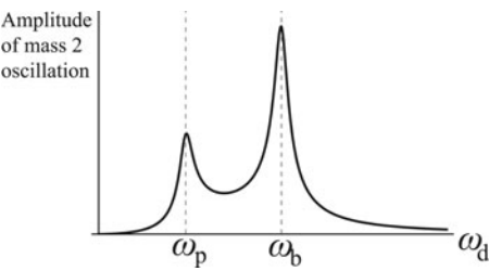
Figure 5.9.1 For a damped driven coupled oscillator system, each part of the system shows a resonant response at the frequencies corresponding to each of the normal modes. This shows the amplitude of response of mass 2 of a two-pendulum system, with the drive force applied to mass 1. The curve for the amplitude of response for mass 1 is similar.
