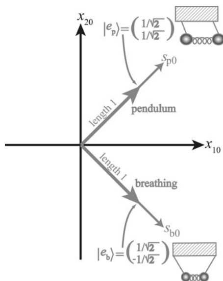
Figure 5.6.2 The eigenvectors for the symmetric coupled pendulum system.
