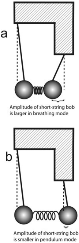
Figure 6.3.2 Normal modes for the system shown in figure 6.3.1. a: breathing mode. b: pendulum mode.
