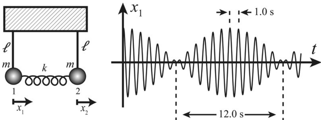
Figure 5.P.3 Left: A pair of coupled pendula. Right: The position of the left mass as a function of time.
