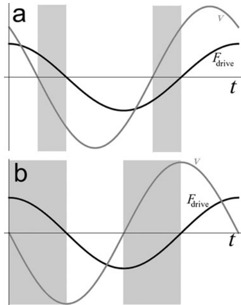
Figure 4.3.1 a: F_{\text{drive}} and v for the case \delta = 45^\circ . In the shaded regions, the two have opposite sign, so P_{\text{drive}} is negative, meaning that the oscillator supplies power to the drive. In the other regions, F_{\text{drive}} and v have the same sign, so P_{\text{drive}} is positive, and the drive supplies power to the oscillator. (Since F_{\text{drive}} and v have different units, the vertical scales cannot be compared.) b: F_{\text{drive}} and v for \omega_d \rightarrow 0 ; in this limit \delta \rightarrow 0 , so F_{\text{drive}} and v are out of phase by \pi/2 . In the shaded regions, the two have opposite sign, so P_{\text{drive}} is negative, meaning that the oscillator supplies power to the drive. In the other regions, F_{\text{drive}} and v have the same sign, so P_{\text{drive}} is positive, and the drive supplies power to the oscillator. (The velocity scale for this plot is greatly magnified compared to part a; for small \omega_d , the velocity is also small.)
