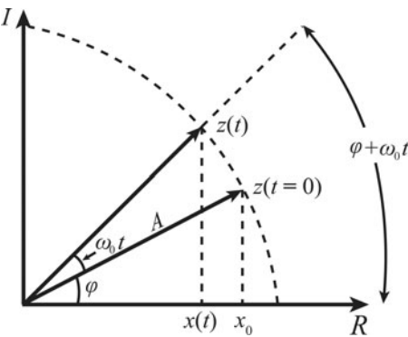
Figure 1.9.1 Complex plane representation of SHM.
