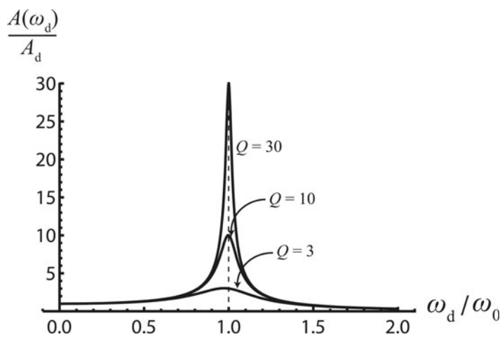
Figure 4.2.1 Dependence of steady state amplitude on \omega_d / \omega_0 .
