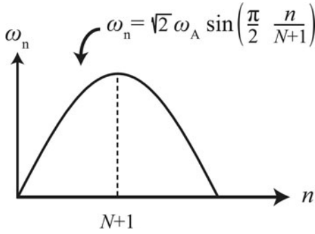
Figure 7.6.1 Angular frequency vs. mode index for a beaded string.
