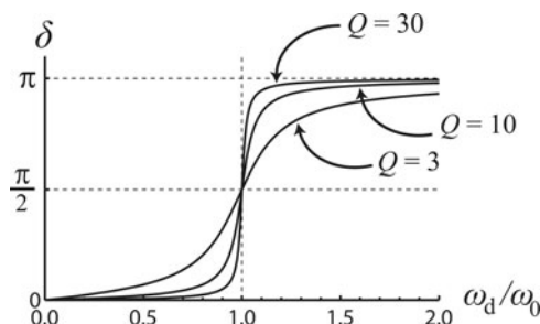
Figure 4.2.2 Phase shift \delta of the steady-state response.
