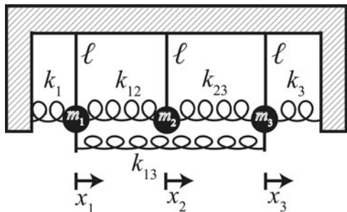
Figure 6.7.1 The same system of three coupled pendula as shown in figure 6.4.1.
