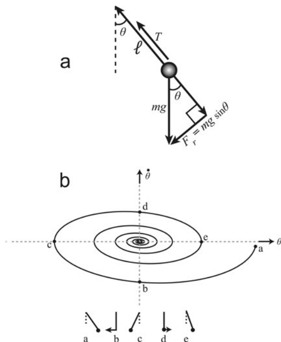
Figure 4.8.3 a: Free body diagram for a pendulum. b: Phase space plot for the damped, undriven pendulum.
