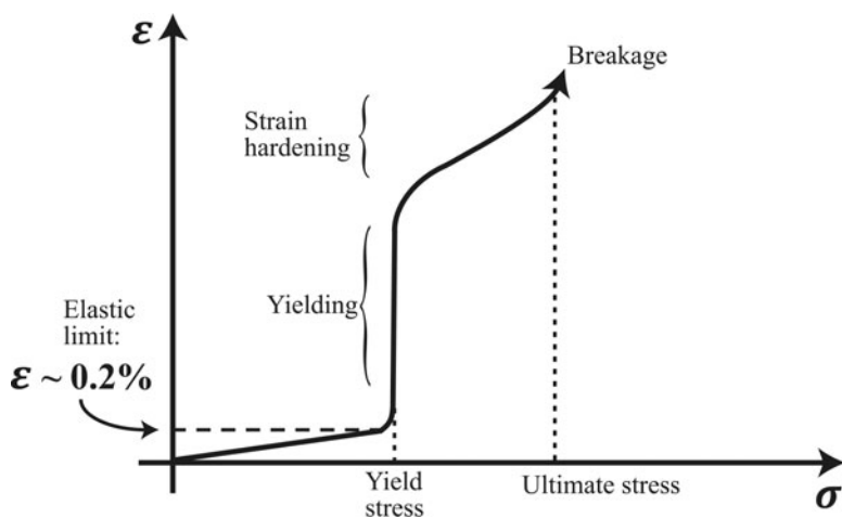
Figure 2.3.2 Strain vs. stress for a typical metal beam.
