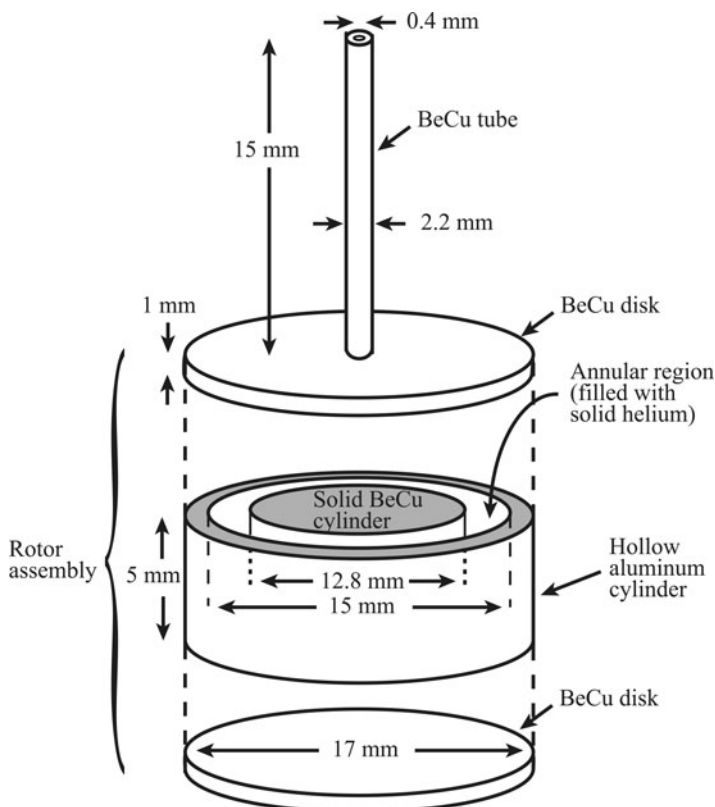
Figure 2.P.2 Torsional oscillator used to detect the transition to supersolid helium.
