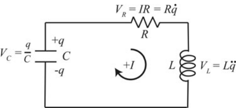
Figure 3.2.1 Damped electrical oscillator.
