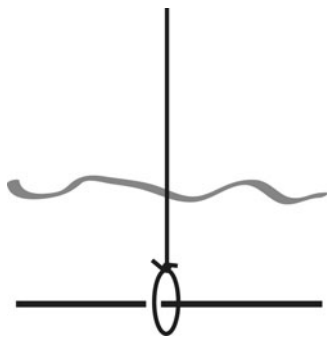
Figure 10.3.2 By connecting a rope to a massless ring immersed in a suitably chosen damping fluid, we can suppress reflections.
