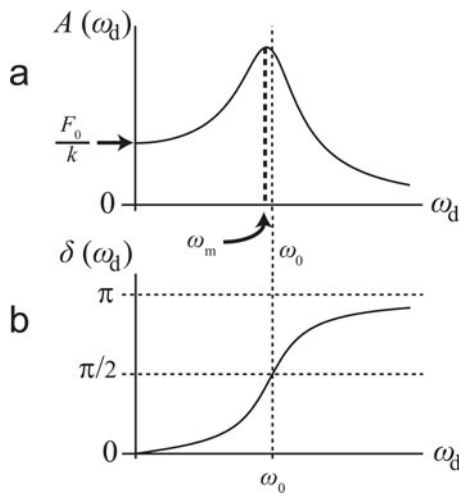
Figure 4.1.5 Amplitude and phase of a damped driven oscillator as a function of the angular frequency of the drive.
