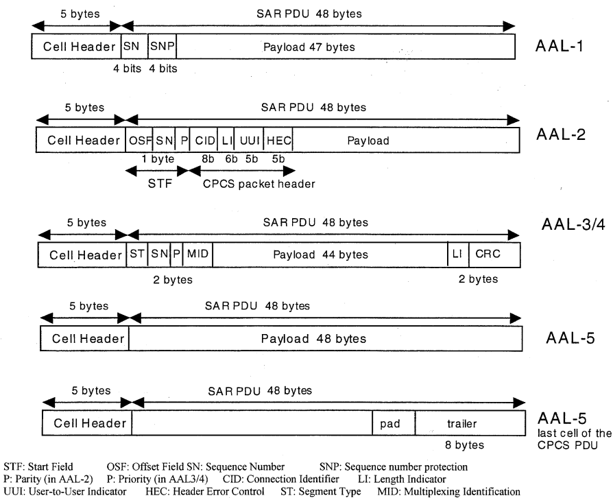
Figure 22.3-3. SAR PDUs for the AAL protocols.
