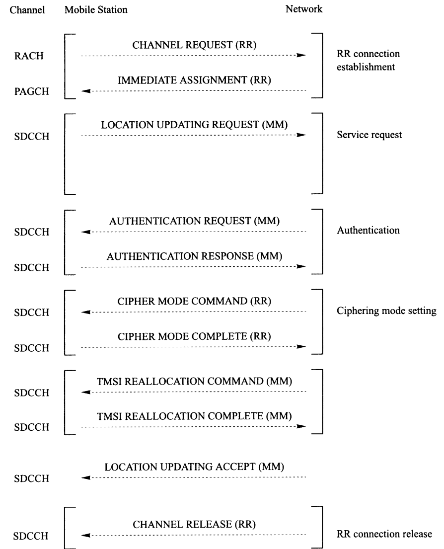
Figure 12.8-1. Location updating. (From GSM 04.08 Version 4.10.0. Courtesy of ETSI.)
