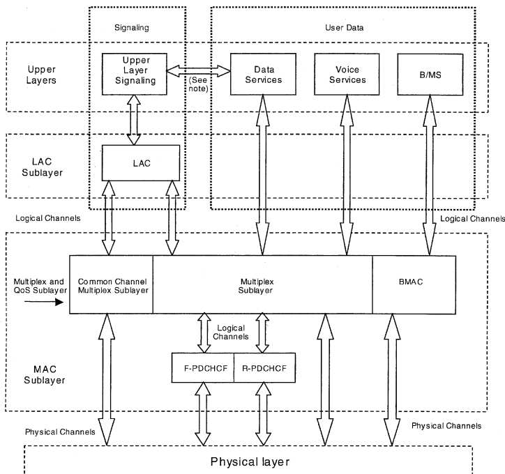
Figure 13.3-5. Detailed protocol structure for the cdma2000® air interface.
