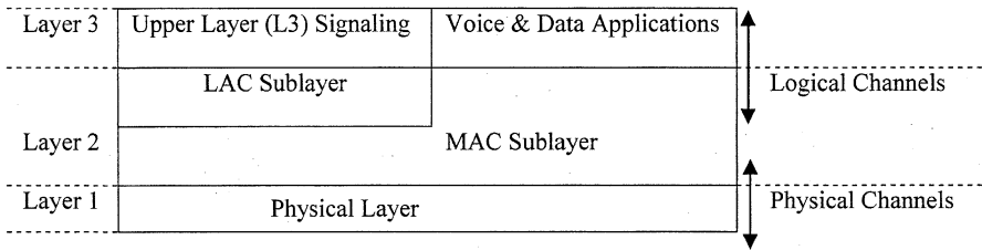
Figure 13.3-2. Protocol stack and physical and logical channels for cdma2000®.
