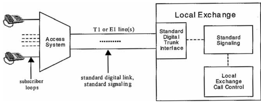
Figure 1.8-2. Access systems.
