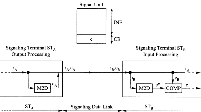
Figure 5.2-6. Cyclic redundancy checking.
