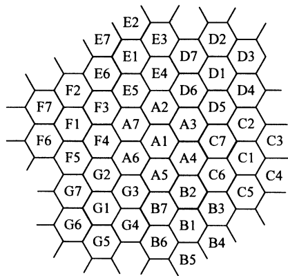
Figure 12.1-5. Seven-cell clusters.
