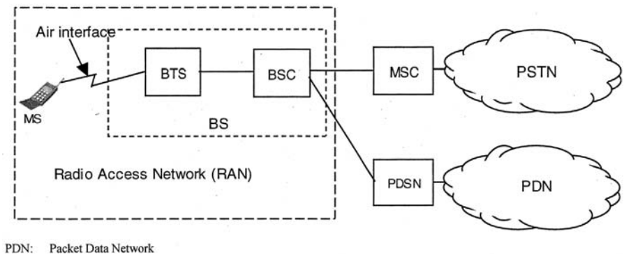
Figure 13.3-1. cdma2000® network and interfaces.
