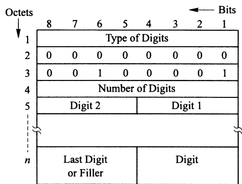
Figure 19.5-2. Format of Par.11 (Digits). (From IS-41.5-B. Reproduced with permission of TIA.)
