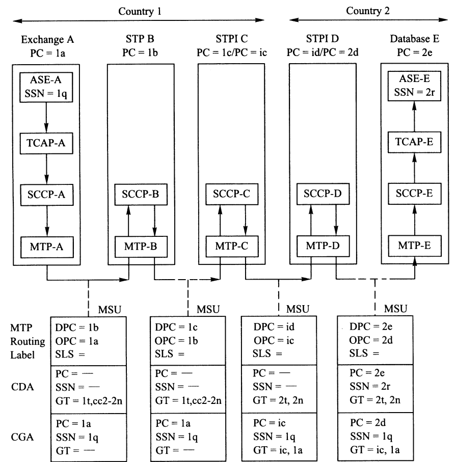
Figure 15.3-5. Address information in the first SCCP Unitdata message of an international transaction.
