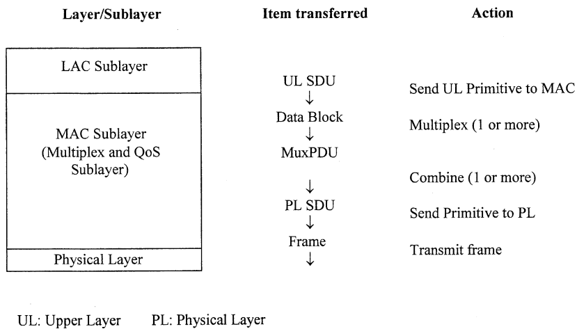
Figure 13.3-9. Transmit operation for the Multiplex and QoS sublayer.
