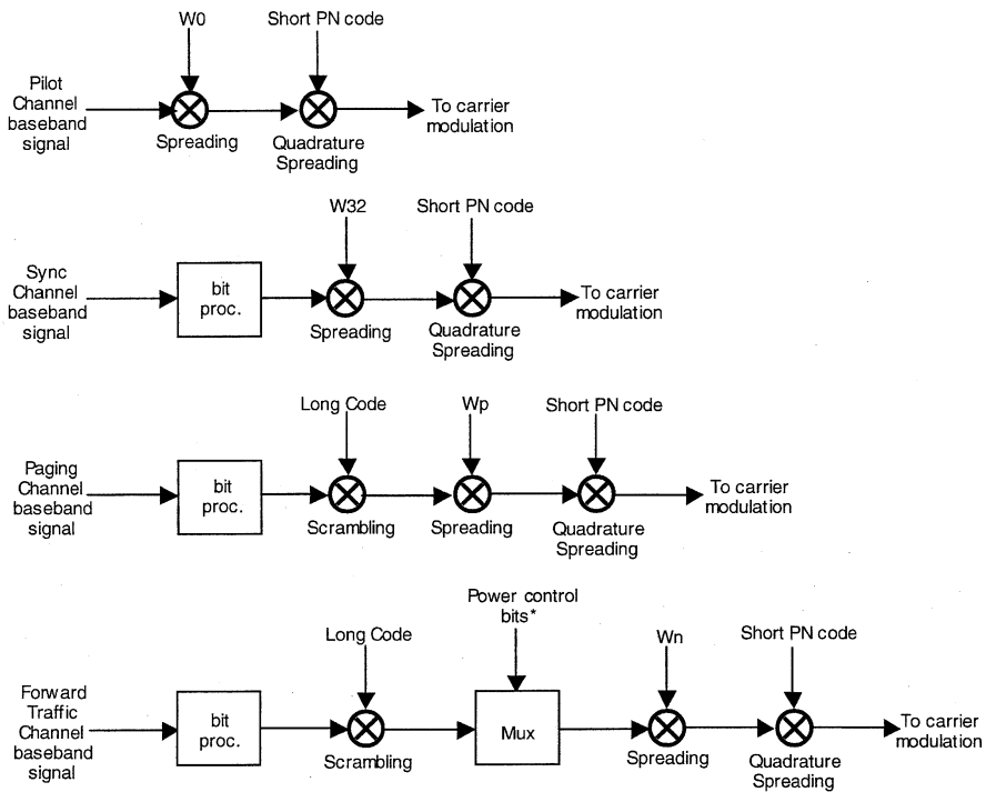
Figure 13.2-1. Conceptual view of Forward CDMA Channel bit processing for IS-95 B.
