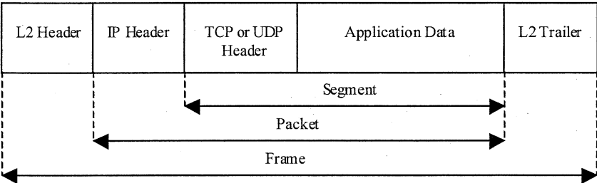
Figure 20.2-2 TCP/IP PDU.
