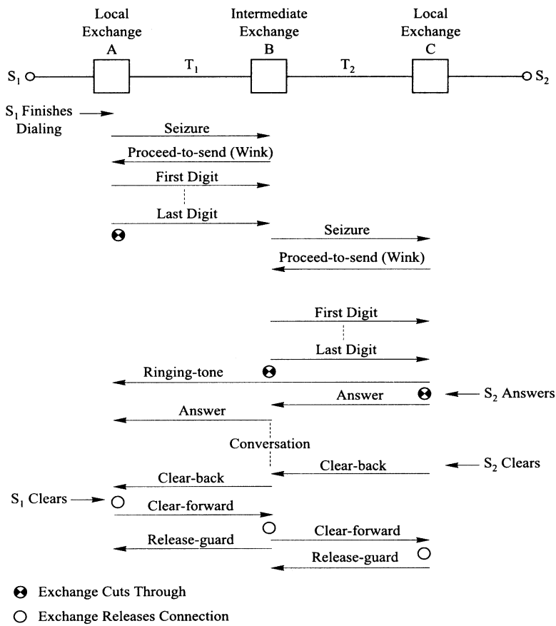
Figure 4.1-1. Interexchange signaling.
