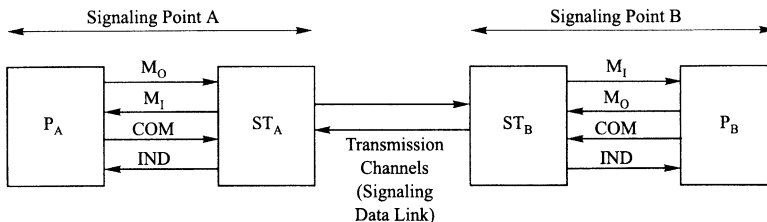
Figure 5.2-1. Signaling link.
