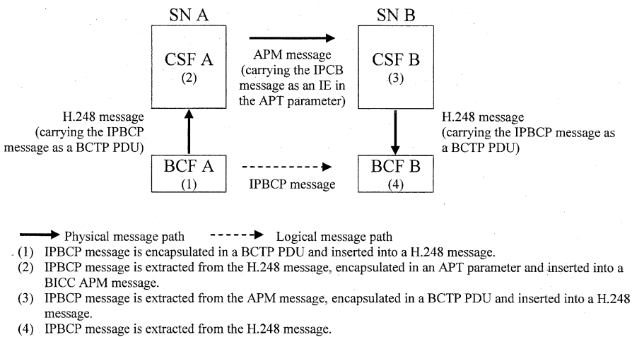
Figure 21.6-5. IPBCP tunneling.
