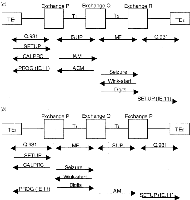
Figure 11.4-2. Connection with ISUP-MF interworking.
