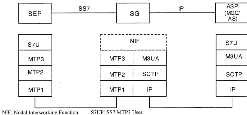
Figure 21.5-14. M3UA signaling architecture. (From RFC 3332 [21].)
