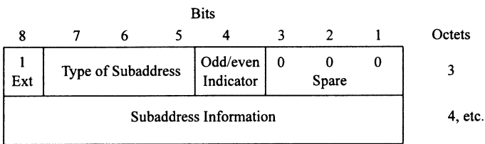
Figure 10.3-5. Formats of IE.A (called party subaddress) and IE.5 (calling party subaddress). (From Rec. Q.931. Courtesy of ITU- T.)
