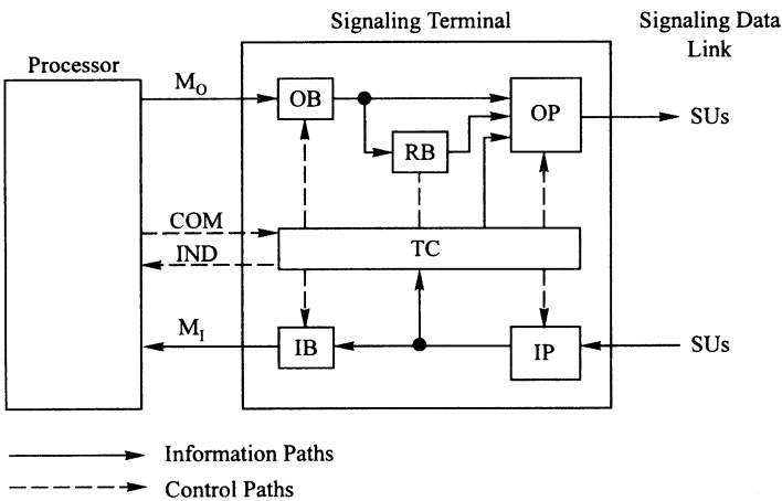
Figure 5.2-4. Signaling terminal.
