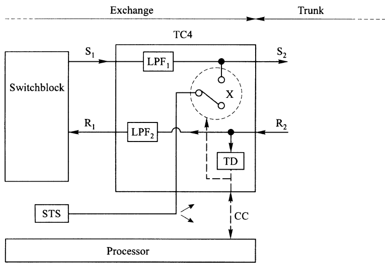
Figure 4.4-1. Four-Wire analog trunk circuit (TC4) for out-of-band supervision signaling.
