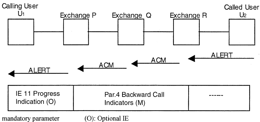
Figure 11.3-4. Mapping of Q.931 ALERT messages and ISUP Address Complete message (ACM).
