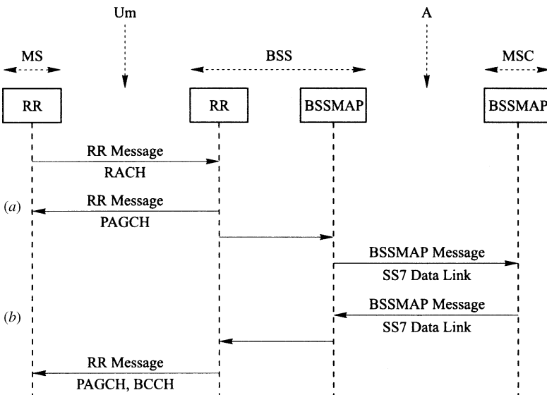
Figure 12.7-3. Transfer of RR messages. (From GSM 04.07 Version.10.0. Courtesy of ETSI.)
