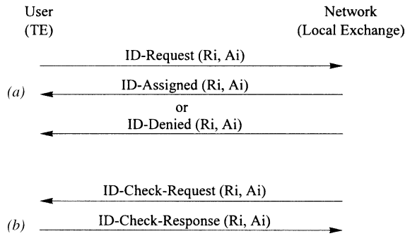
Figure 10.2-6. TEI management procedures: (a) TEI assignment and (b) TEI checking. All TEI management message are sent in UI frames with TEI = 127 and SAPI = 63. (From Rec. Q.921. Courtesy of ITU-T.)
