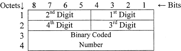
Figure 11.2-10. Format of Par.11: closed user group interlock code. (From Rec. Q.763. Courtesy of ITU-T.)
