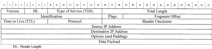
Figure 20.2-4 IP packet format.
