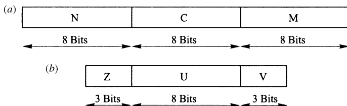
Figure 7.2-1. Point code formats: (a) ANSI No. 7 and (b) CCITT No. 7. (From Rec. Q.708. Courtesy of ITU-T.)
