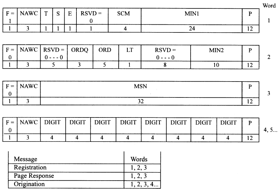
Figure 12.4-3. Mobile control messages on Reverse Control Channel. (From EIA/TIA 553. Reproduced with permission of TIA.)
