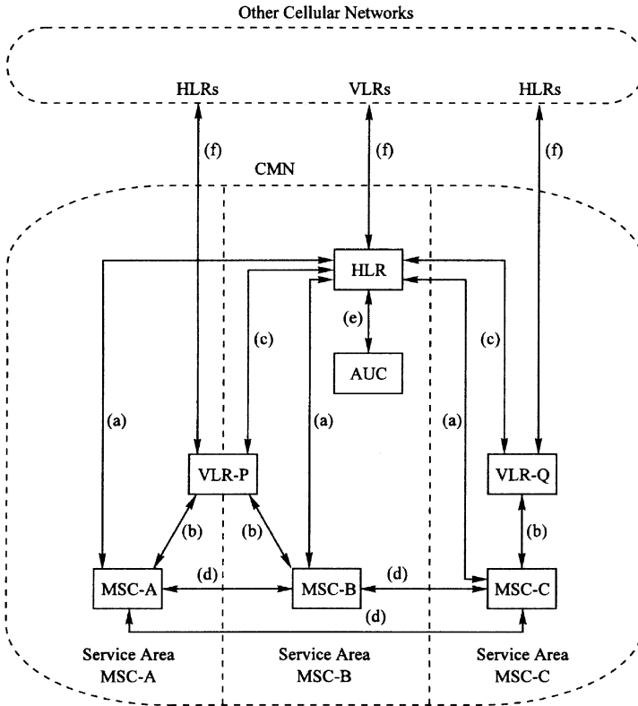
Figure 19.1-1. IS-MAP related equipment entities and interfaces.
