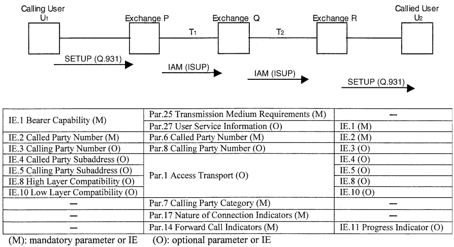
Figure 11.3-3. Mappings of Q.931 SETUP messages and ISUP IAM message.
