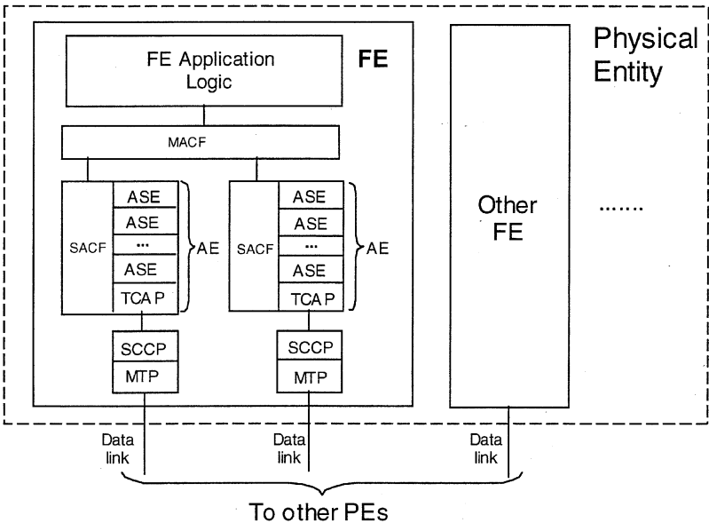
Figure 18.4-2 INAP architecture in a physical entity.
