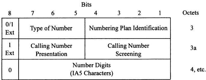
Figure 10.3-4. Formats of IE.2 (called party number) and IE.3 (calling party number) (From Rec. Q.931. Courtesy of ITU-T.)
