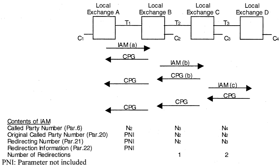
Figure 11.6-2. Call forwarding.
