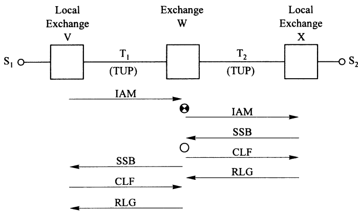
Figure 9.3-3. Release of a failed connection. Signaling path is TUP all the way.
