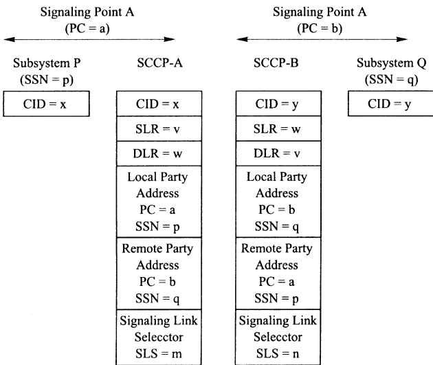
Figure 15.4-2. Connection records.
