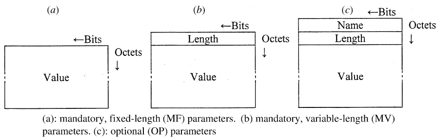
Figure 11.2-1. ISUP parameters.
