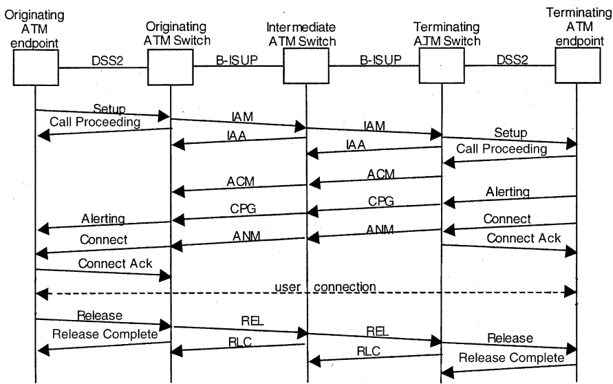
Figure 22.7-6. Example of B-ISUP call setup sequence with DSS-2 interworking.
