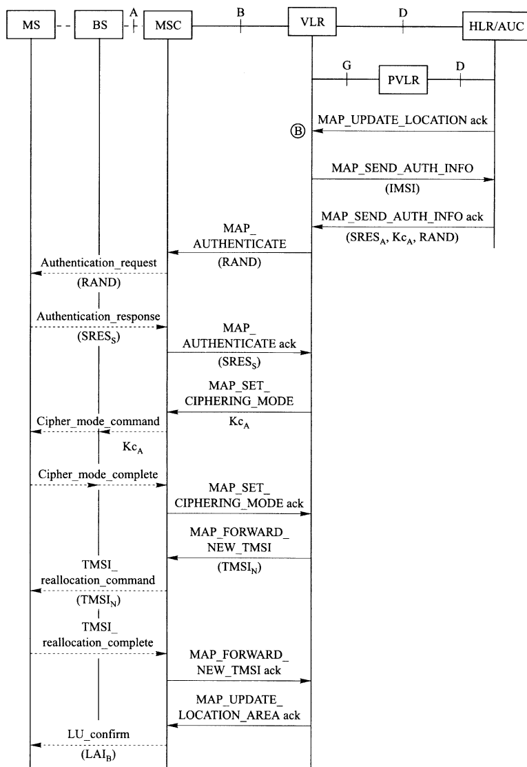
Figure 19.7-7. Final operations for location area updating. (From GSM.09.02-Version 4.9.0. Courtesy of ETSI.)
