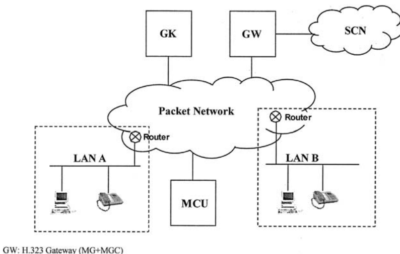
Figure 21.2-1. Example of a H.323 network.
