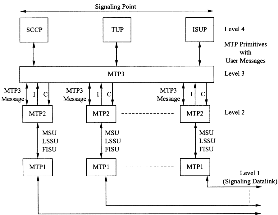
Figure 8.1-2. MTP structure.
