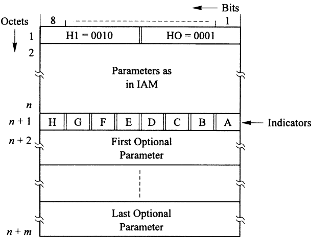
Figure 9.2-2. Initial Address Message with Additional Information (IAI). (From Rec. Q.723. Courtesy of ITU-T.)
