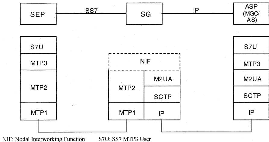
Figure 21.5-9. M2UA signaling architecture. (From RFC 3331 [19].)
