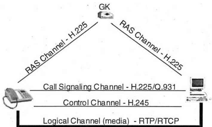
Figure 21.2-4. H.323 channels.
