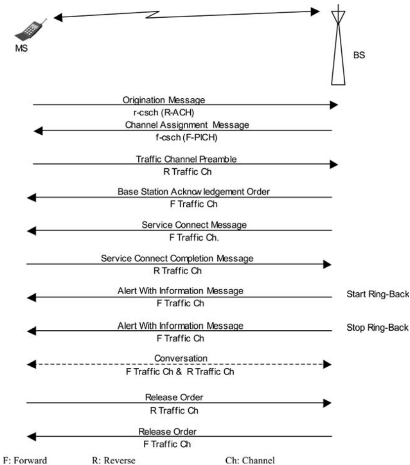
Figure 13.3-14. Example of message flow on the Forward and Reverse Traffic Channels for a MS-originated call.
