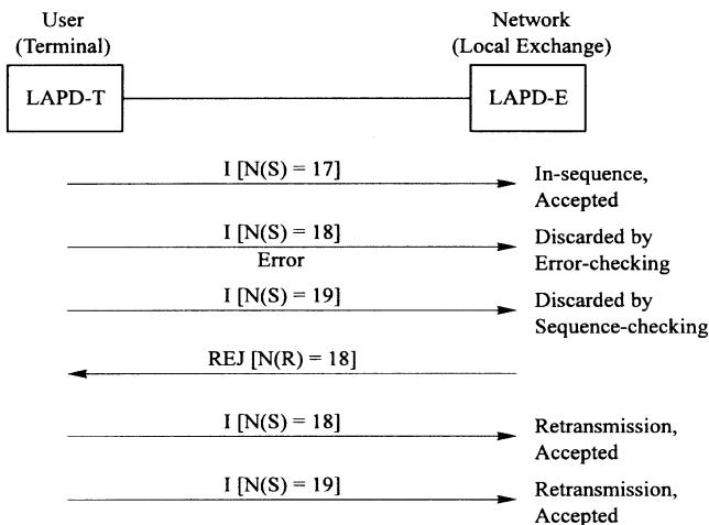
Figure 10.2-3. Error correction on information frame.
