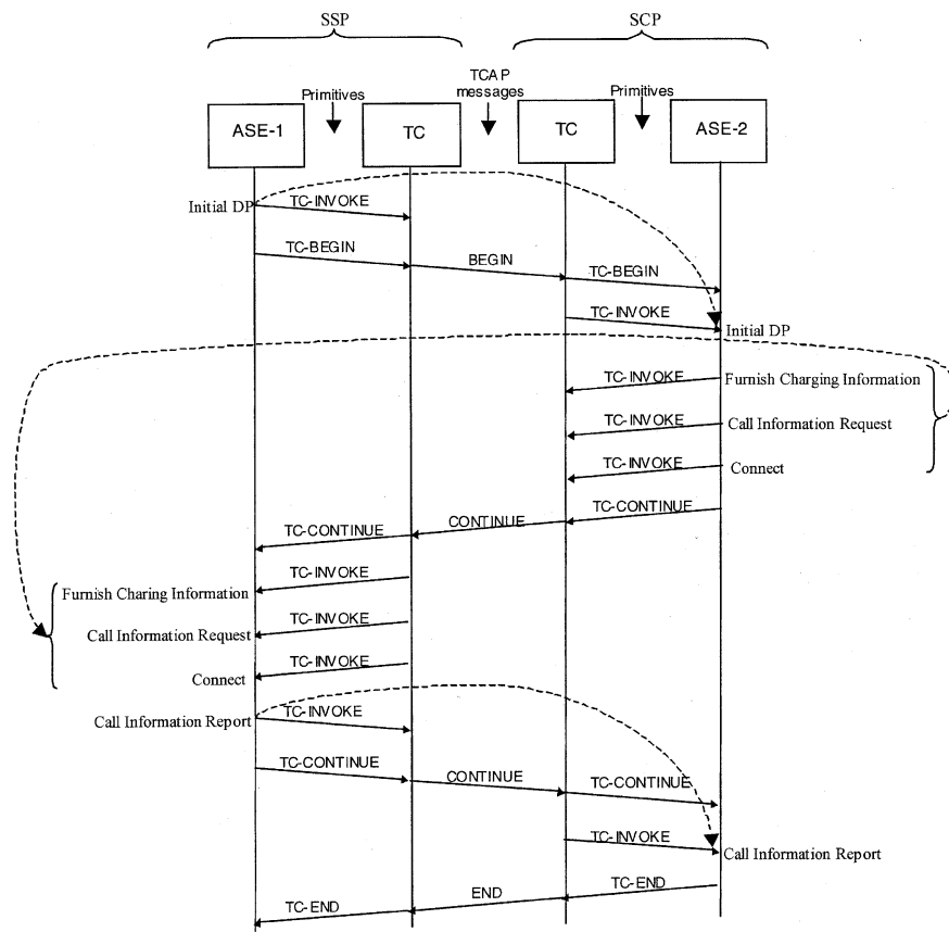
Figure 18.4-3 Example of INAP signaling exchange.
