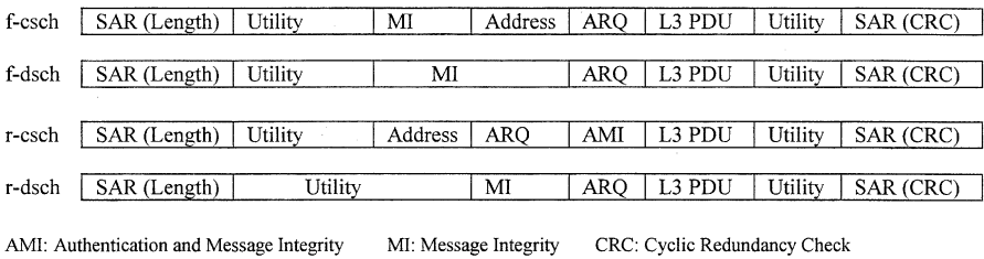
Figure 13.3-11. LAC PDU structure before SAR segmentation.
