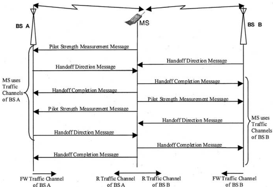
Figure 13.2-6. Call flow example of a soft handoff.
