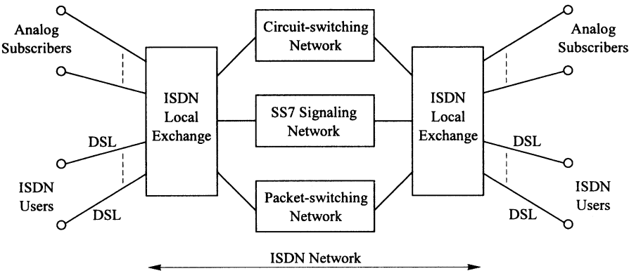
Figure 10.1-2. ISDN network.
