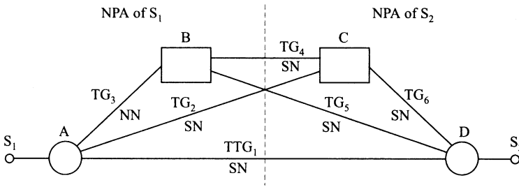
Figure 1.2-1. Called numbers. SN, subscriber number; NN, national number.
