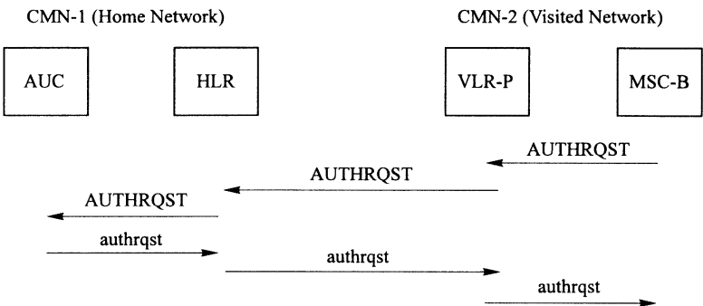
Figure 19.2-2. Authentication of a mobile. (From TSB-51. Reproduced with permission of TIA.)
