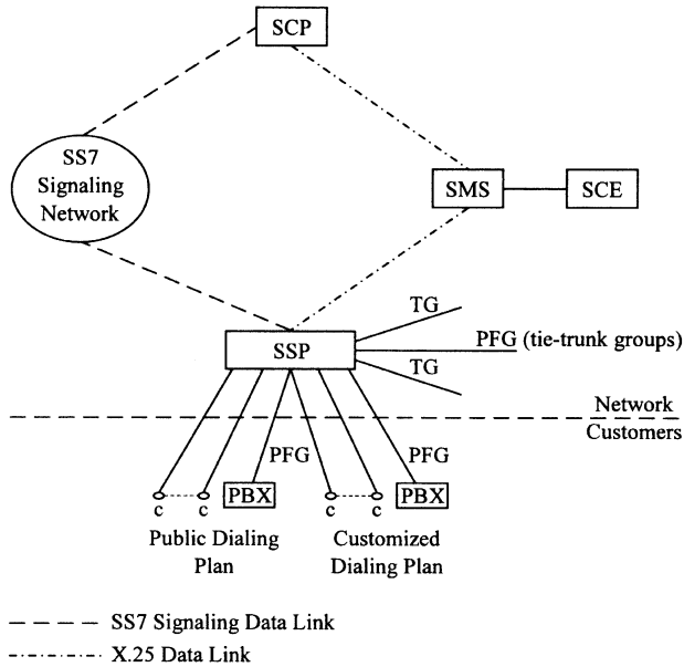
Figure 17.1-1. AIN 0.1 architecture.
