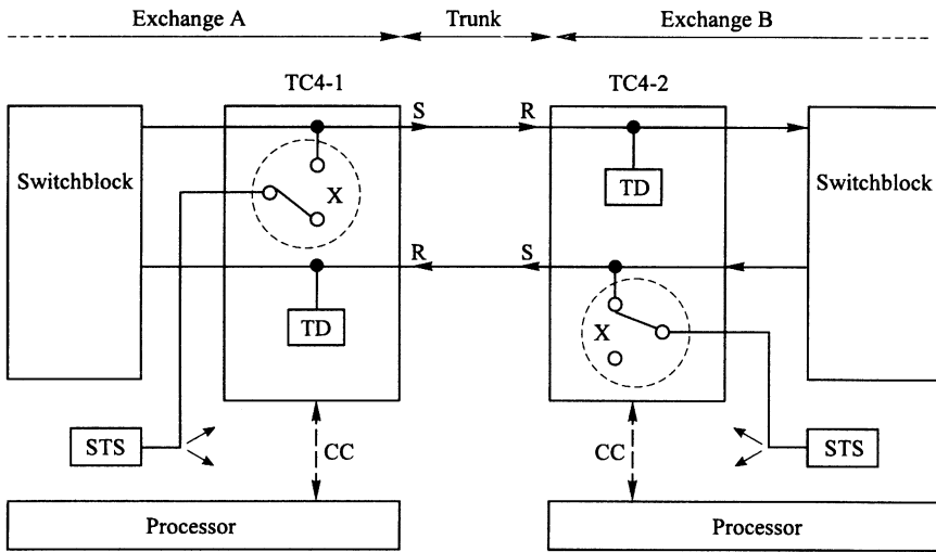
Figure 4.2-2. Four-wire analog trunk circuits (TC4).
