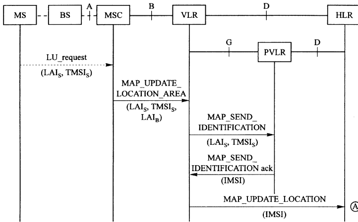
Figure 19.7-3. Initial operations for location area updating. Mobile is not known at VLR and is identified by LAI S and TMSI S . (From GSM.09.02-Version 4.9.0. Courtesy of ETSI.)
