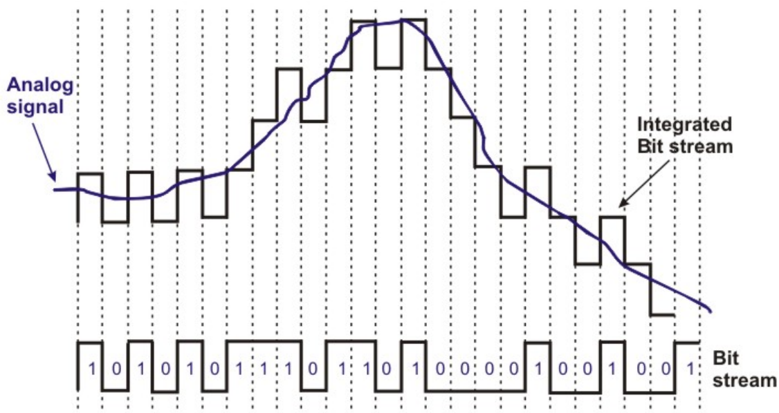
Figure 2.4.20 Delta modulation
