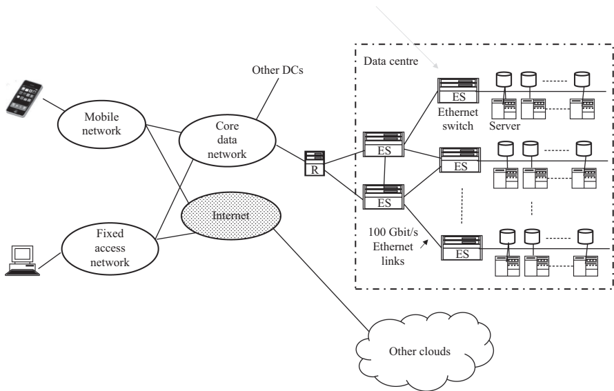
Figure 8.30 Cloud and DC, as provided by a Telco
