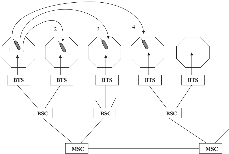
Figure 9.12 GSM handover
