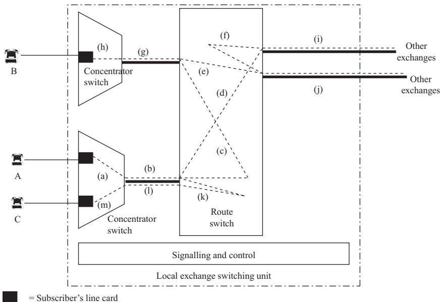
Figure 6.2 Generalised local exchange (folded)
