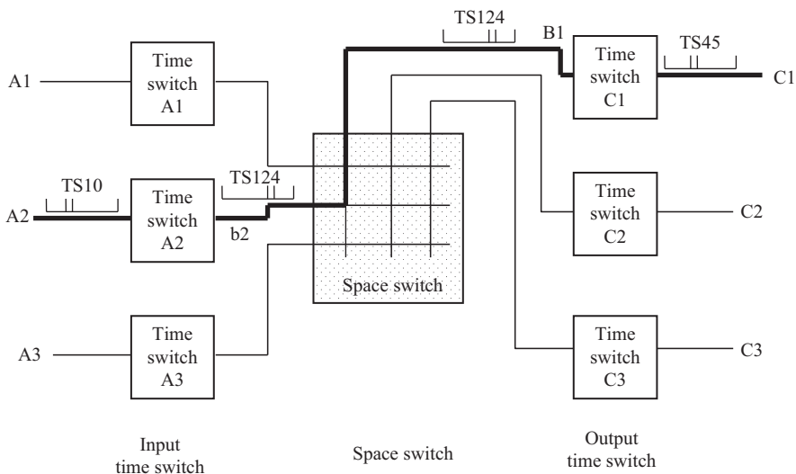
Figure 6.9 T-S-T switch-block
