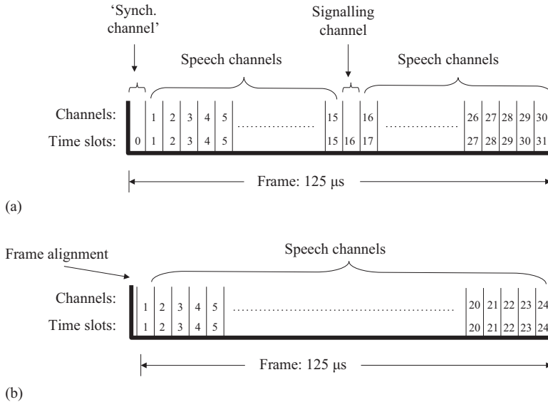
Figure 6.3 Summary of PCM frame formats. (a) 30-channel international standard. (b) 24-channel North American standard
