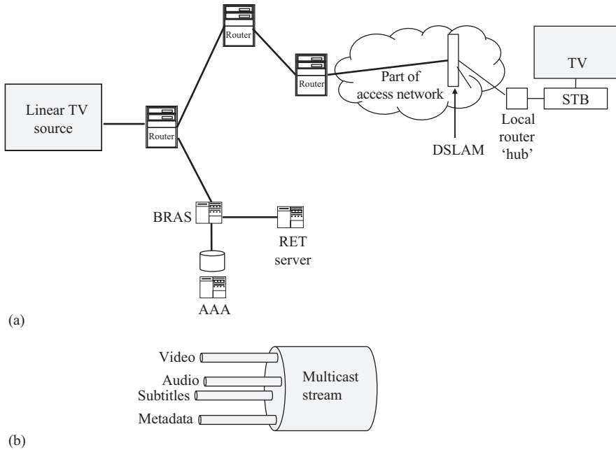
Figure 8.28 Linear TV multicast delivery. (a) Linear TV distribution networking. (b) Multicast stream assembly
