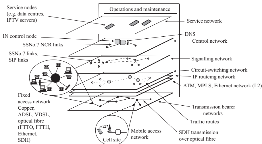
Figure 11.4 The multilayer view of a set of telecommunication networks
