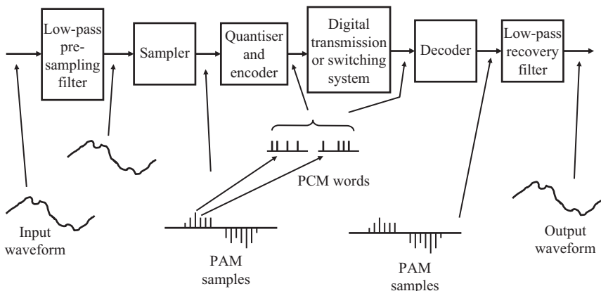
Figure 3.17 The pulse-code modulation process
