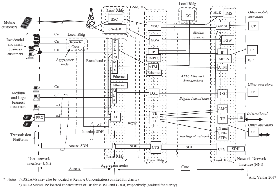
Figure 11.5 Typical set of Telco networks
