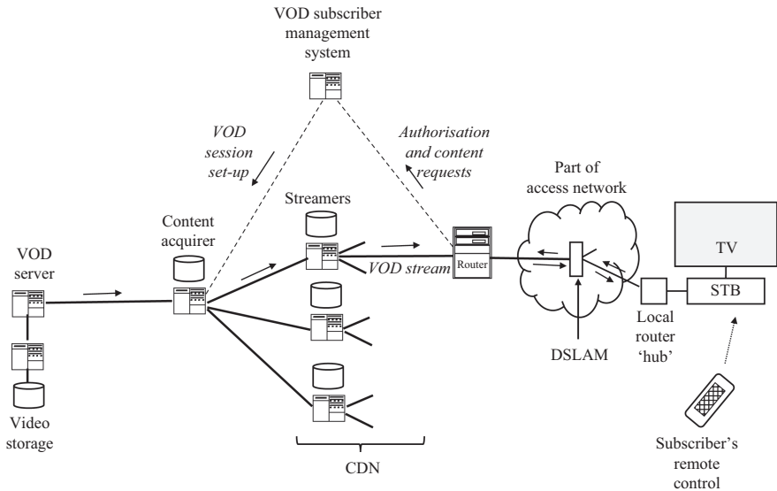
Figure 8.27 Video on demand delivery using content-distribution network
