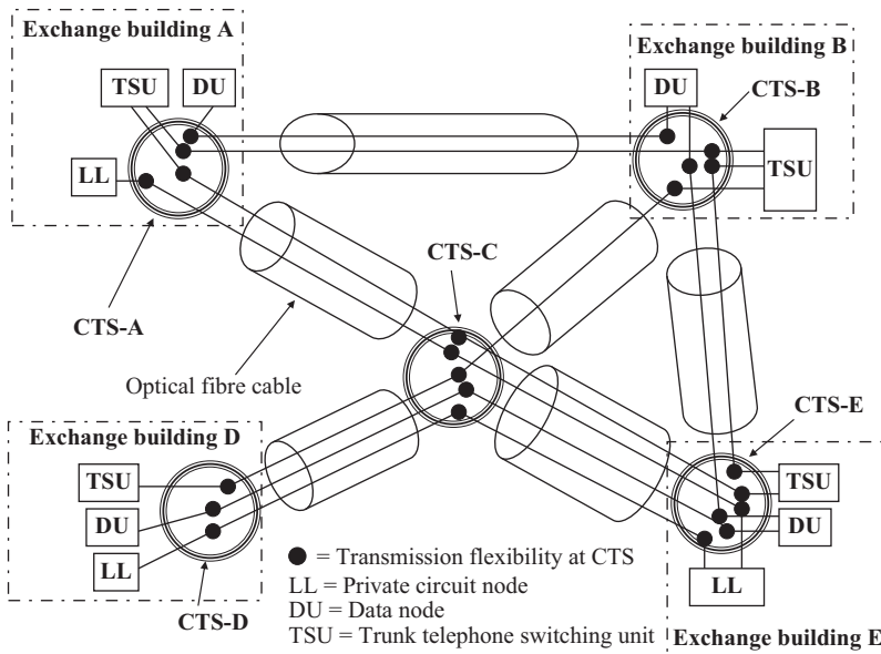
Figure 5.8 Transmission network configuration
