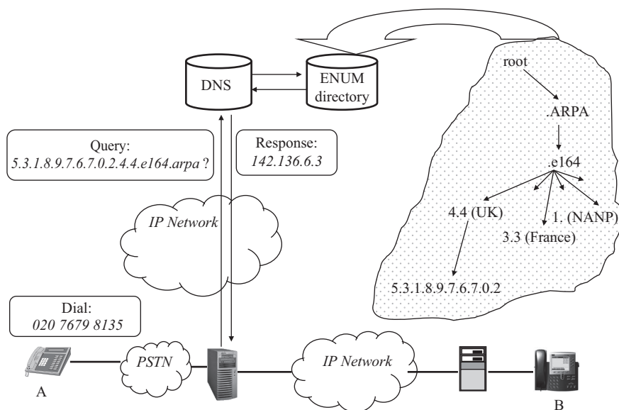
Figure 10.17 Use of ENUM system
