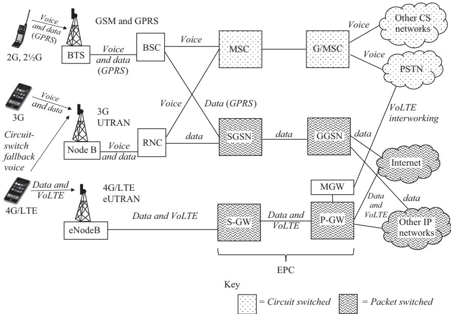
Figure 9.25 The routing of voice calls in multigeneration set of mobile networks
