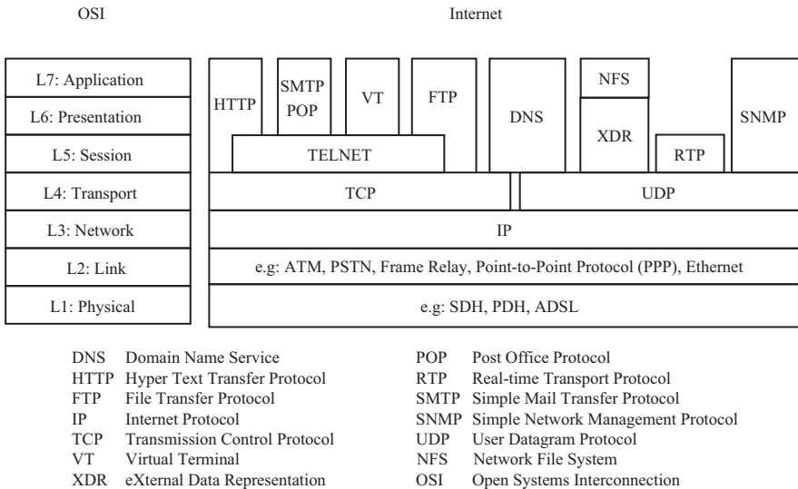
Figure 8.14 The Internet and OSI protocol reference models
