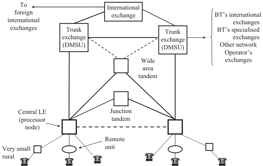
Figure 1.10 British Telecommunication's public switched telephone network
