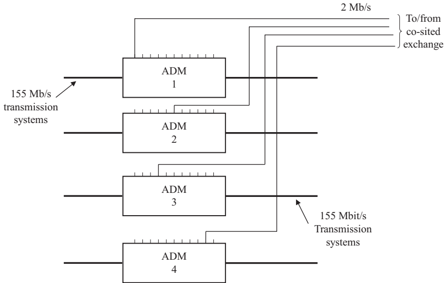
Figure 5.11 SDH core transmission network station – using ADMs
