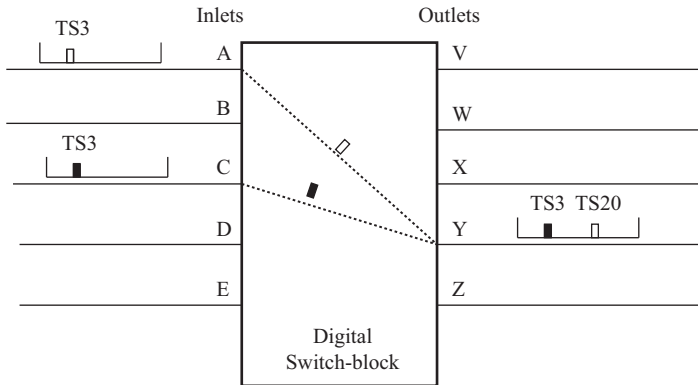
Figure 6.6 Digital switch-blocks
