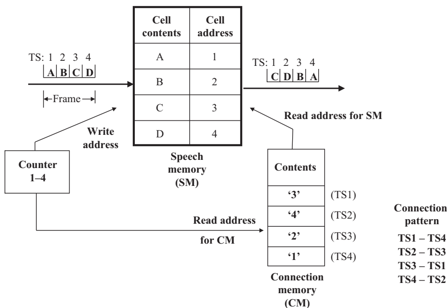
Figure 6.7 The principle of time switching using storage
