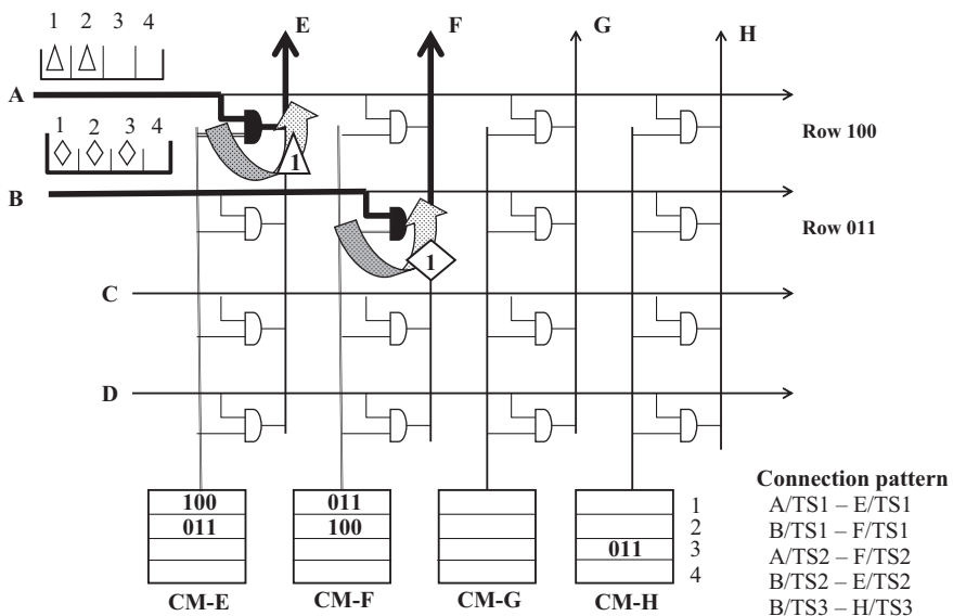
Figure 6.8 Digital space switching
