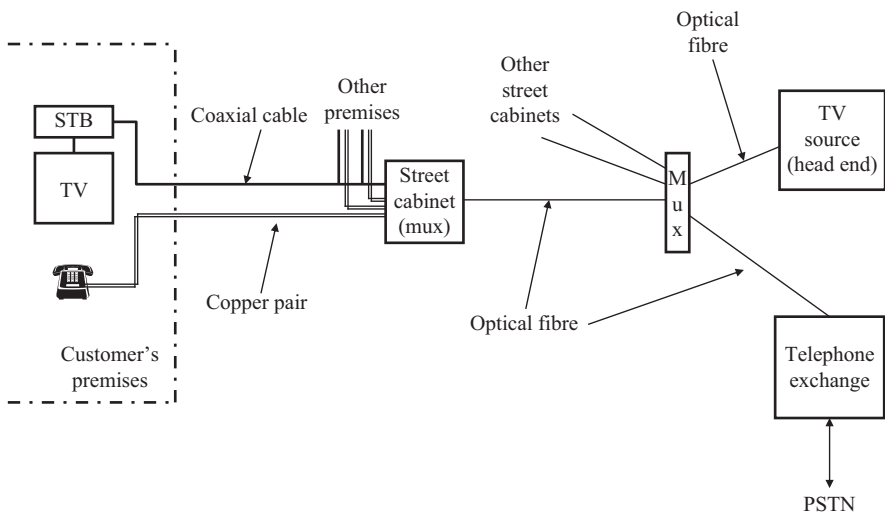
Figure 2.2 Cable TV network
