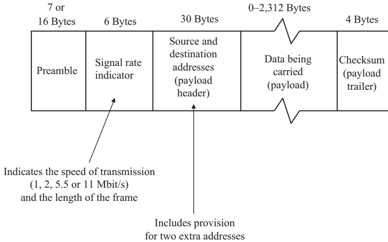
Figure 8.26 A simplified illustration of the frame format of IEEE 802.11 wireless LAN
