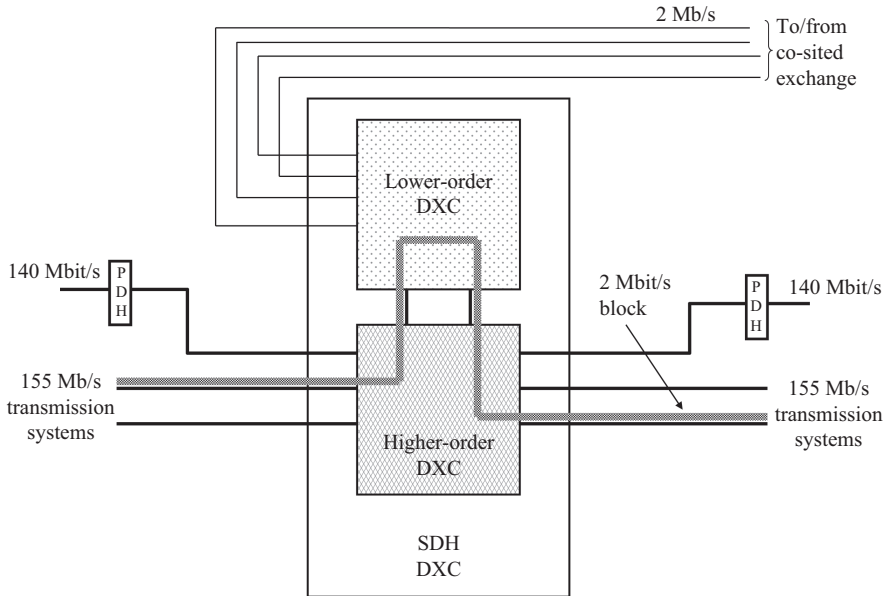
Figure 5.10 SDH core transmission station – using DXCs
