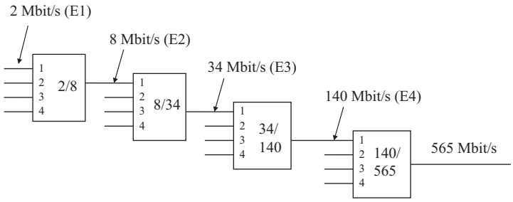
Figure 4.12 Plesiochronous digital hierarchy European standard
