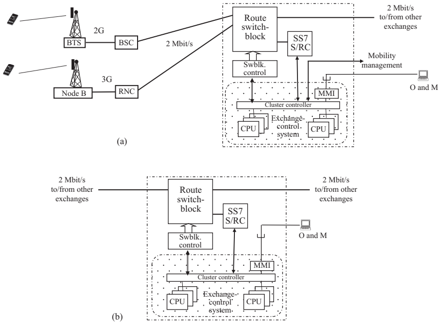
Figure 7.11 Exchange-control systems in other types of circuit-switched exchanges. (a) Mobile exchange (MSC). (b) Trunk, junction tandem or international exchange
