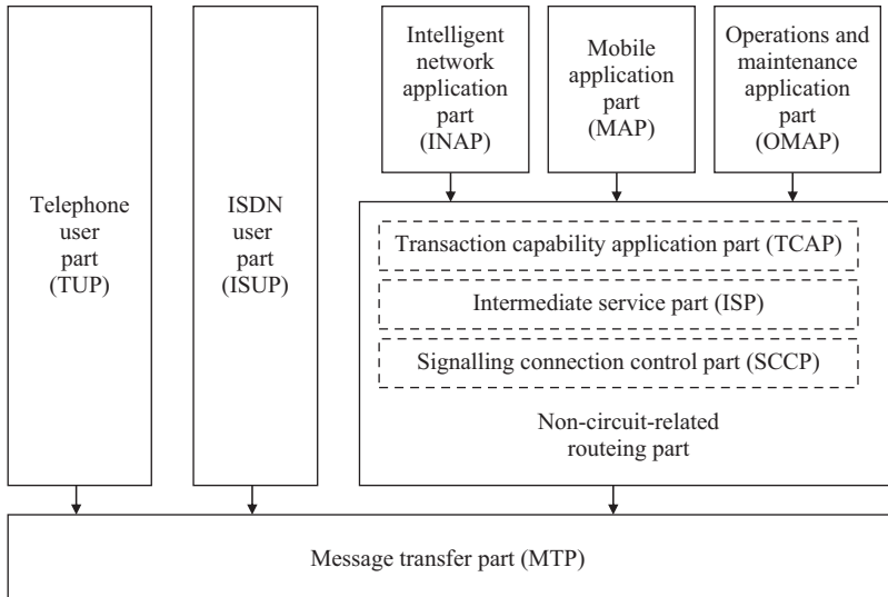
Figure 7.8 Simplified architectural view of SS7
