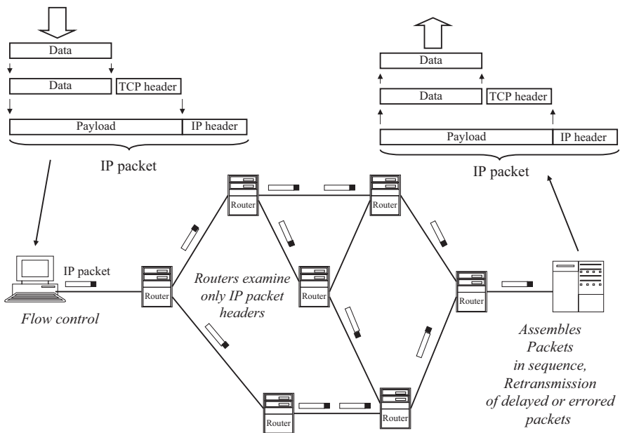
Figure 8.12 Transmission control protocol
