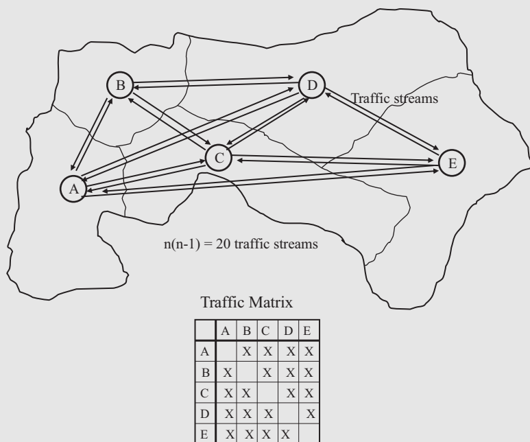
Figure 6.24 Planning example; Stage 3; Traffic distribution [Ward]
