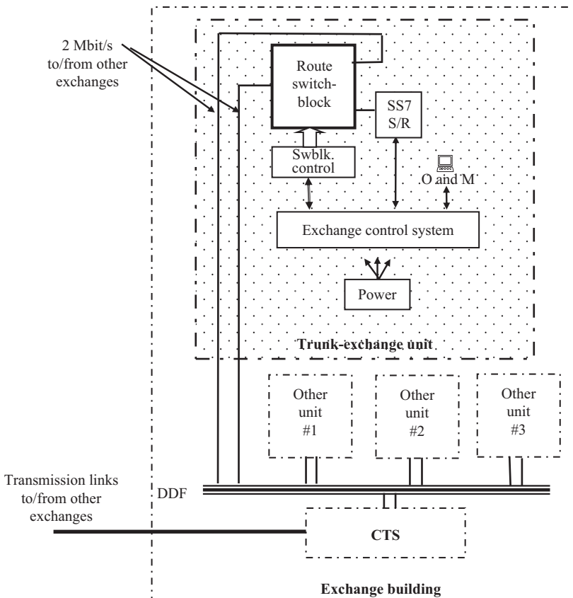
Figure 6.14 Trunk-exchange structure within a typical operational exchange building
