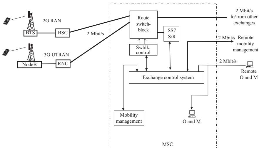
Figure 6.13 Structure of a mobile switching centre
