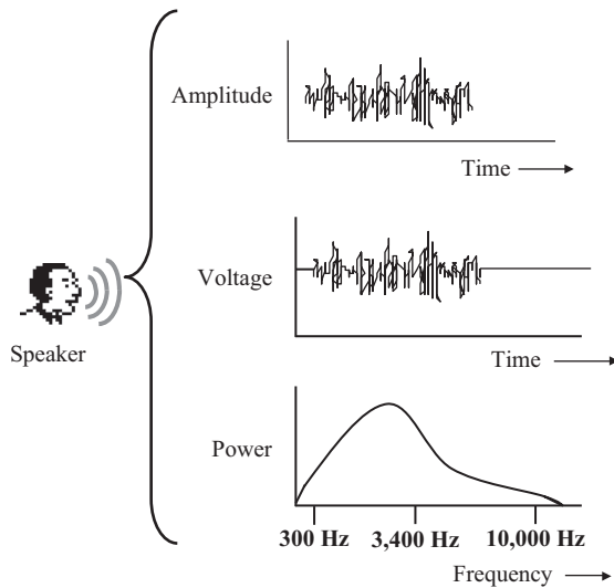
Figure 3.6 Waveform analysis of speech
