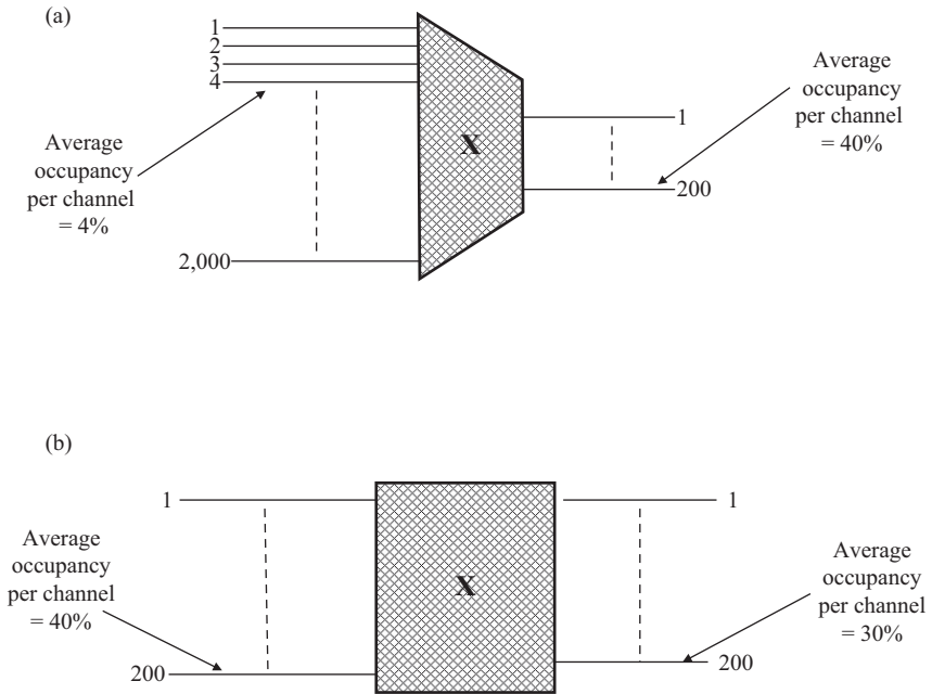
Figure 3.2 (a) Concentration switching. (b) Route switching
