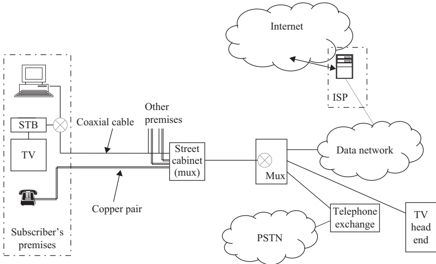
Figure 2.9 Access to the Internet via cable modem
