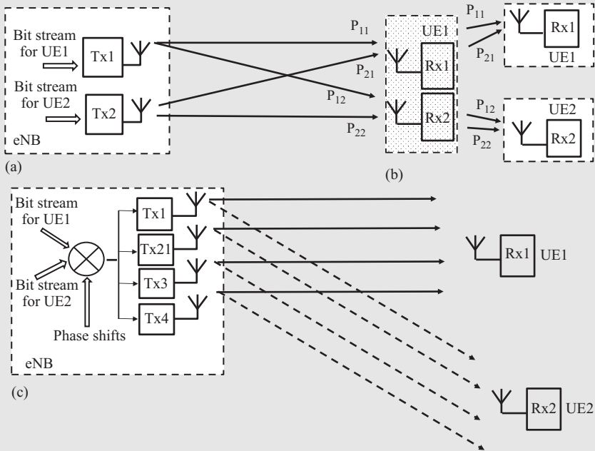
Figure 9.19 MIMO and beam steering. (a) Spatial multiplexing, (b) downlink MU-MIMO, and (c) beam steering
