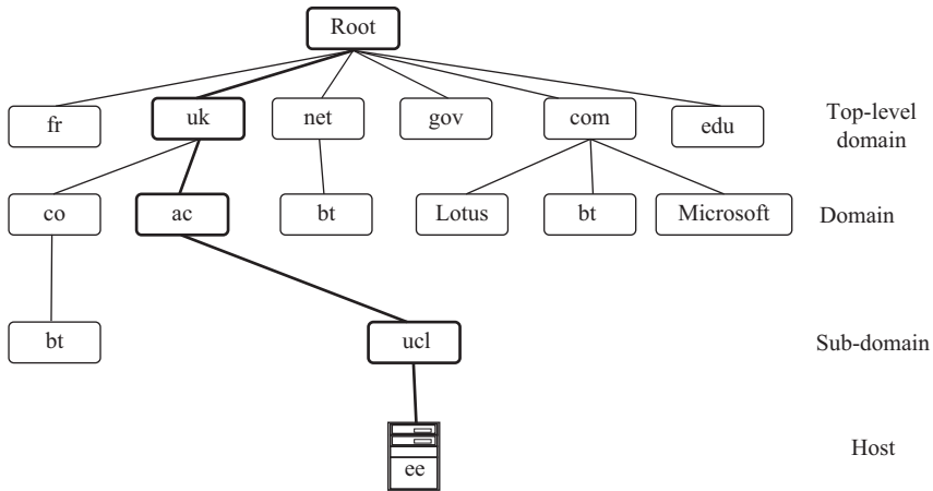
Figure 10.12 Internet domain-name system hierarchy, for example, 'ee.ucl.ac.uk'
