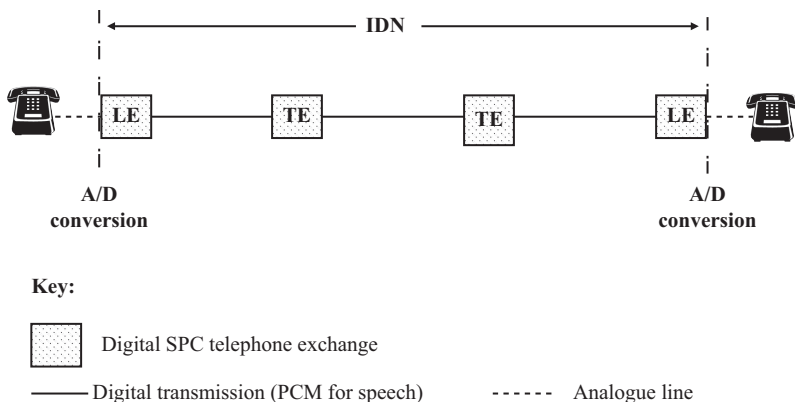
Figure 3.15 Integrated digital network
