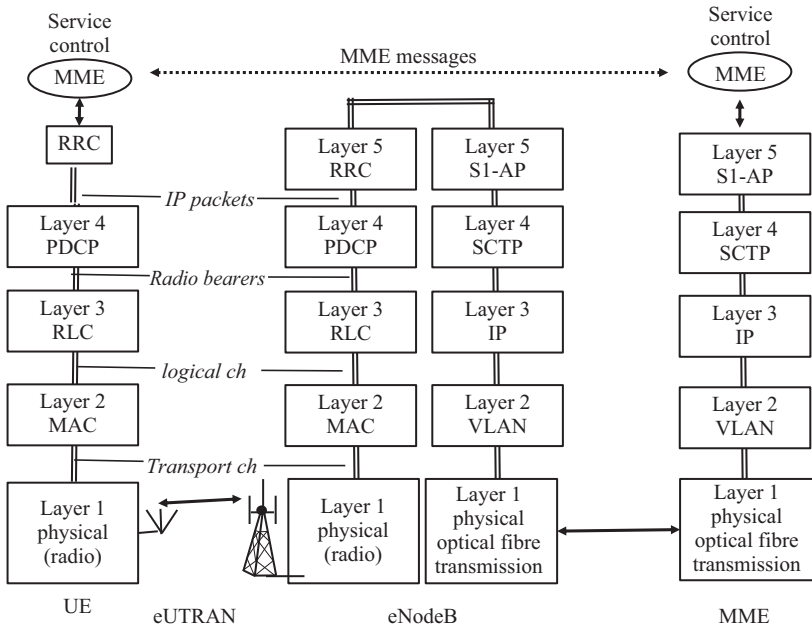
Figure 9.23 The protocol stack for the control plane within LTE
