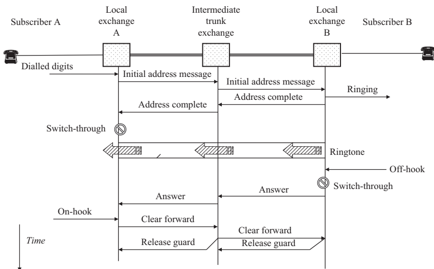
Figure 7.4 A typical telephone call sequence
