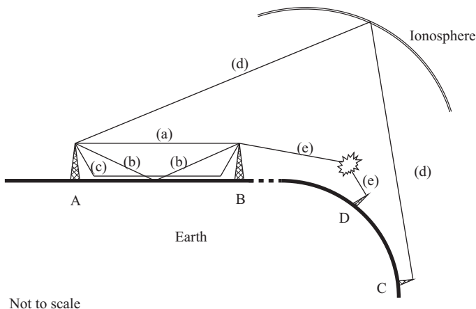
Figure 4.6 Different types of radio paths
