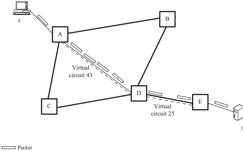
Figure 8.2 Connection-orientated packet switching
