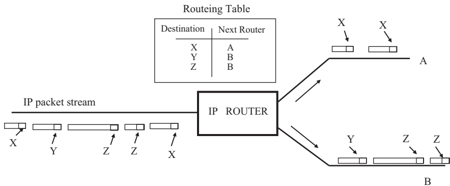
Figure 8.10 IP packet routing
