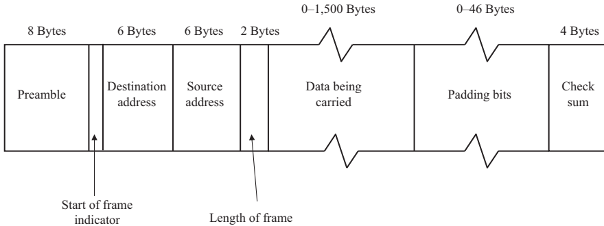
Figure 8.24 Ethernet LAN frame format
