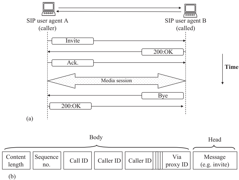
Figure 7.9 The SIP concept. (a) SIP message sequence. (b) SIP message format
