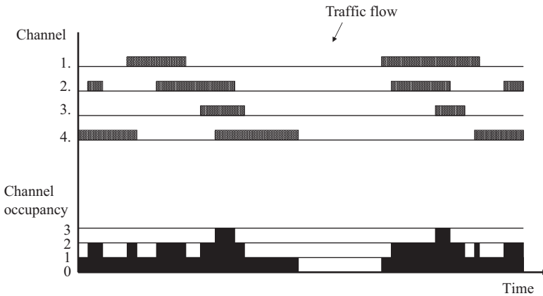
Figure 6.16 Traffic and occupancy
