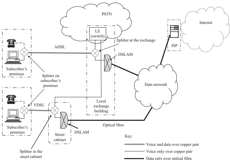
Figure 2.8 Access to the Internet via ADSL and VDSL
