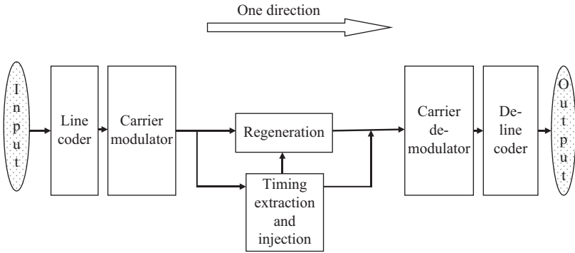
Figure 4.3 Digital line transmission system
