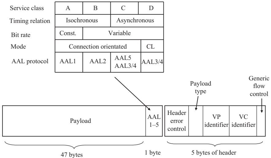
Figure 8.7 ATM service classes, AAL and cell structure
