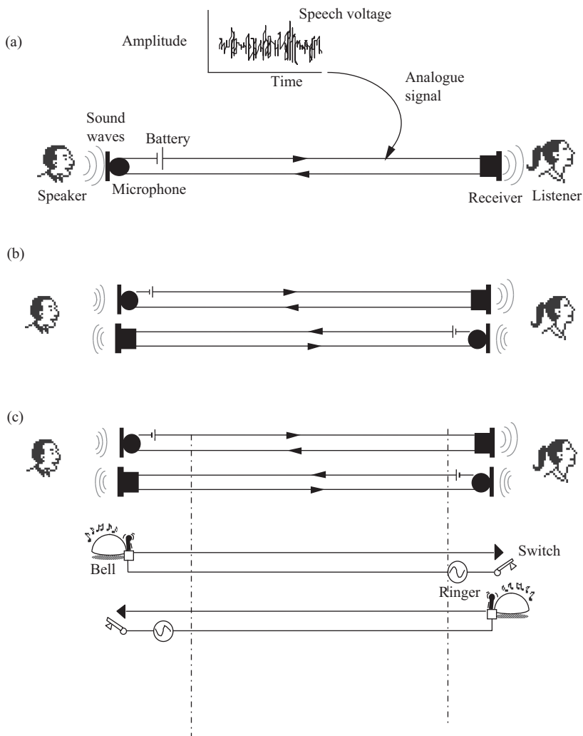
Figure 1.1 (a) Simple one-way speech over two wires. (b) Both-way speech over four wires. (c) Both-way speech and alerting over eight wires. [Ward]
