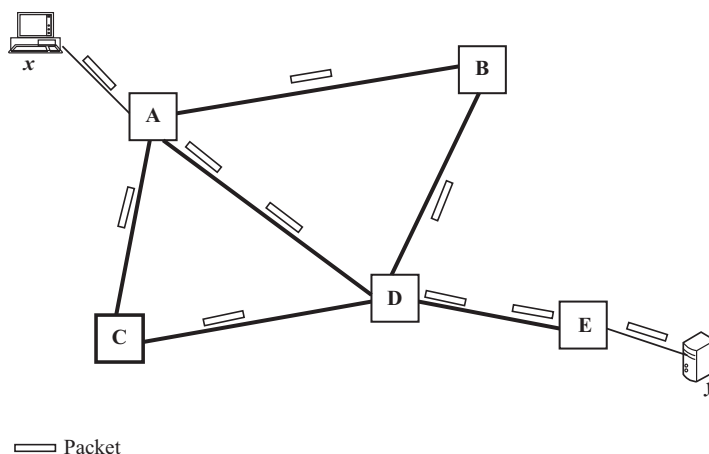
Figure 8.3 Connectionless packet switching
