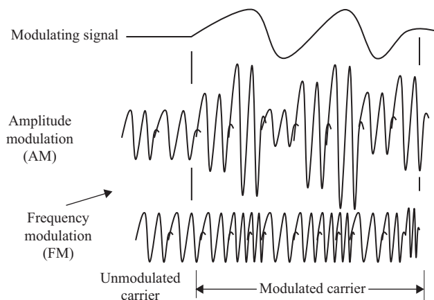
Figure 4.1 Carrier-wave modulation
