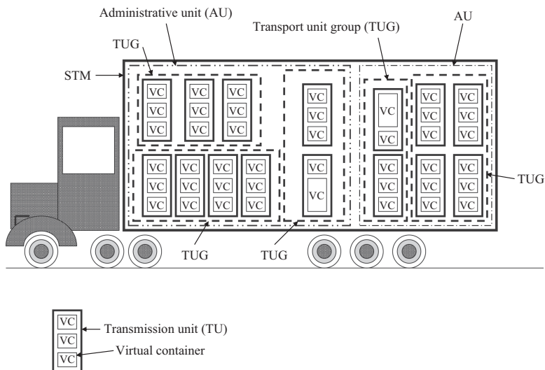
Figure 4.18 SDH/SONET concept
