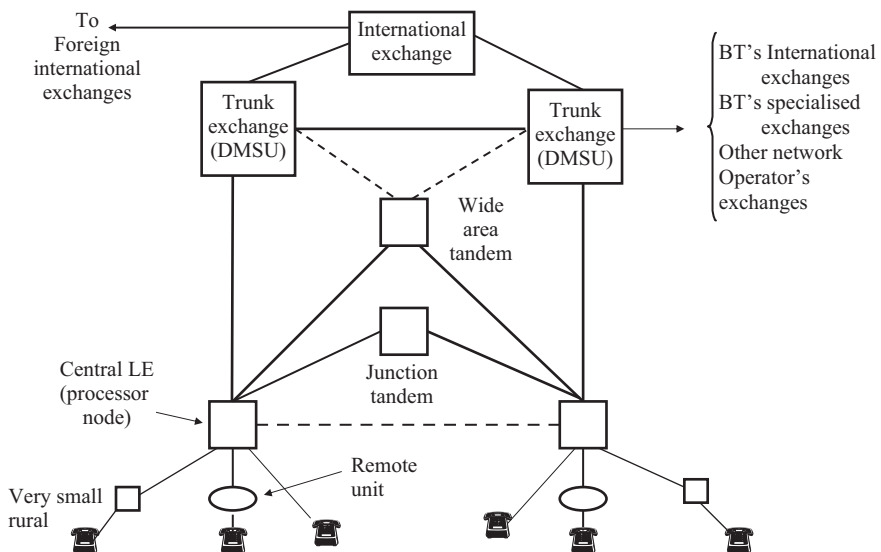
Figure 6.18 BT's public switched telephone network
