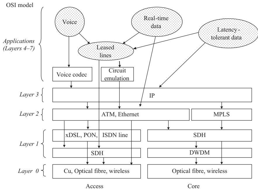
Figure 11.16 Generalised logical architecture for NGN
