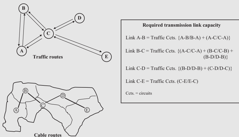
Figure 6.28 Planning example; Stage 7; Transmission (engineering route) dimensioning [Ward]
