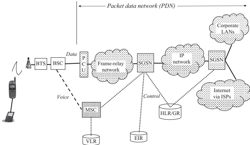
Figure 9.15 GPRS outline
