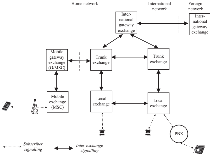
Figure 7.1 The domains of signalling
