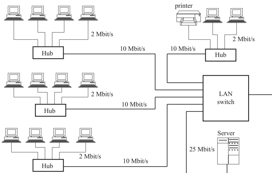
Figure 8.23 Local area network concept
