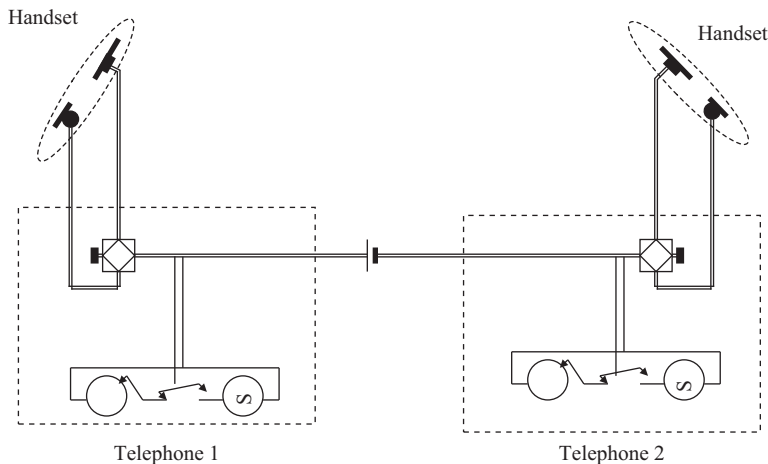
Figure 1.4 A simple two-phone system
