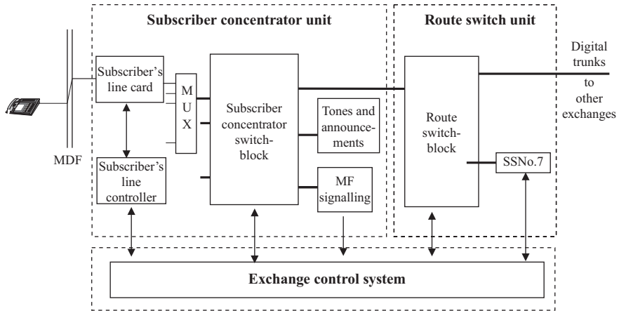
Figure 6.4 SPC digital exchange: functional overview
