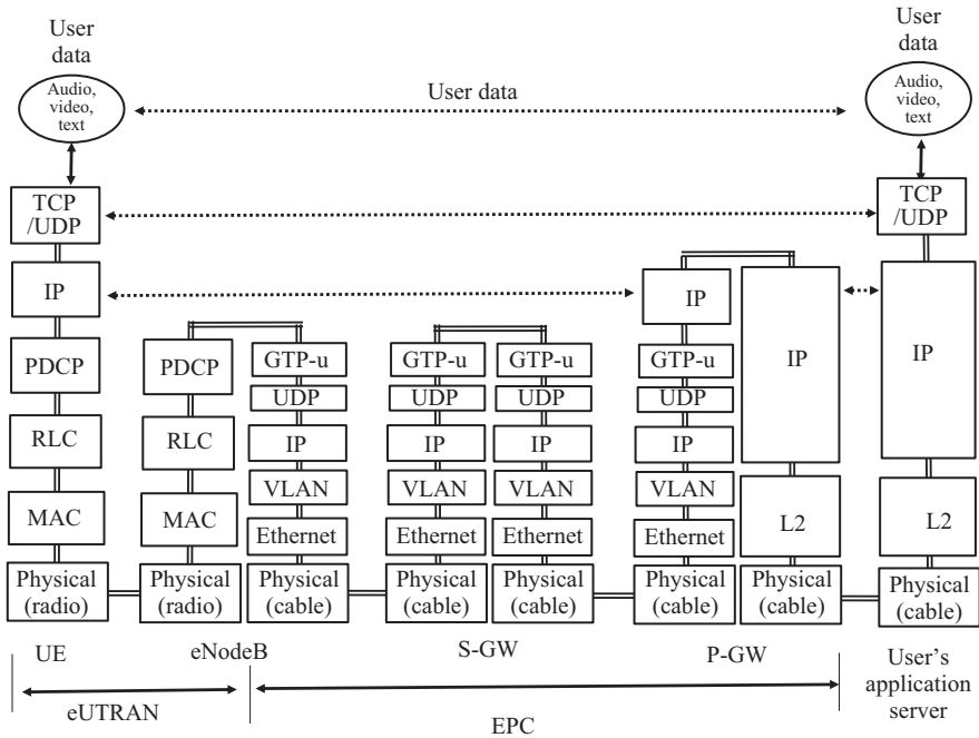
Figure 9.24 The protocol stack for the data plane within LTE
