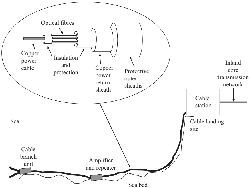
Figure 4.26 Submarine optical fibre cable system
