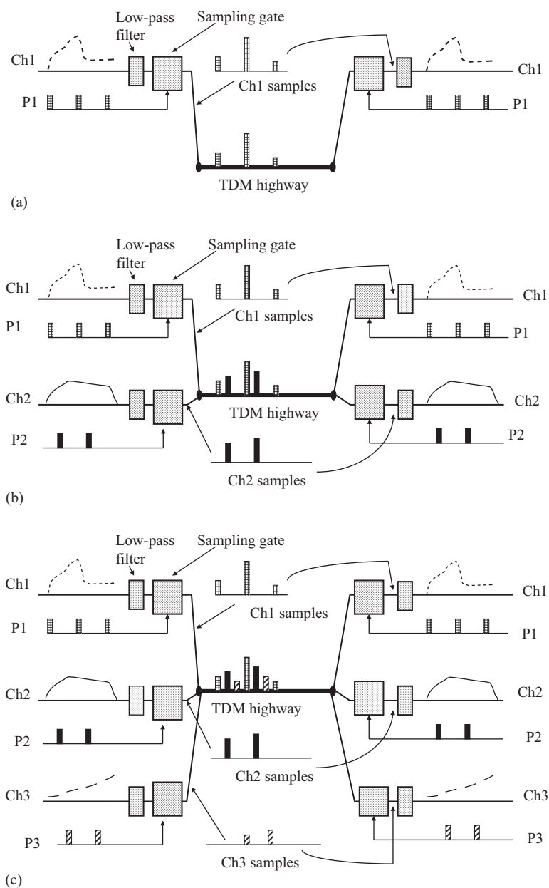
Figure 3.9 Principle of a time-division multiplexing system
