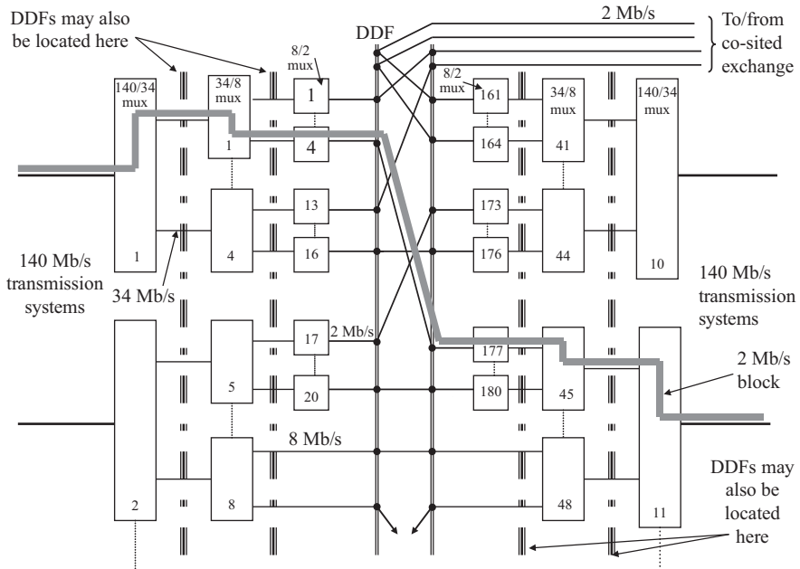
Figure 5.9 PDH transmission network station
