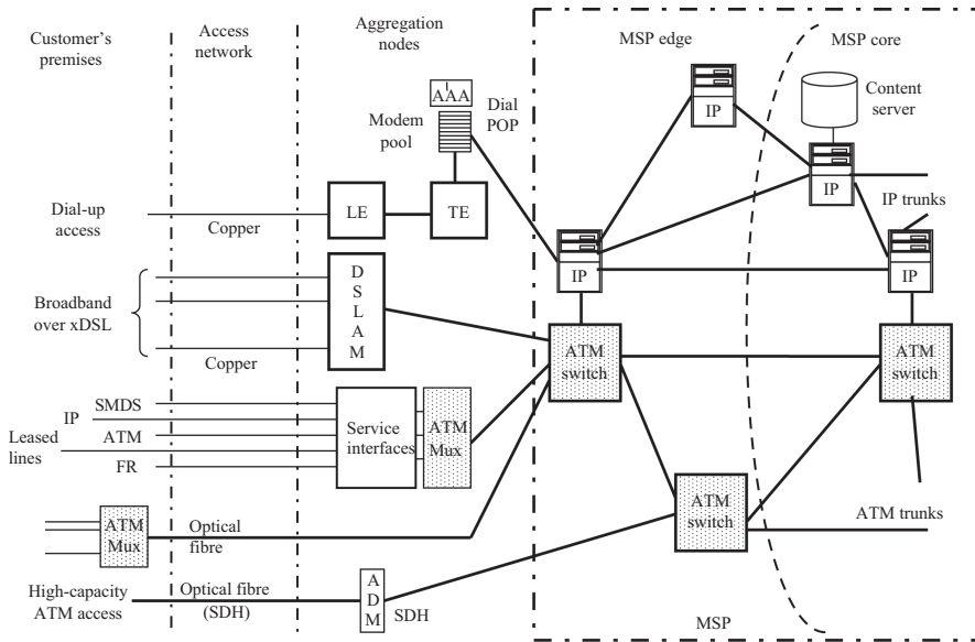
Figure 8.20 Multiservice platform
