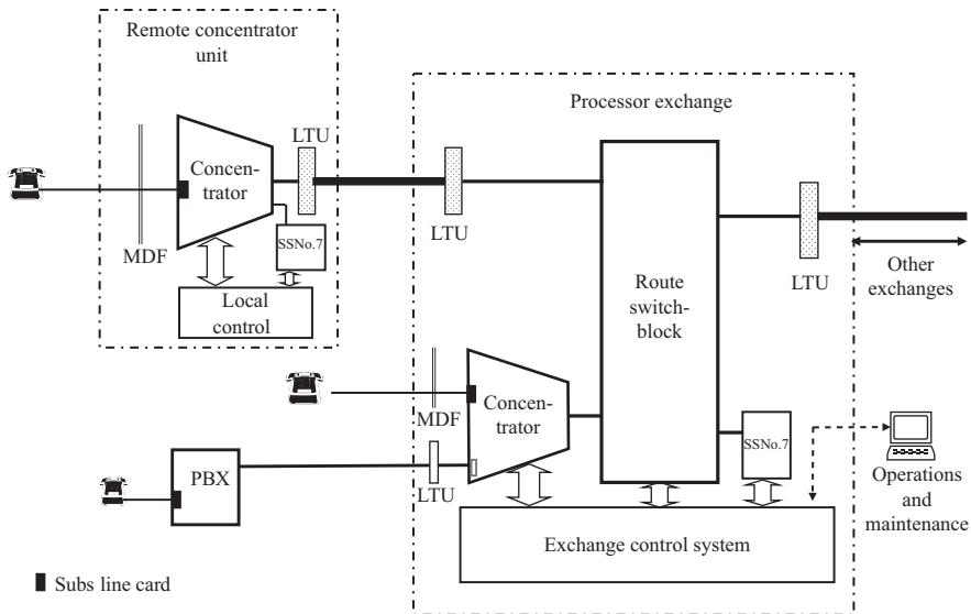
Figure 6.11 Local exchange structure with remote concentrator units
