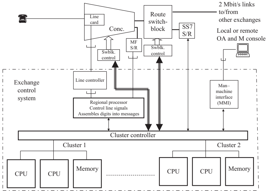
Figure 7.10 Exchange-control system in a local exchange
