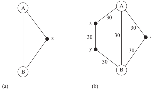
Figure 5.14 Transmission-path resilience: diverse routing. (a) Physical diversity of two. (b) Physical diversity of three
