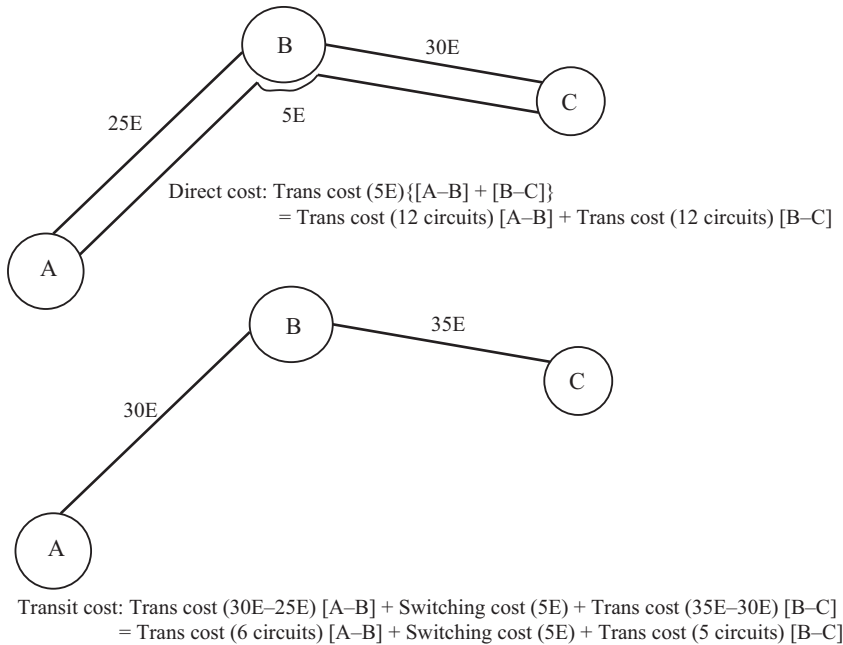
Figure 6.19 Example of direct versus tandem routing comparison
