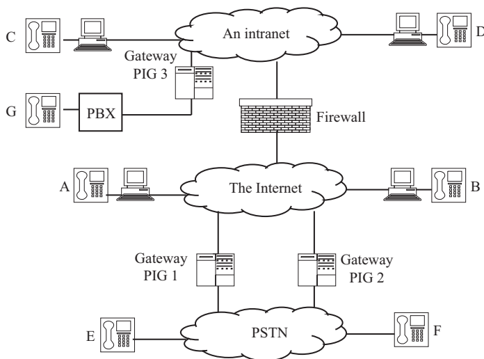
Figure 8.16 Voice-over-IP scenarios
