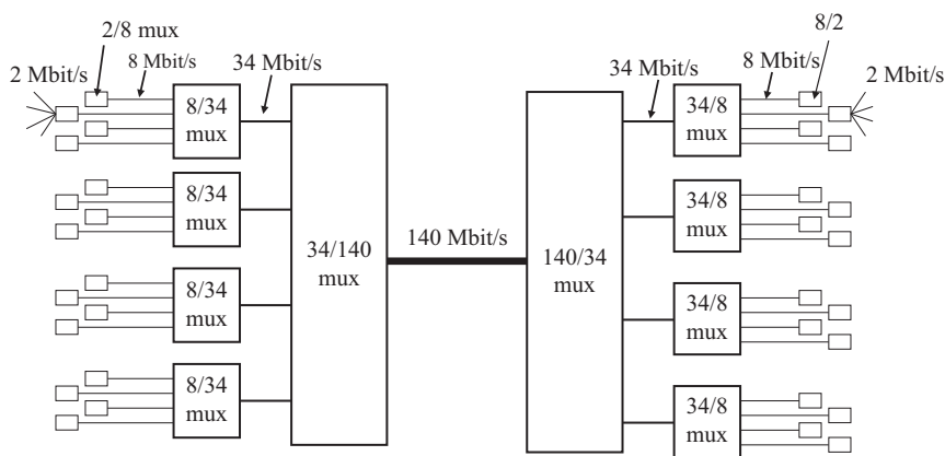
Figure 4.14 A 140 Mbit/s PDH line multiplexed system
