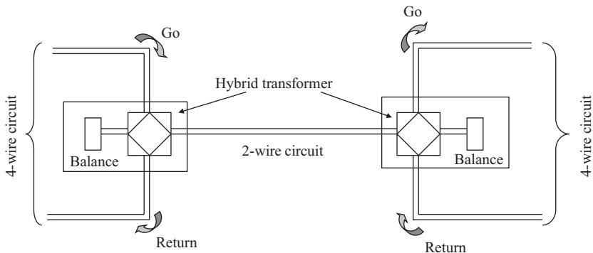
Figure 1.3 The 4-to-2 wire conversion
