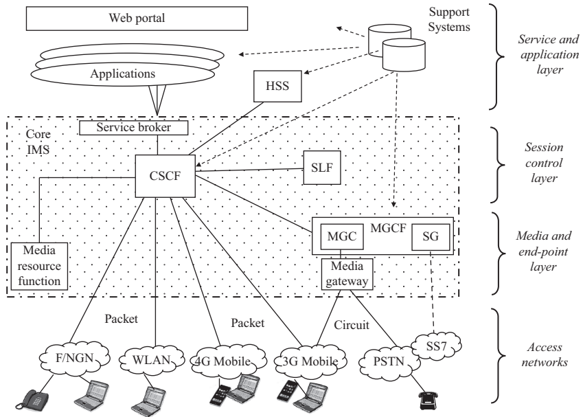
Figure 7.15 IP multimedia subsystem
