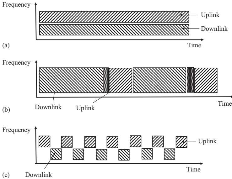
Figure 9.21 Categories of duplex working in the eUTRAN of the LTE system. (a) Pure FDD, (b) pure TDD, and (c) mixed FDD and TDD (half duplex)
