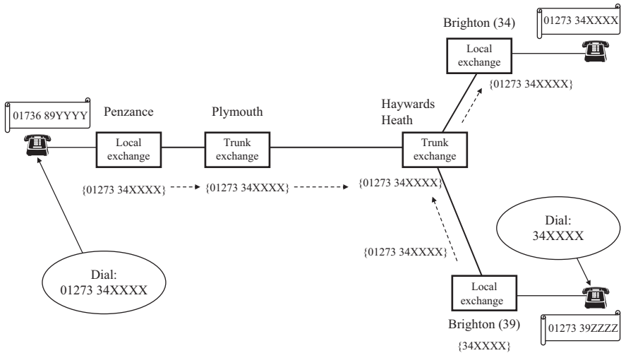
Figure 1.11 An example of a call routing
