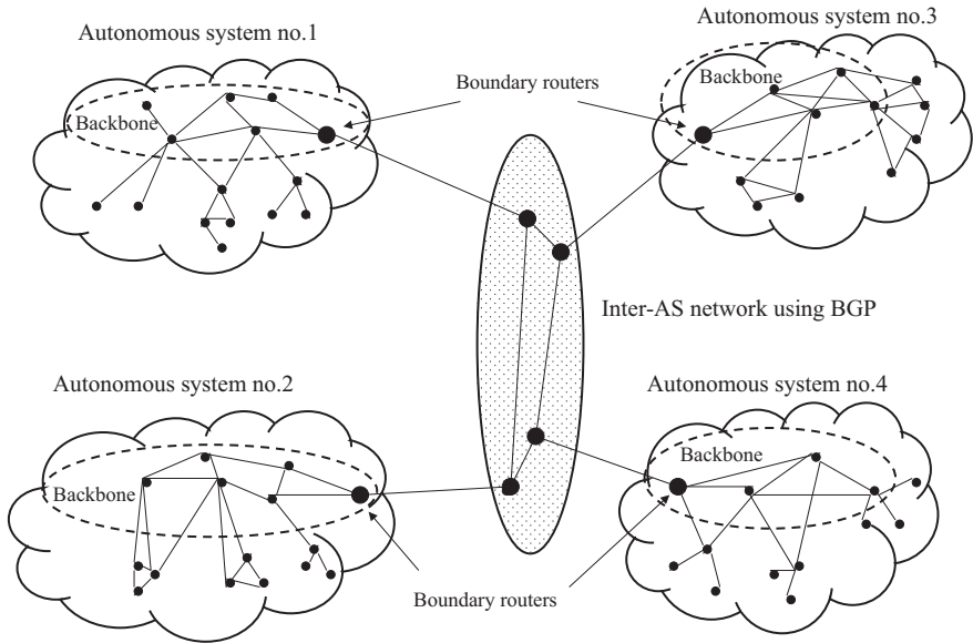
Figure 8.11 Autonomous IP systems
