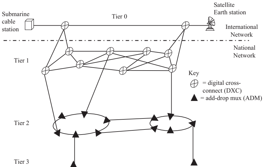
Figure 5.12 SDH transmission network structure
