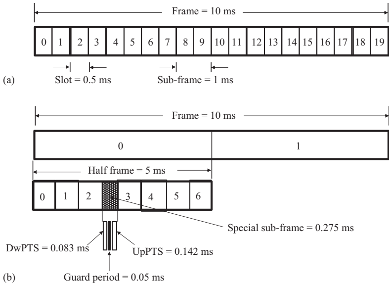
Figure 9.22 Frame structures for eUTRAN in LTE system. (a) Type 1 frame and (b) type 2 frame
