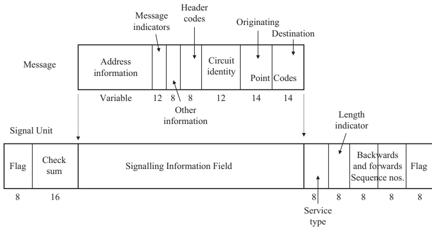
Figure 7.5 SS7 message and signal unit format
