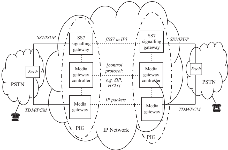
Figure 8.17 PSTN-to-IP Gateway (PIG)
