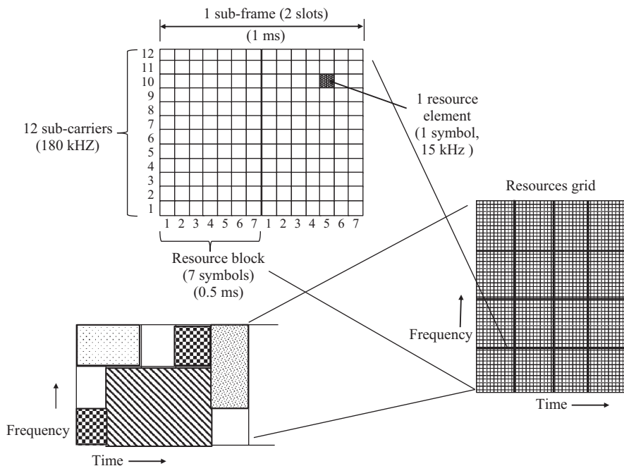
Figure 9.20 LTE resource elements and blocks
