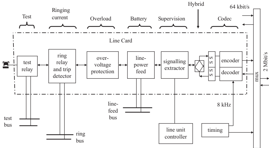
Figure 6.5 The components of a subscriber's line card
