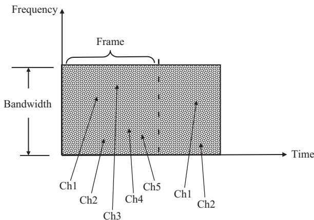
Figure 3.10 Code-division multiplexing
