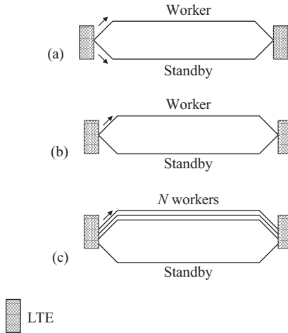
Figure 5.16 Transmission-media resilience: Use of spare links: (a) 1 + 1 protection, (b) 1:1 protection (automatic protection systems (APS)) and (c) 1:N protection (APS)
