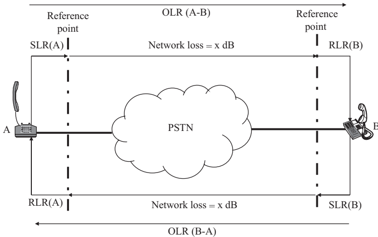
Figure 11.7 Transmission loss in the PSTN
