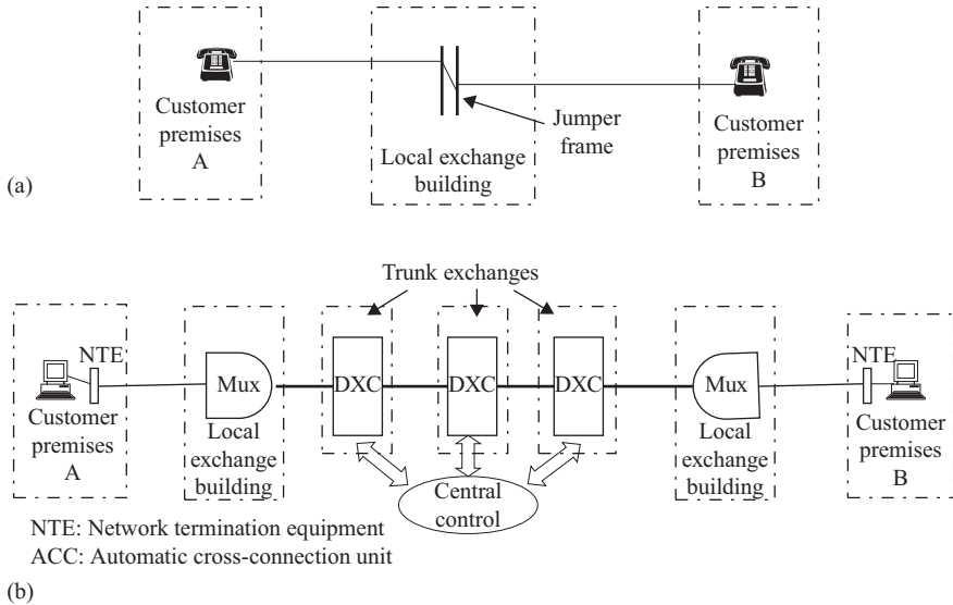
Figure 2.10 A leased-line services network. (a) Manually-jumpered leased-line circuit. (b) Leased-line circuit using digital cross-connection units
