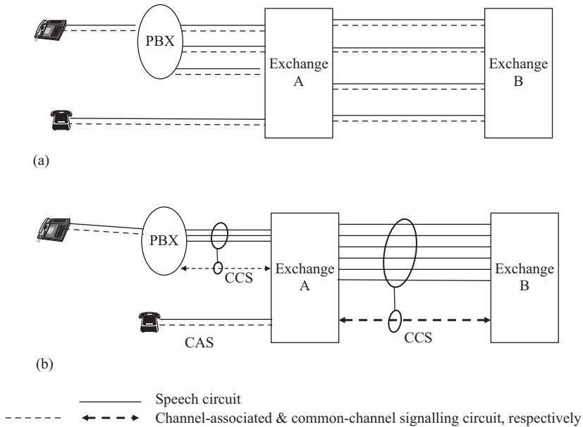
Figure 7.2 Relationships between voice channels and their signalling channels. (a) Channel-associated signalling (CAS). (b) Common-channel signalling (CCS)
