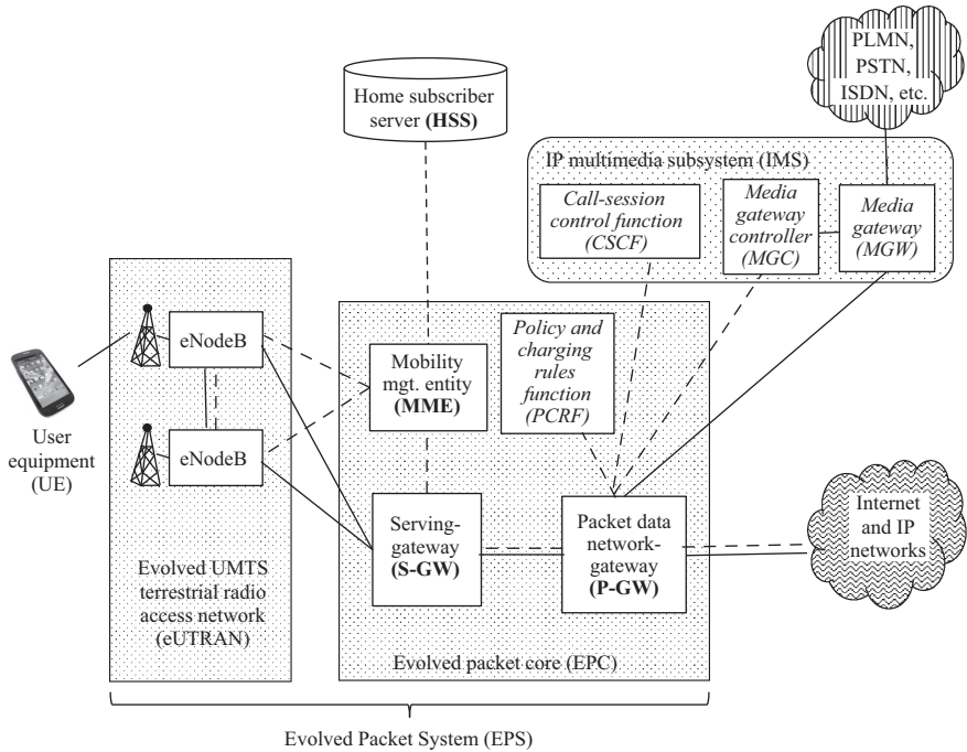
Figure 9.18 LTE system architecture
