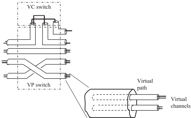
Figure 8.6 Virtual channels, virtual paths and switches
