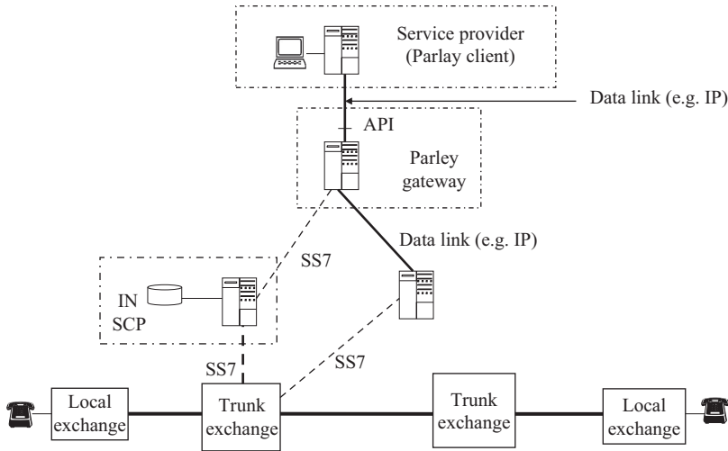
Figure 7.14 The Parlay concept
