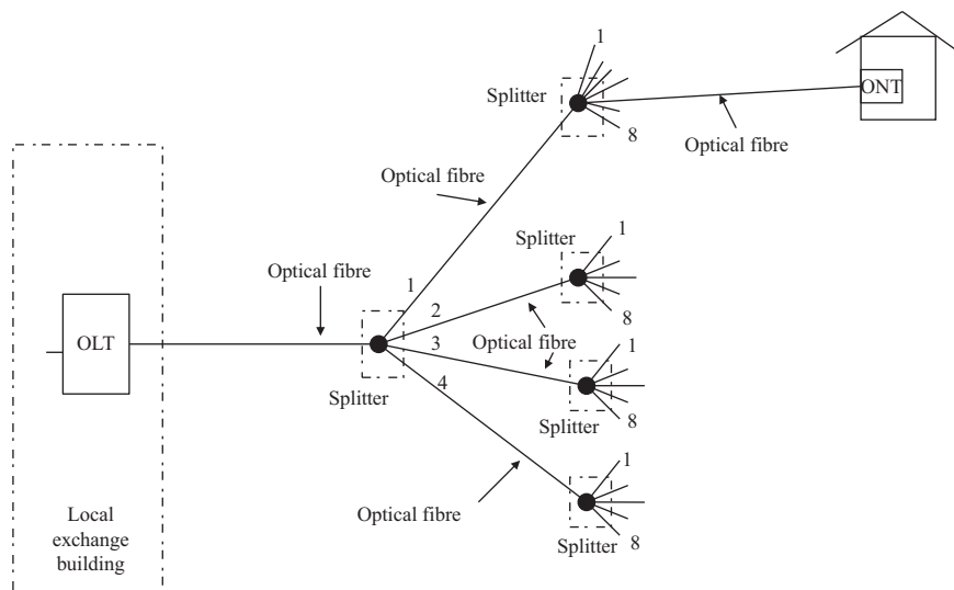
Figure 4.24 Passive optical fibre network
