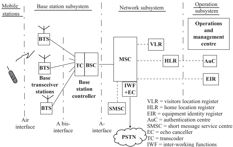
Figure 9.8 Architecture of the GSM network system
