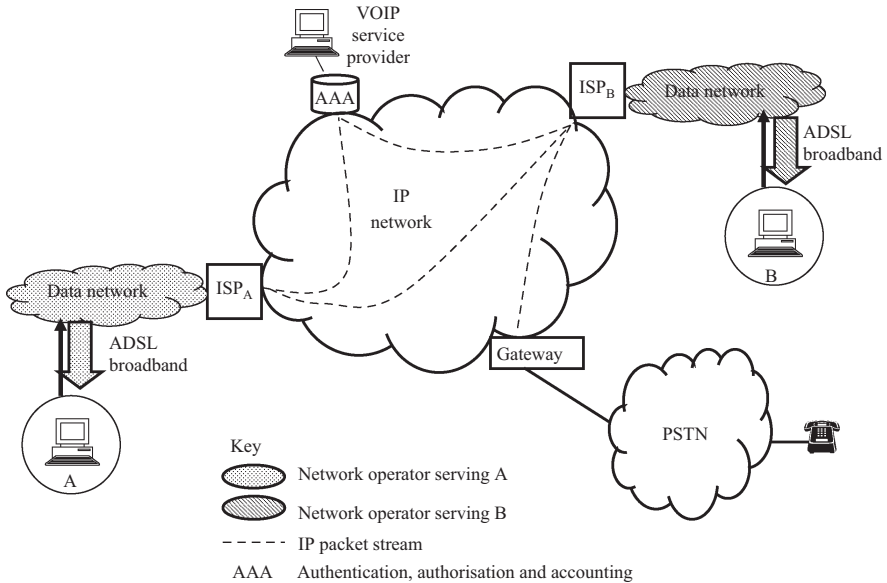
Figure 8.18 VoIP over broadband services
