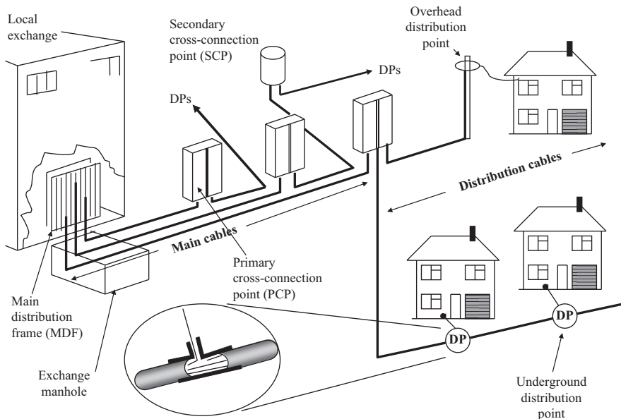
Figure 5.1 The physical architecture of a copper access network
