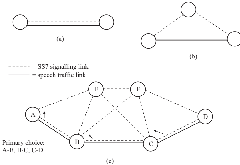
Figure 7.7 Modes of association of SS7 links with their traffic circuits. (a) Fully associated. (b) Quasi associated. (c) Alternative routing and non-associated working
