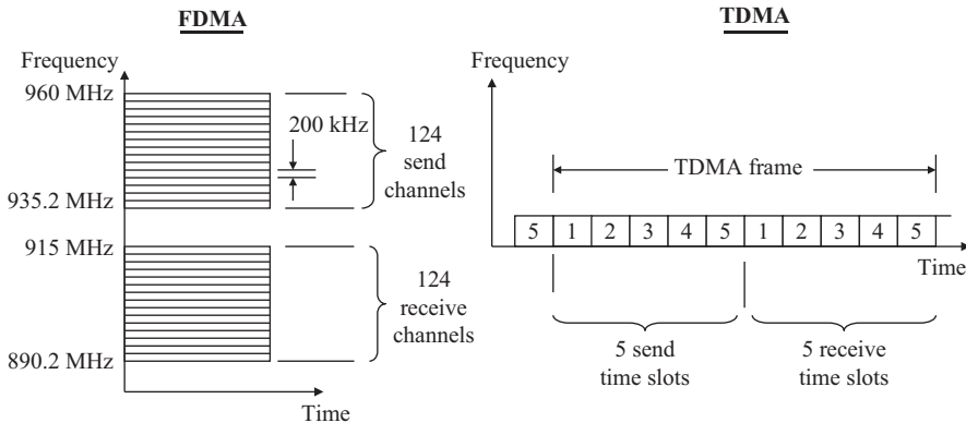
Figure 9.7 Multiple access and duplex arrangements for mobile networks
