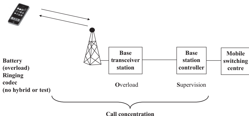
Figure 9.6 BORSCHT functions in a mobile system
