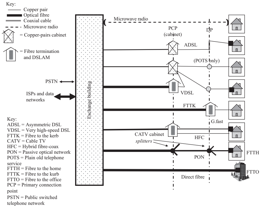
Figure 5.5 Broadband options for the access network
