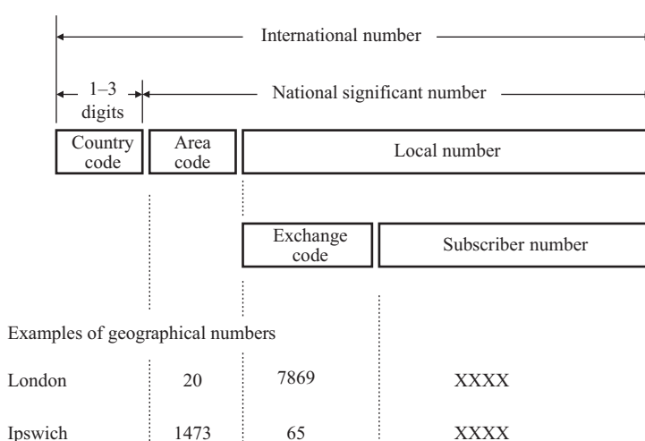
Figure 10.2 Standard format for geographical numbers (E164)
