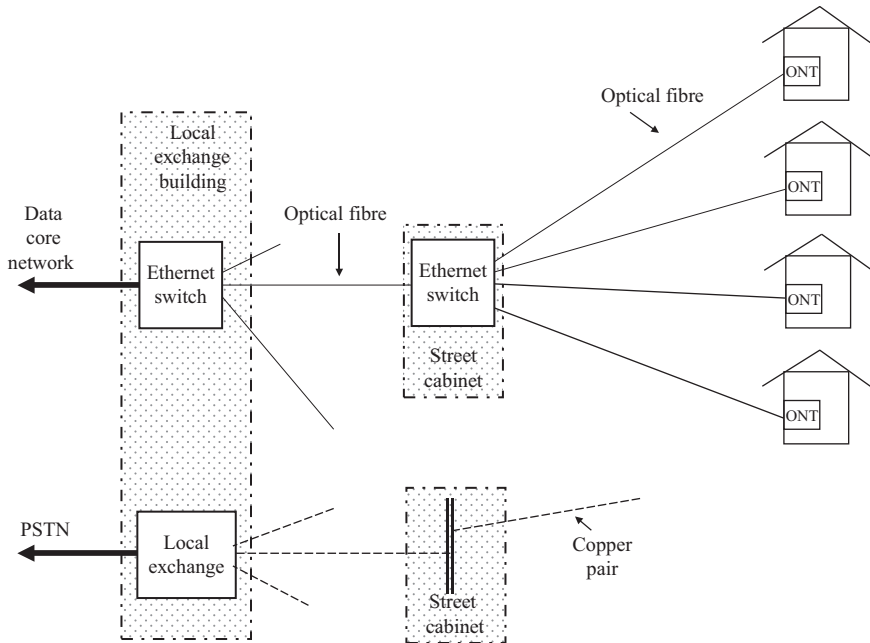
Figure 4.25 Ethernet fibre to the premises (home)
