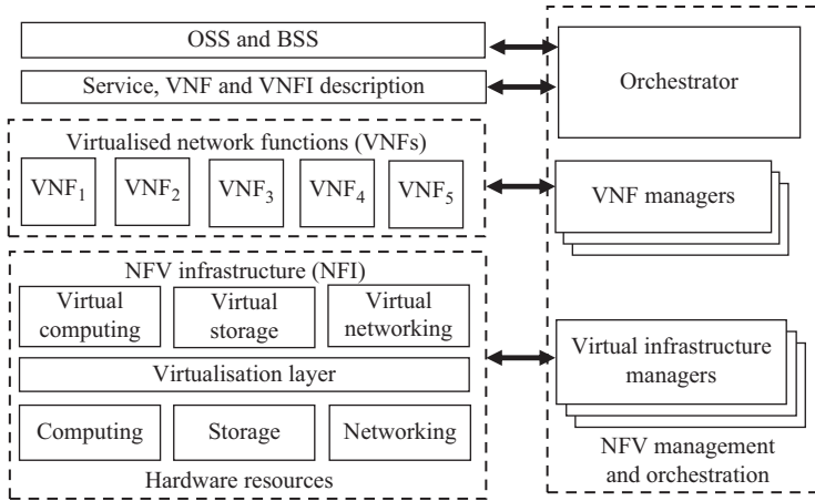
Figure 8.31 ETSI's NFV general architectural model
