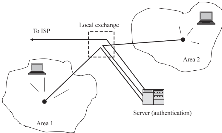
Figure 5.3 Wireless LAN access network
