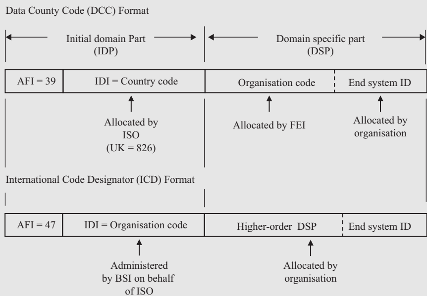
Figure 10.11 ISO NSAP ATM addressing formats
