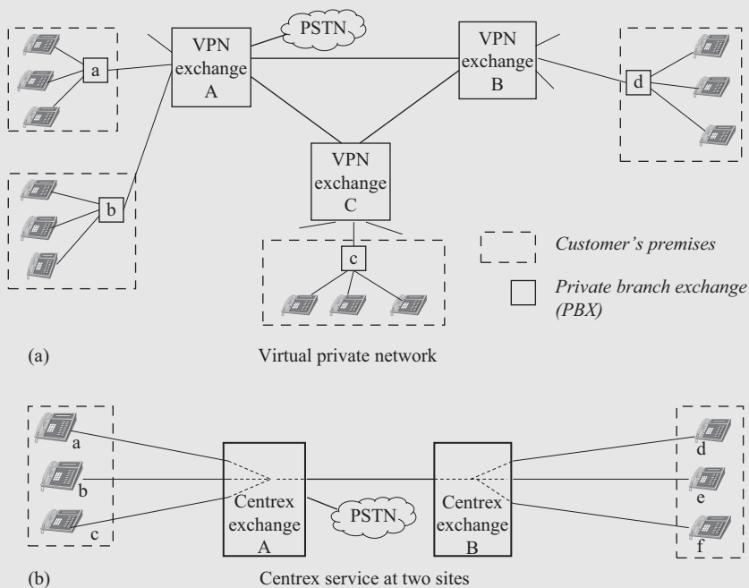
Figure 2.12 Centrex private network and VPN
