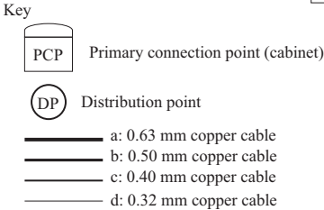
Figure 5.2 Typical local loop make-up
