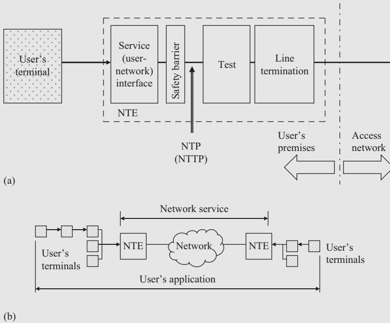
Figure 5.6 Network termination. (a) The network terminating equipment functions. (b) The extent of network service
