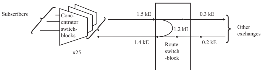
Figure 6.17 Exchange dimensioning
