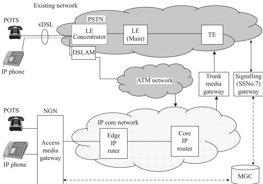
Figure 11.15 Generic fixed NGN architecture for voice calls
