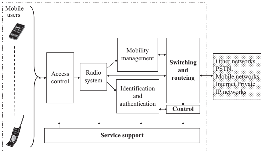
Figure 9.1 A simplified generic mobile system
