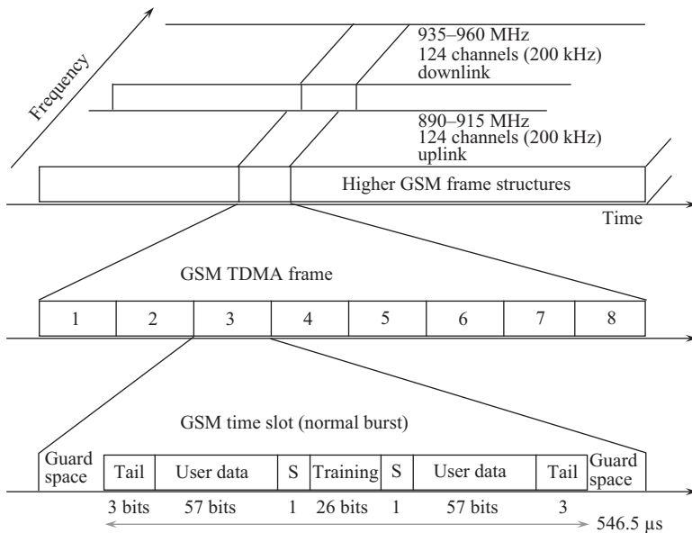
Figure 9.13 The GSM frame structure
