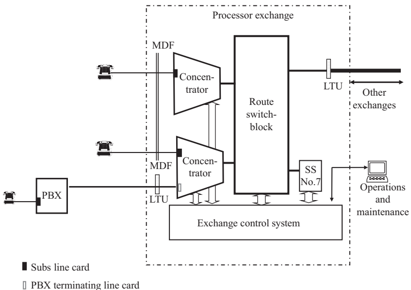
Figure 6.10 Local exchange unit structure
