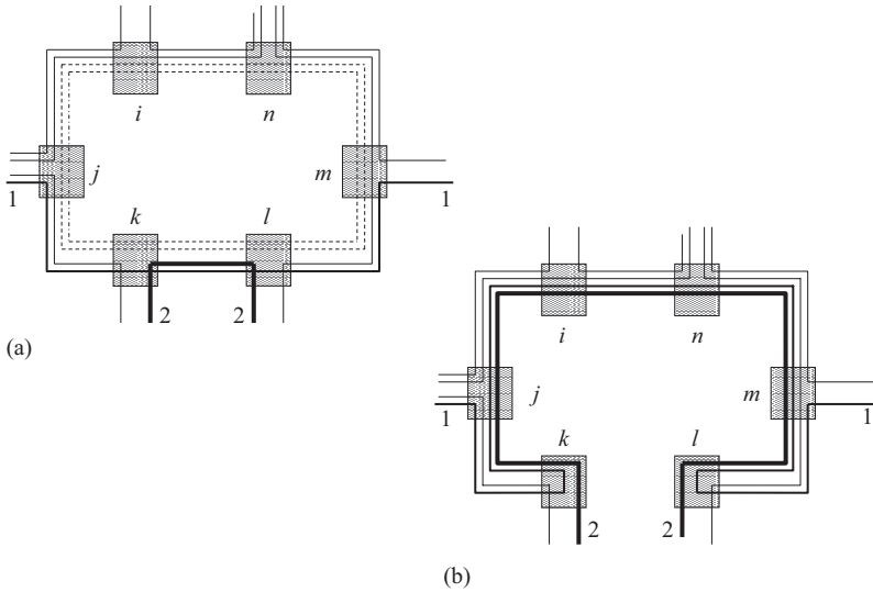
Figure 5.15 Transmission-path resilience: SPRINGS. (a) Ring with vacant standby paths. (b) Break between k – l ; Circuits 1 and 2 routed over standby paths around RING
