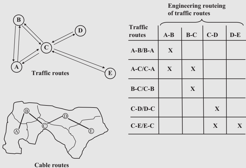
Figure 6.27 Planning example; Stage 6; Traffic route to engineering route matrix [Ward]
