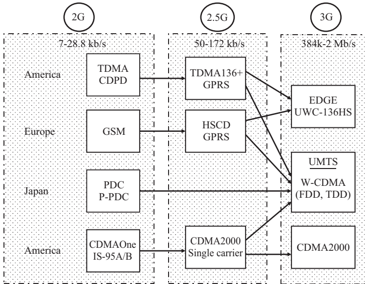
Figure 9.16 Mobile standards evolution from 2G to 3G
