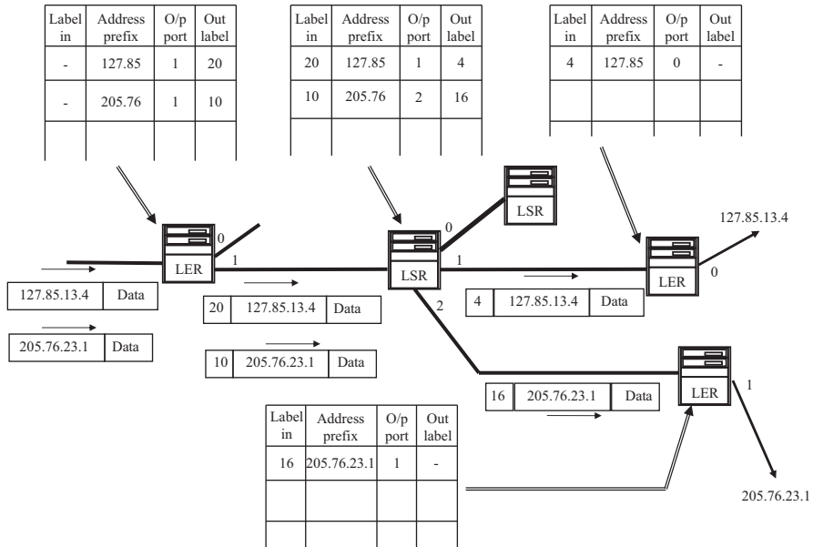
Figure 8.21 Example of multiprotocol label switching forwarding of packets
