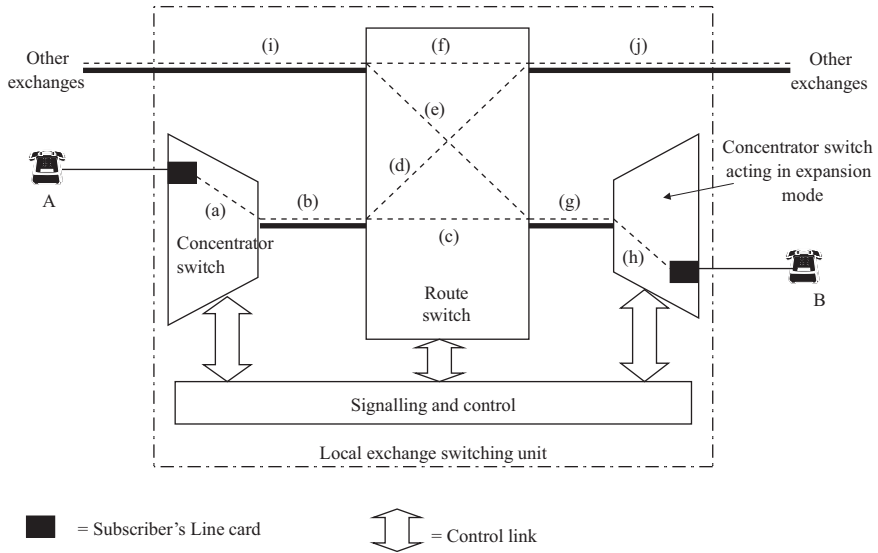
Figure 6.1 Simplified generalised local exchange
