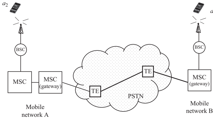
Figure 2.5 Mobile-to-mobile call via PSTN
