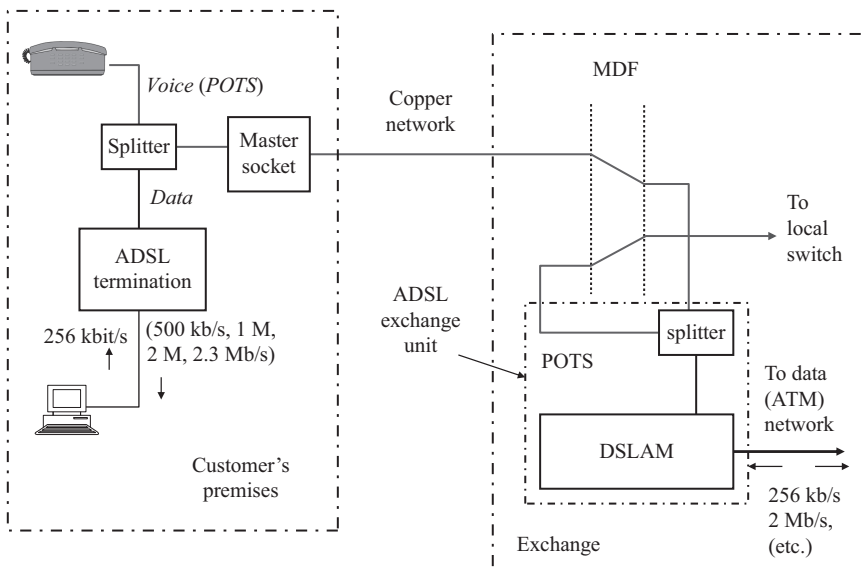
Figure 5.4 Basic ADSL architecture
