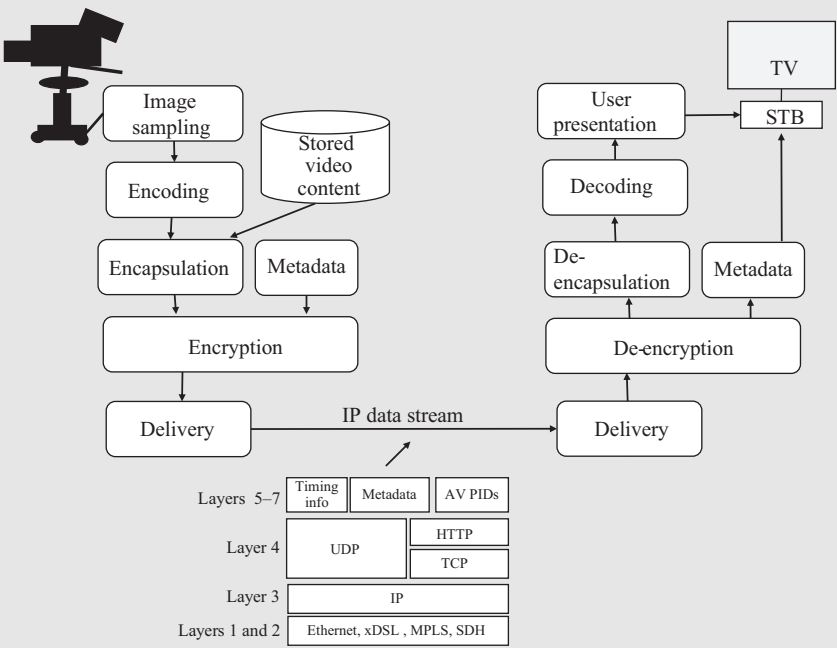
Figure 8.29 The process of carrying TV programmes over an IP network
