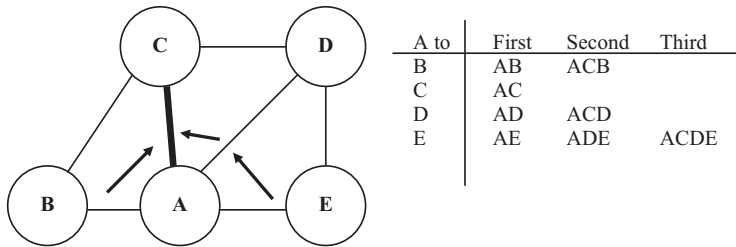
Figure 6.20 Automatic alternative routing
