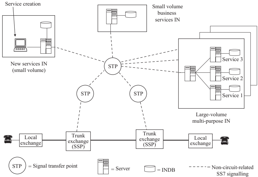
Figure 7.13 A typical set of INs
