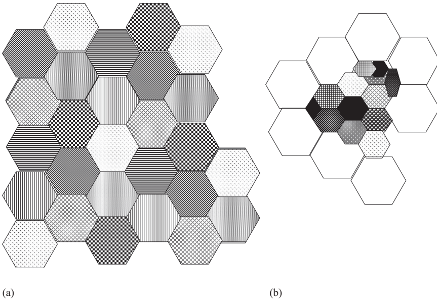
Figure 9.4 Cellular structure of a mobile radio network. (a) Full frequency re-use in a 7-cell structure and (b) micro- and pico-cells
