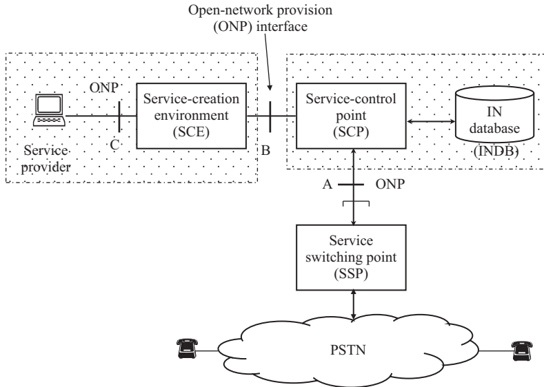
Figure 7.12 The intelligent network concept
