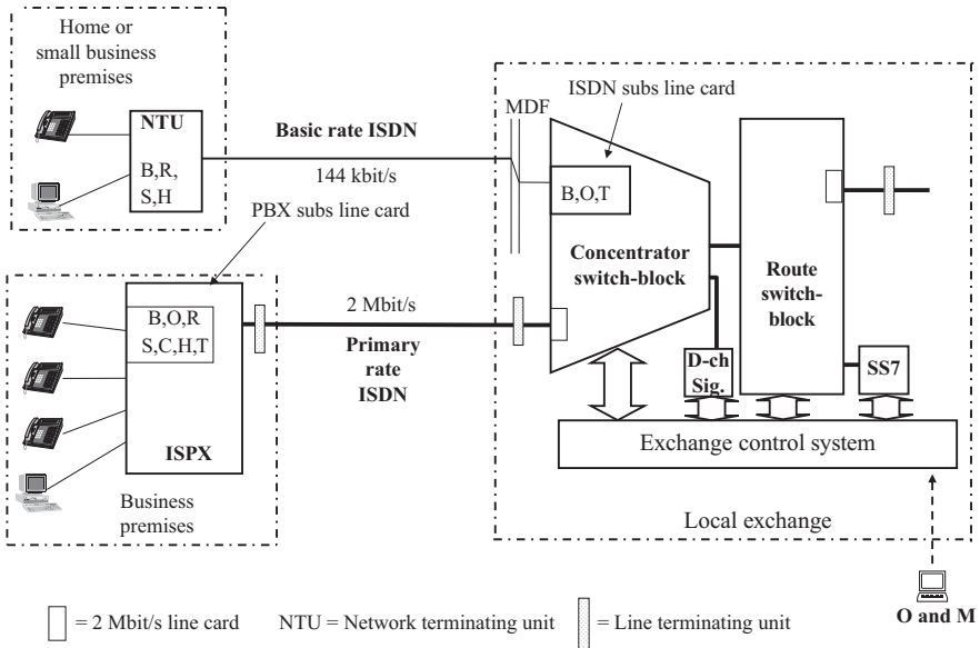
Figure 6.12 ISDN lines on a digital local exchange
