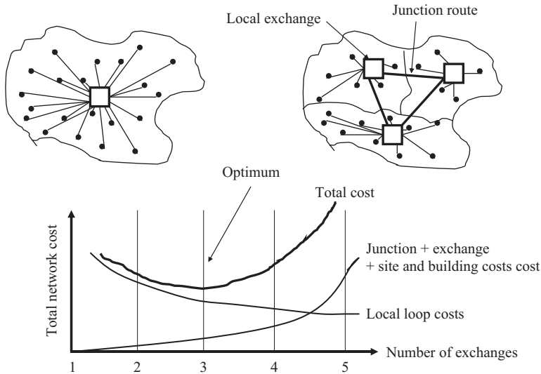
Figure 1.8 Network optimisation [Ward]
