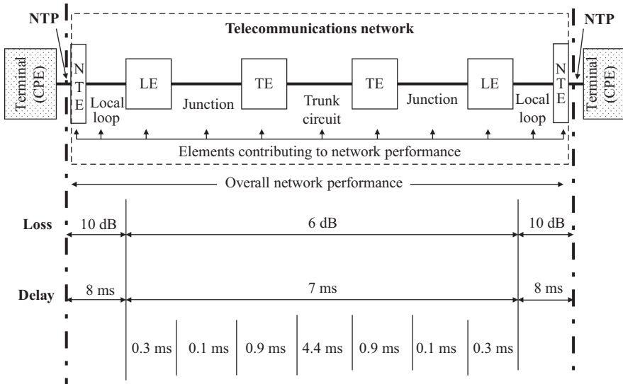
Figure 11.10 Apportionment of performance parameters
