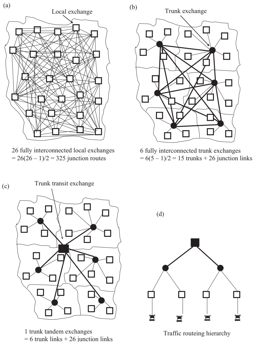
Figure 1.9 (a) Network structure 1. (b) Network structure 2. (c) Network structure 3. (d) Network structure 4 [Ward]
