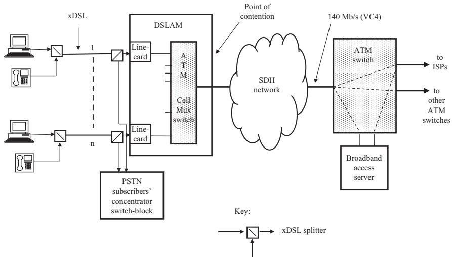
Figure 8.19 IP over ATM using xDSL access
