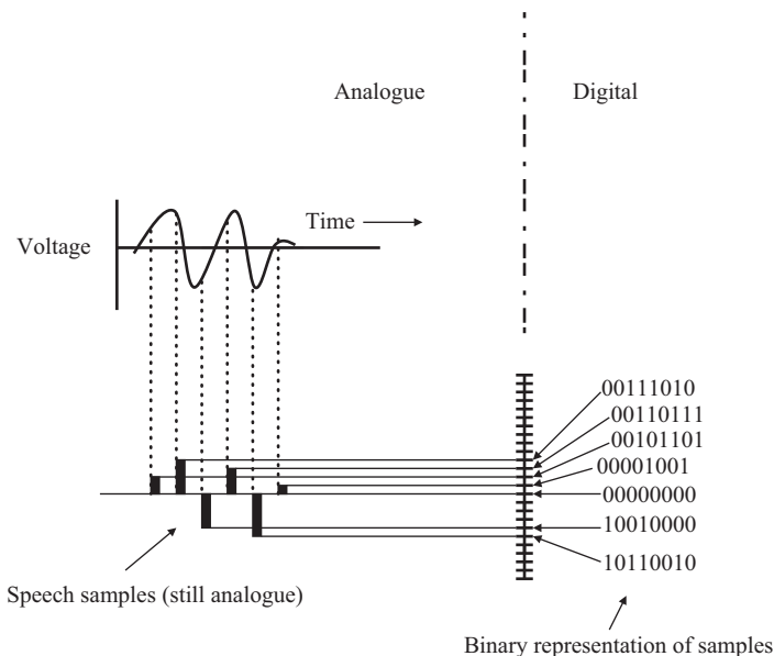
Figure 3.16 Analogue-to-digital conversion
