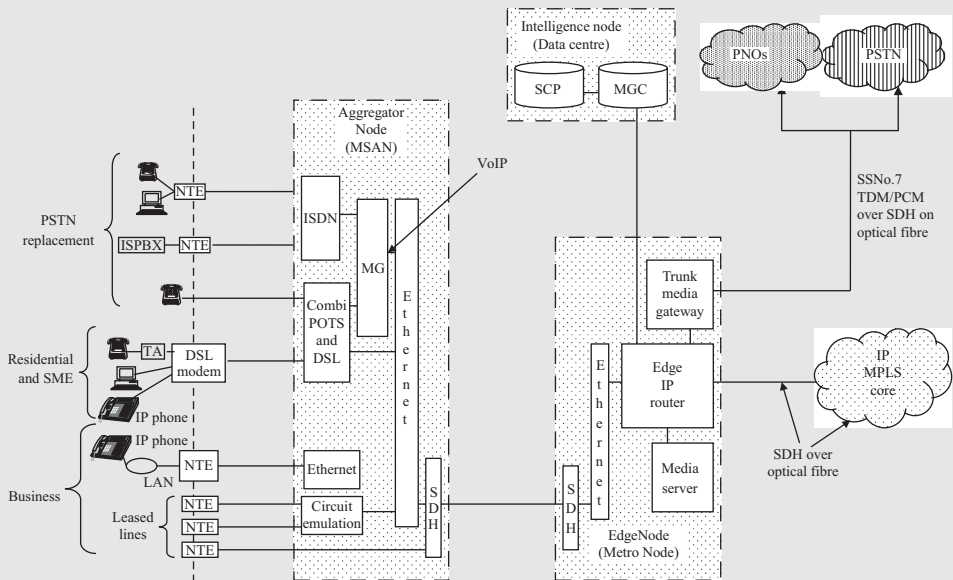
Figure 11.17 Example of a fixed network NGN physical architecture
