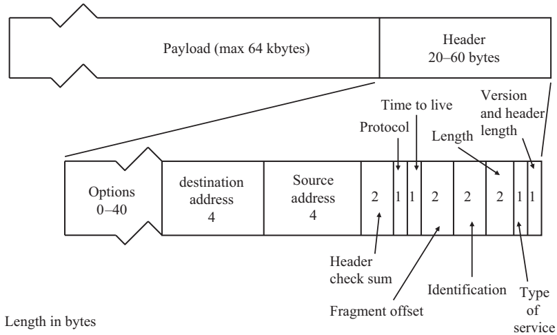
Figure 8.9 IPv4 packet format
