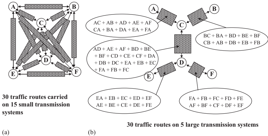
Figure 5.7 Economies of transmission aggregation [Ward]. (a) No aggregation. (b) With aggregation
