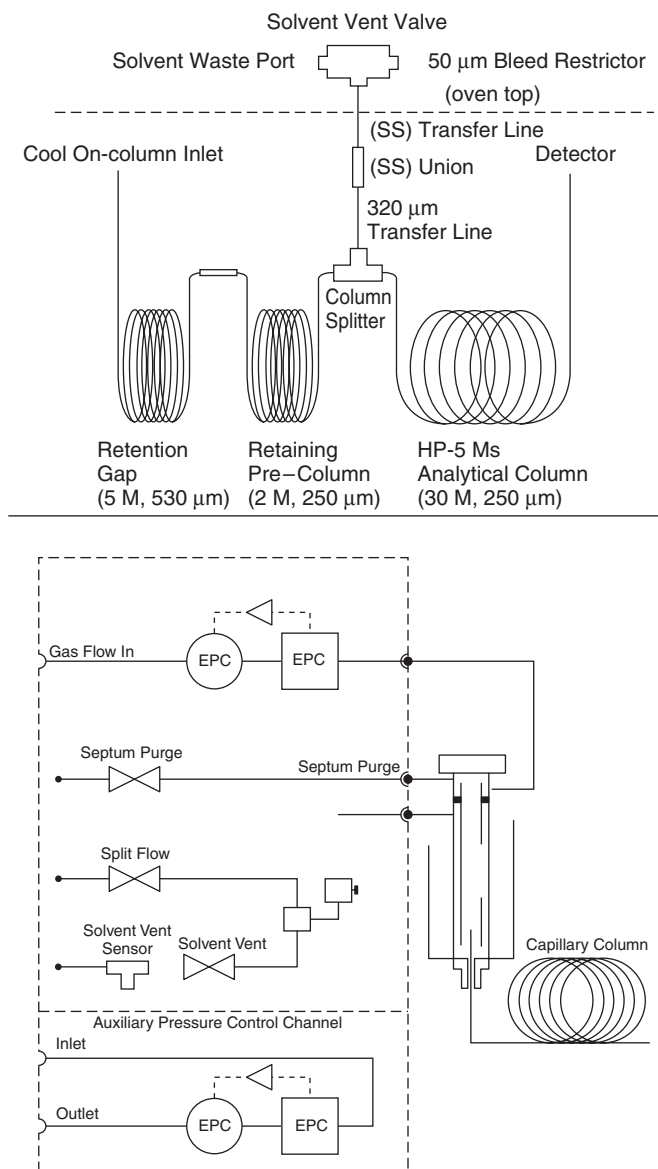
Figure 4.13. Schematic diagrams of large-volume injection systems. Top: on-column configuration with solvent vapor exit. (Drawing courtesy of Agilent Technologies.) Bottom: programmed temperature vaporization configuration. (Drawing courtesy of ATAS, International.)
