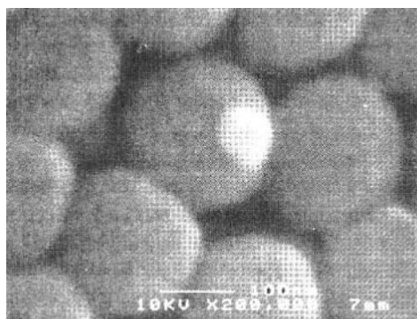
Figure 10.12. Atomic force microscope (a) and field-emission scanning electron microscope (b) images of an ordered array of 200-nm silver-coated silica spheres. (With permission from Ref. 37.)
