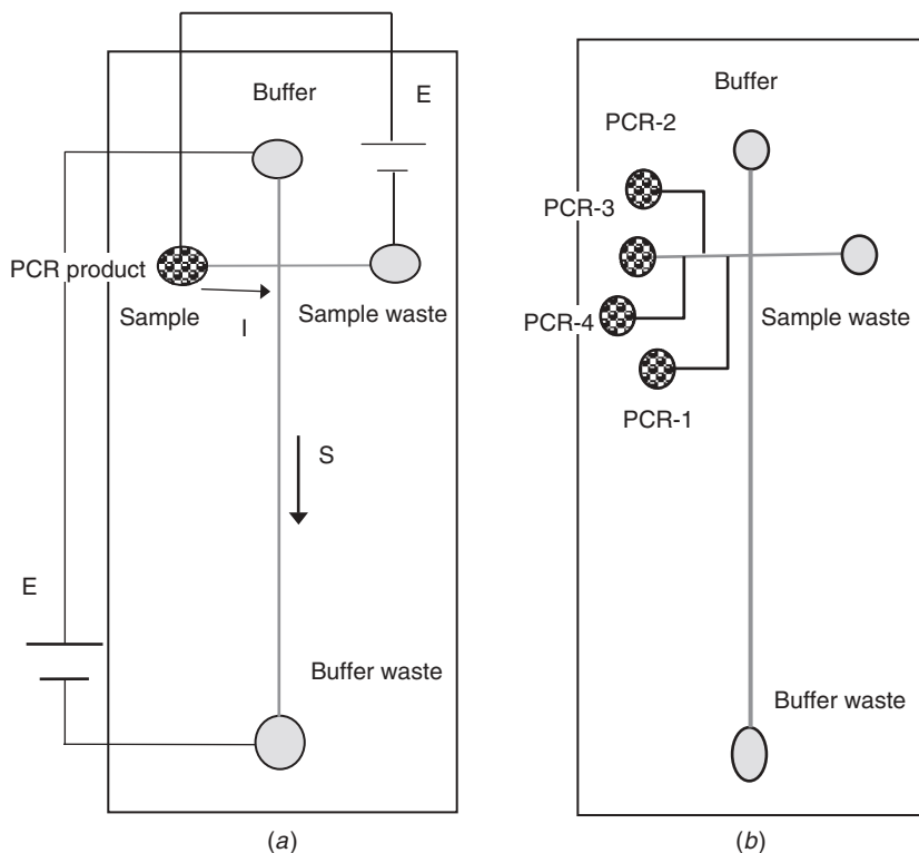
Figure 8.22. Capillary electrophoresis on a chip. (a) Schematic of the microchip used for PCR amplification and electrophoresis. The direction of arrows indicate injection (I) and separation (S). (b) Electrophoretic microchip with multiple PCR chambers.
