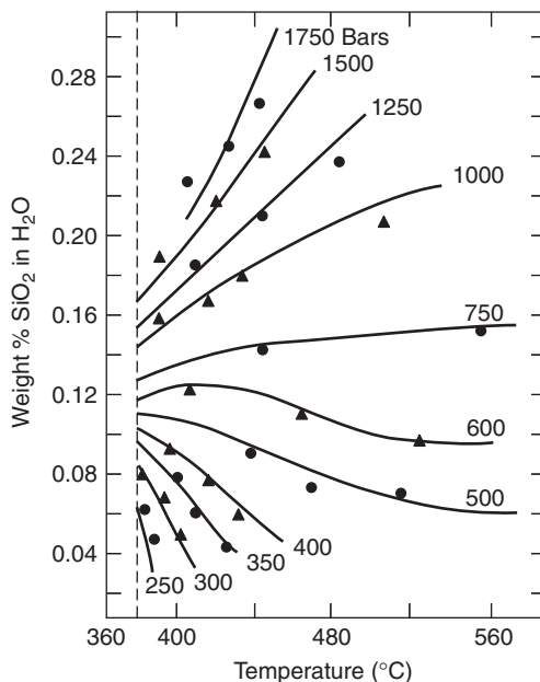
Figure 3.5. Solubility of \text{SiO}_2 in supercritical \text{H}_2\text{O} . (Reproduced from Ref. 22, with permission from Preston Publications.)
