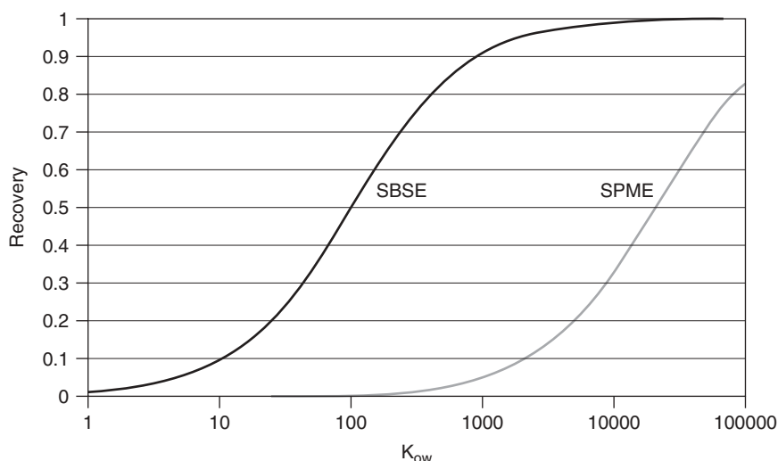
Figure 2.52. Theoretical recovery of analytes in SBSE and SPME from a 10-mL water sample as a function of their octanol–water partitioning constant. Volume of PDMS on SPME fiber: 0.5 \mu L; volume of PDMS on SBSE stir bar: 100 \mu L. (Reprinted with permission from Ref. 141. Copyright © 1999 John Wiley & Sons, Inc.)
