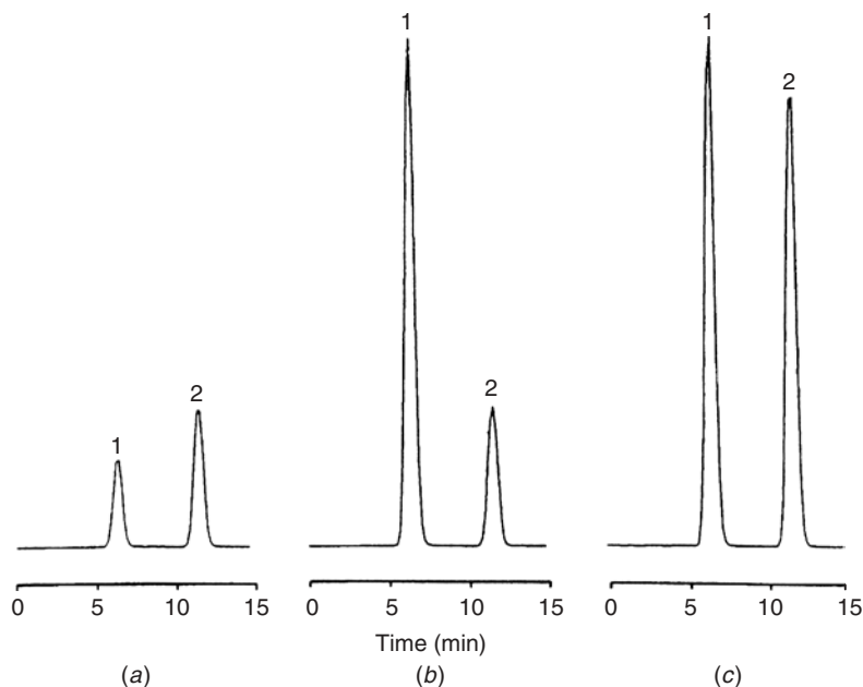
Figure 4.5. Analysis of three samples of an aqueous solution of cyclohexane (0.002 vol %) and 1,4-dioxane (0.1 vol %) in a 22.3-mL vial: (a) 1.0 mL of solution ( \beta = 21.3 ); (b) 5.0 mL of solution ( \beta = 3.46 ); (c) 5.0 mL of solution ( \beta = 3.46 ) to which 2 g of NaCl was added. Headspace conditions: equilibration at 60°C, with shaker. Peaks: 1, cyclohexane; 2, 1,4-dioxane. [Reprinted with permission from Ref. 15 (p. 30). Copyright John Wiley & Sons.]
