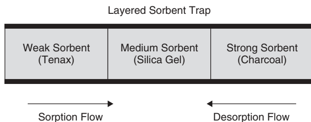
Figure 4.9. Schematic diagram of a multilayer sorbent trap.
