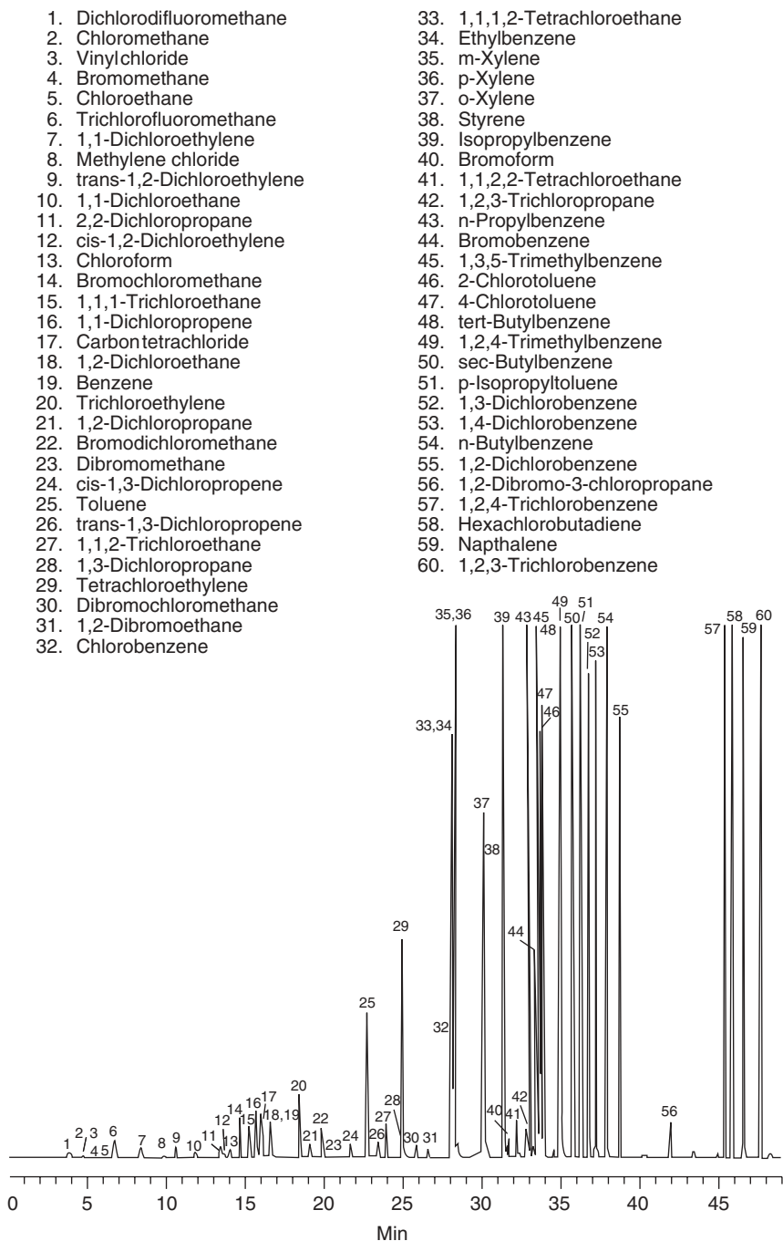
Figure 4.7. Chromatogram obtained using a purge-and-trap procedure as described in EPA method 524.2. (Reproduced from Ref. 26, with permission from Supelco Inc.)
