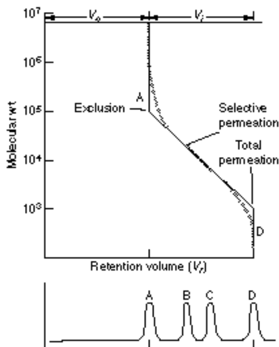
Figure 46.2 Log molecular weight versus retention volume plot for a typical SEC experiment with four narrow-fraction molecular weight standards. (From Introduction to Modern Liquid Chromatography , 2nd edition by L. Snyder and J. J. Kirkland, © 1979 by John Wiley & Sons, Inc. Reprinted by permission of John Wiley & Sons, Inc.)
