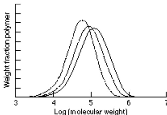
Figure 46.7 PEO apparent MWDs of polyurethane samples after various thermal processing steps. Virgin = solid curve, compounded = dashed curve, injection-molded = dot-dashed curve.
