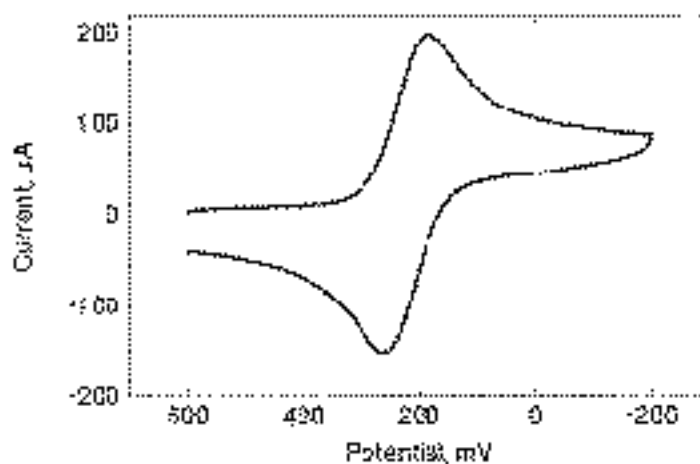
Figure 37.5 Cyclic voltammograms of 5 mM \text{Fe}(\text{CN})_6^{3-} in 1 M KCl with v = 500 \text{ mV/s} .
