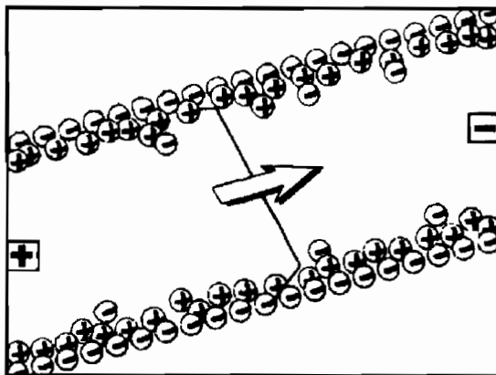
Figure 10.3 Representation of electroosmotic flow. The negatively charged spheres represent \text{SiO}^- groups on the surface of the capillary wall. The arrow indicates the direction of the flow and the flat line under the arrow indicates that the flow profile is relatively flat. (Reprinted courtesy of Hewlett-Packard Company.)
