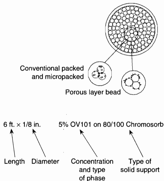
Figure 8.5 Packed column. (Courtesy of Hewlett-Packard Company.)
