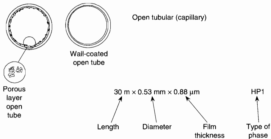
Figure 8.4 Capillary columns. (Courtesy of Hewlett-Packard Company.)
