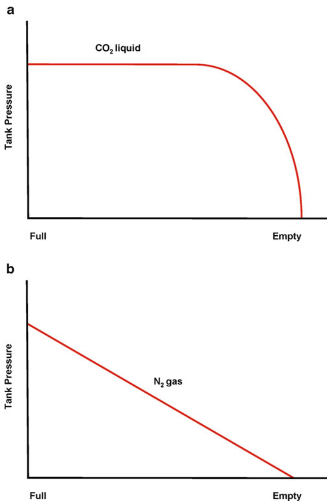
Fig. 9.3 (a) Because of the liquid state of the CO 2 supply and a constant pressure in the air space in the container above the liquid, one will not see a notable drop in manifold pressure until shortly before the cylinder runs empty. Liquid N 2 dewars will behave in the same manner. The manifold pressure is not an accurate reflection of the amount of gas left in the container. (b) In contrast, the pressure of compressed N 2 supplied in H-size metal cylinders is directly related to the amount of N 2 gas left in the cylinder, and the pressure in the tank is a reliable indication of the N 2 reserve
