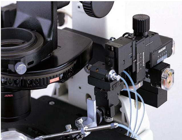
Fig. 35.3 Example of drive unit of hydraulic manipulator (connected to control unit by tubing) mounted on electrical coarse control manipulator and universal joint for mounting of the tool holder (courtesy of Nikon, Melville, NY, USA)
