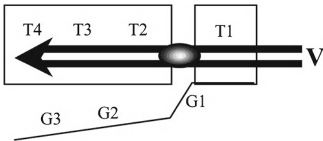
Fig. 60.1 Along the blocks, different temperatures (T1, T2, T3, T4) can be set, thereby imposing a temperature gradient (G1, G2, G3)
