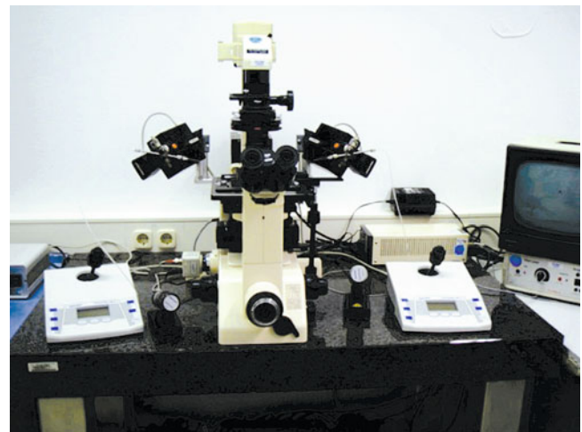
Fig. 37.1 The Eppendorf micromanipulator is composed of three main components: motor module unit, control board, and main power supply
