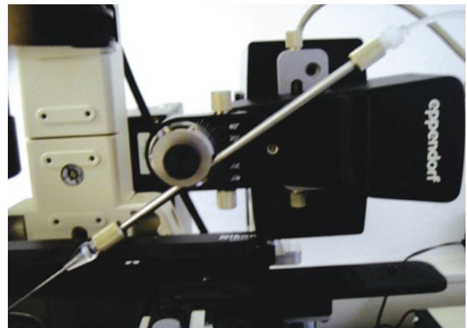
Fig. 37.2 Mounted motor module with attached capillary holder
