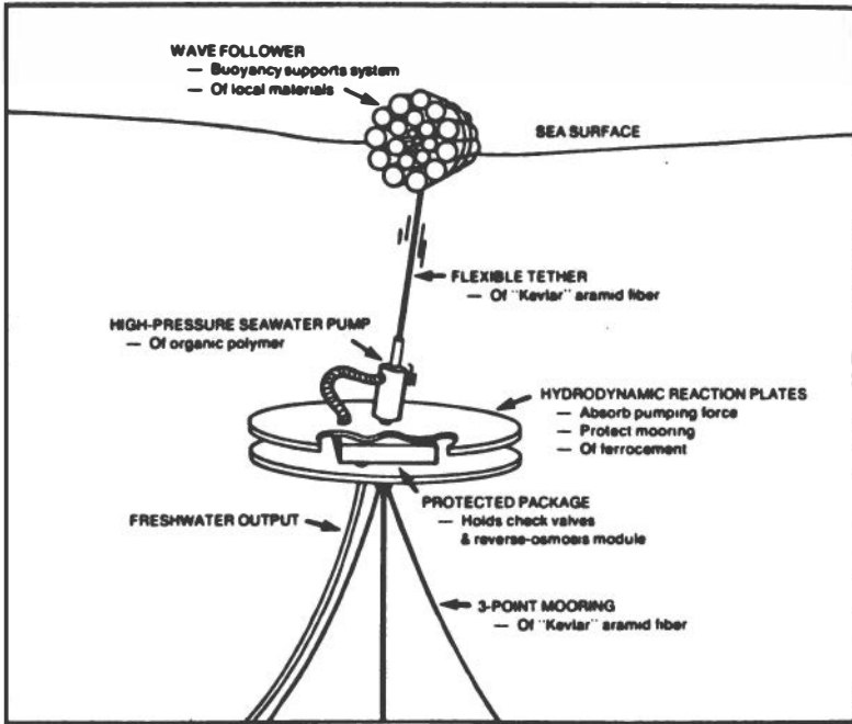
FIGURE 7-2 Pump used in wave energy desalinization device designed by scientists at the University of Delaware. (University of Delaware)
