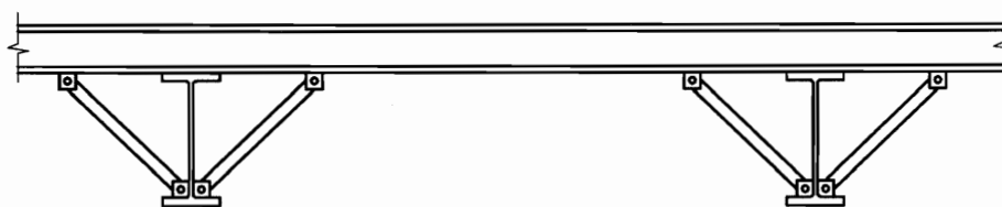
Figure 6.5: Typical stiff torsional restraint
