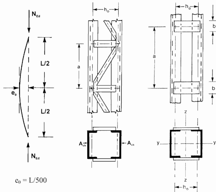
Figure 6.7: Uniform built-up columns with lacings and \overline{AC_2} battens \overline{AC_2}
