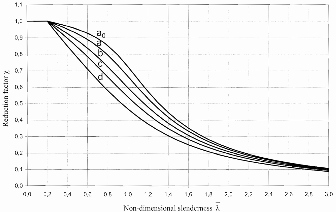
Figure 6.4: Buckling curves
