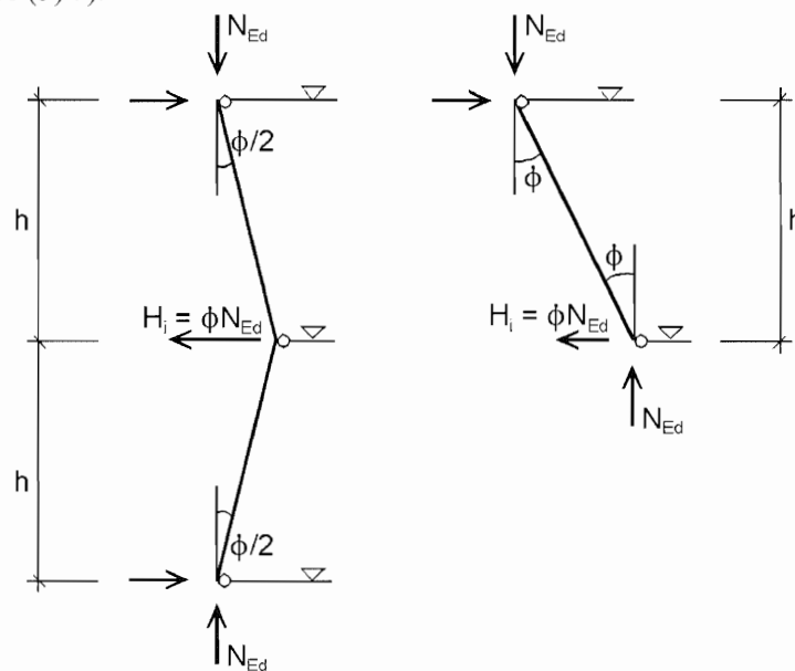
Figure 5.3: Configuration of sway imperfections \phi for horizontal forces on floor diaphragms
