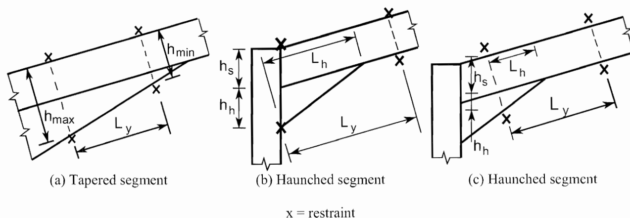
Figure BB.6: Dimensions defining taper factor
