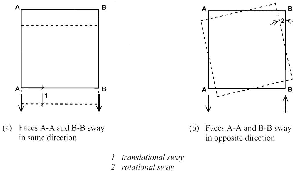
Figure 5.5: Translational and torsional effects (plan view)
