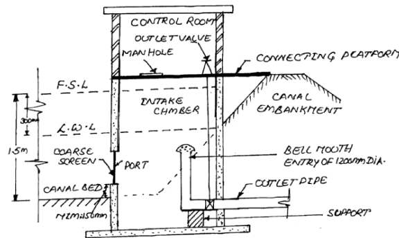
Fig. 3.14 Canal Intake
