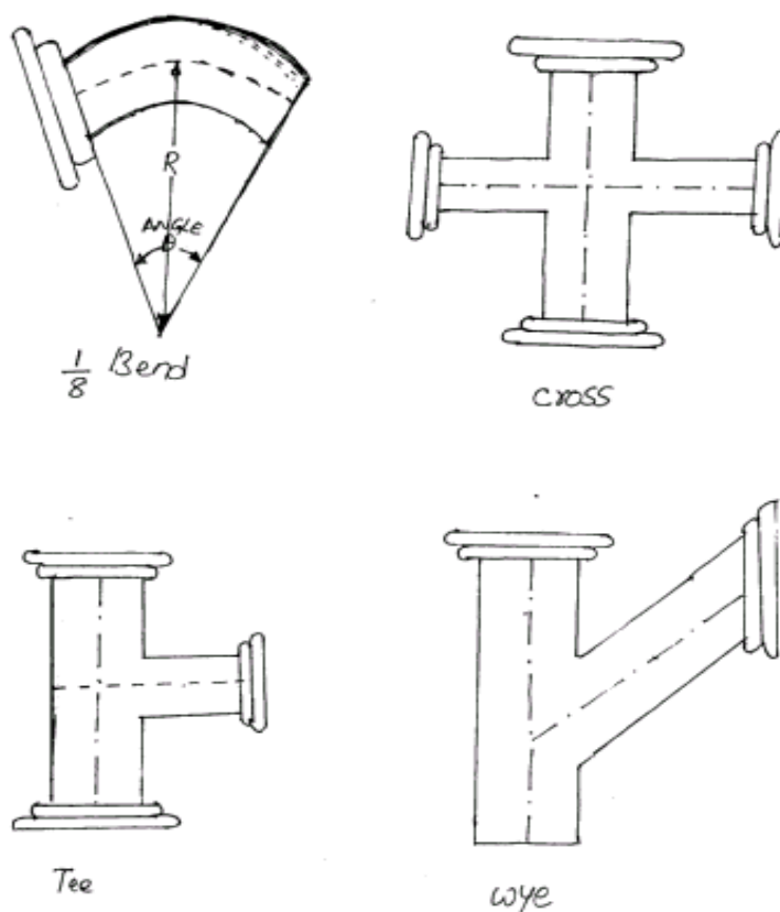
Fig 8.4 Pipe Fittings
