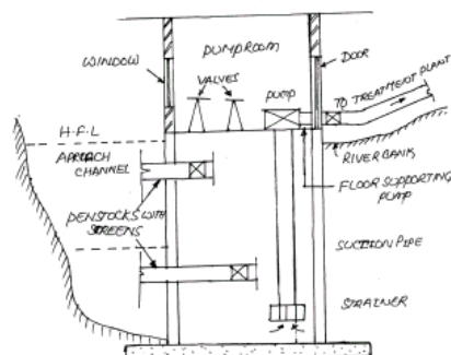
Fig. 3.12 River Intake
