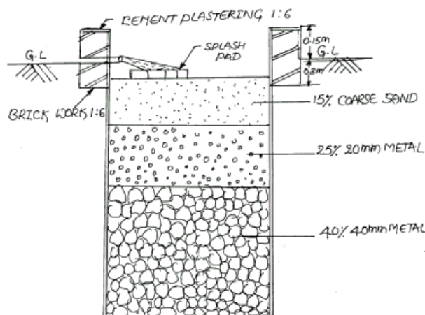
Fig 9.2 Percolation Pit
