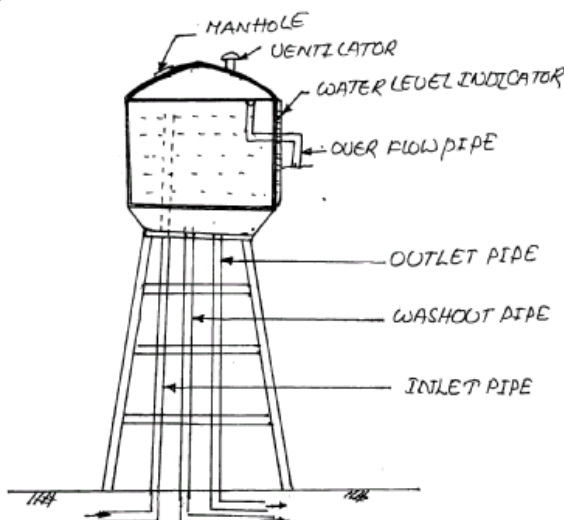
Fig 8.5. Overhead Tank
