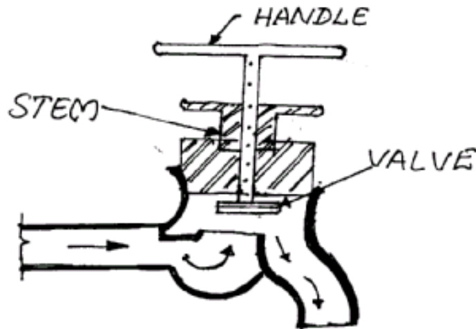
Fig 8.3 Bib Cock
