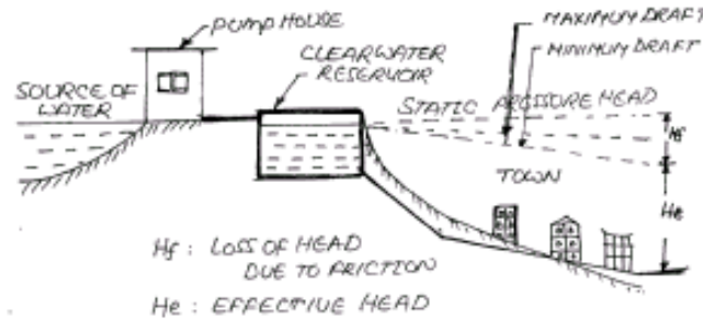
FIG 6.5 Gravity System
