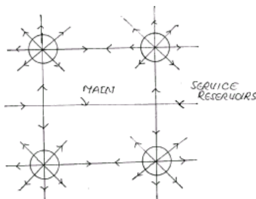
Fig. 6.4 Radial System
