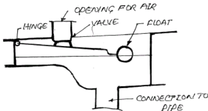
Fig 7.3. Air Valve
