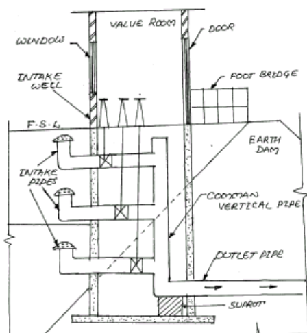
Fig. 3.13 Reservoir Intake
