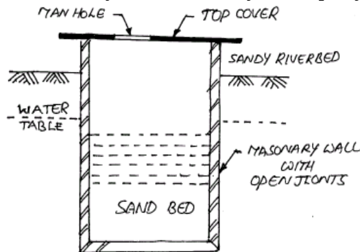
Fig 3.3 Infiltration Well
