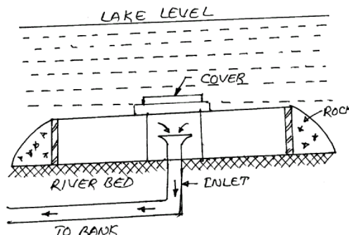
Fig 3.11 Lake Intake
