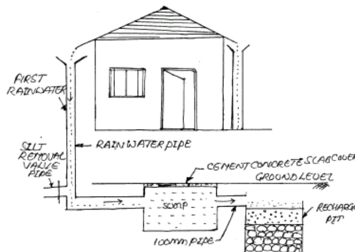
Fig 9.1 Storage Sump and Recharge Pit
