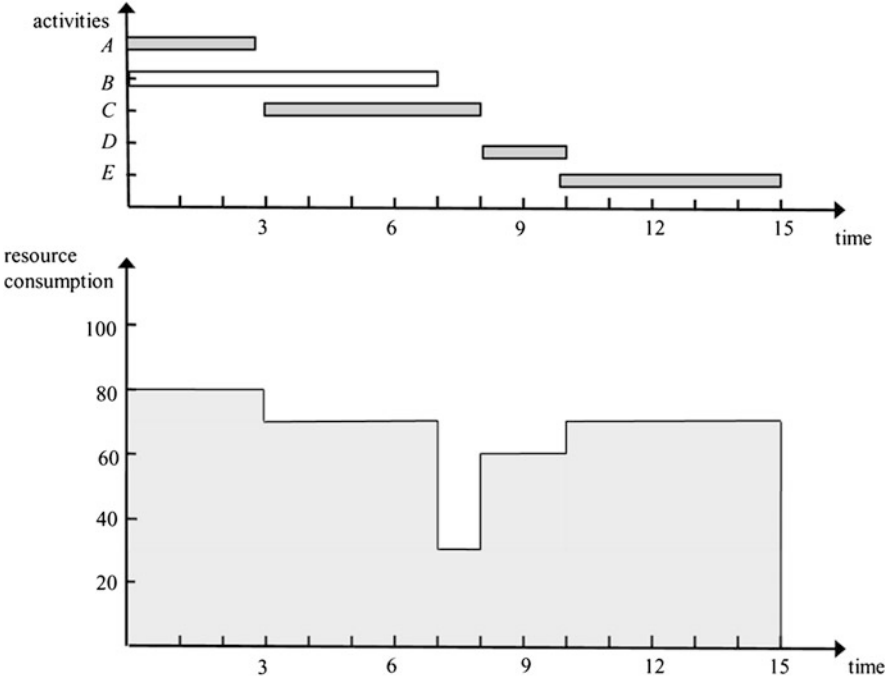
Fig. 7.18 Gantt chart and resource requirement graph for Problem 2
