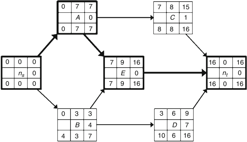
Fig. 7.20 Project activity network for Problem 4
