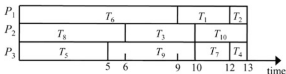
Fig. 8.15 Optimal schedule for Problem 1(e)
