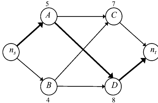
Fig. 7.5 Critical path with normal activity durations
