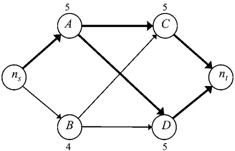
Fig. 7.8 Critical path with activities C and D accelerated
