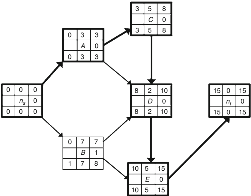
Fig. 7.17 Project network for Problem 2
