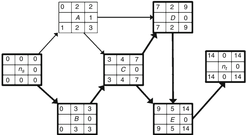
Fig. 7.19 Project activity network for Problem 3
