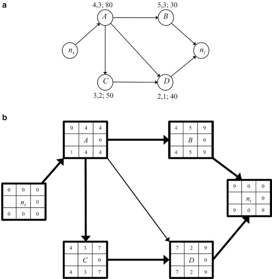
Fig. 7.16 (a) Project network for Problem 1 with original data; (b) project network with earliest and latest starting and finishing times and total floats
