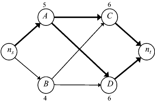
Fig. 7.7 Critical path with activities C and D accelerated
