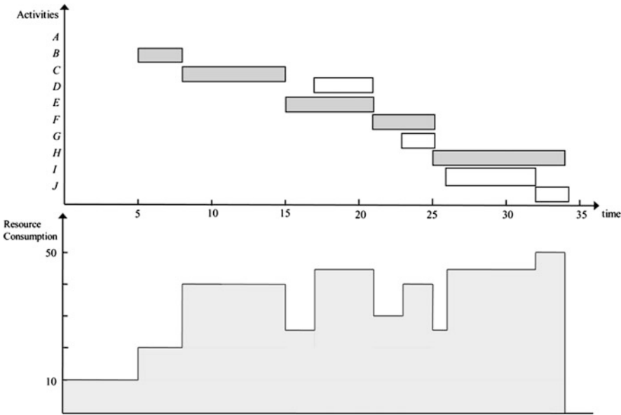
Fig. 7.12 Gantt chart and resource requirement graph for alternative schedule
