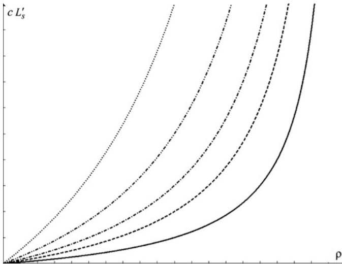
Fig. 13.2 Customers in the system as a function of the utilization rate, for various numbers of servers
