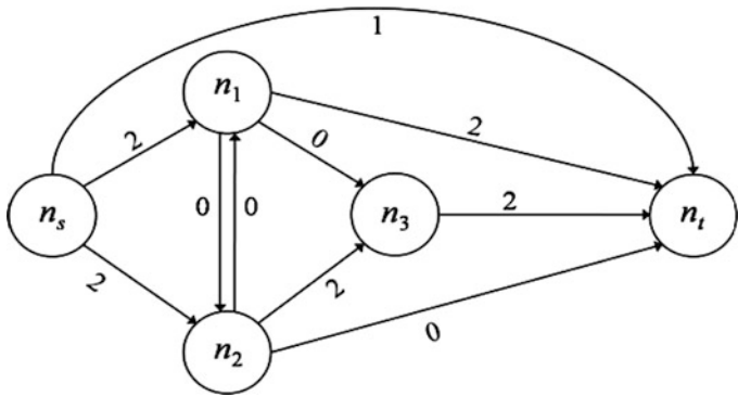
Fig. 5.34 Optimal flow pattern for Problem 2
