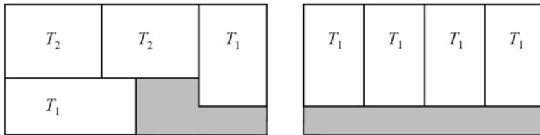
Fig. 4.5 Cutting patterns for plywood boards
