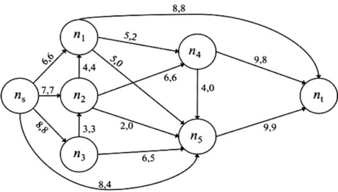
Fig. 5.32 Third and optimal flow pattern for Problem 1
